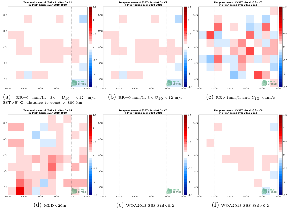
Figure 12: Temporal mean gridded over spatial boxes of size 1^\circ \times 1^\circ of \Delta SSS (SMOS SSS L3 v4 - 9 Days (CATDS-CECOS-LOCEAN) - Argo) for 6 different subdatasets corresponding to:RR=0 mm/h, 3 < U_{10} < 12 m/s, SST >5^\circ\text{C} , distance to coast > 800 km (a), RR=0 mm/h, 3 < U_{10} < 12 m/s (b), RR >1 mm/h and U_{10} < 4 m/s (c),MLD <20 m (d),WOA2013 SSS Std <0.2 (e),WOA2013 SSS Std >0.2 (f).
