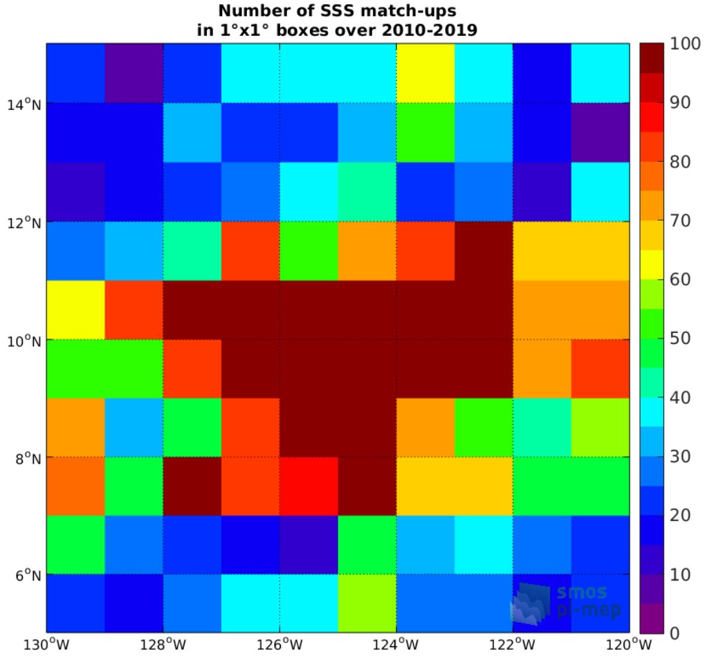
Figure 4: Number of SSS match-ups between Argo SSS and the SMOS SSS L3 v4 - 9 Days (CATDS-CECOS-LOCEAN) SSS product for the SPURS 2 Pi-MEP region over 1°x1° boxes and for the full satellite product period.
