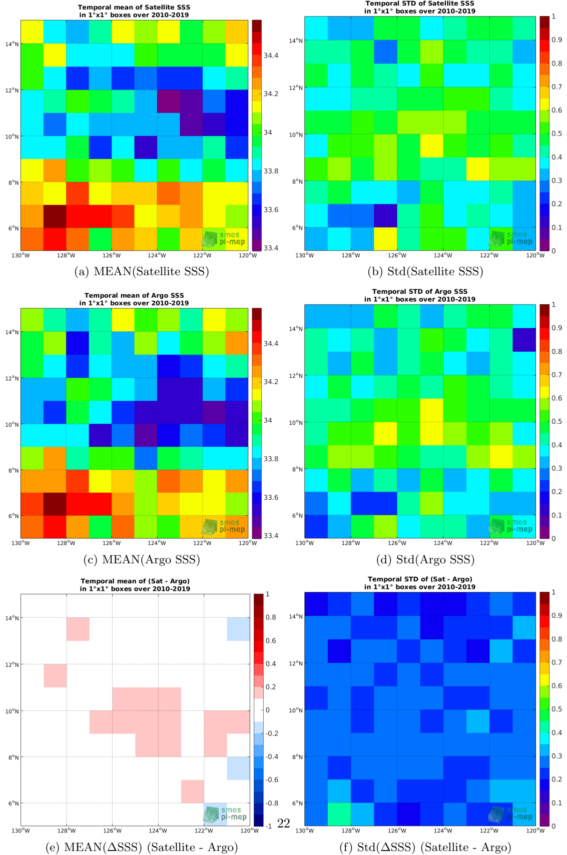
Figure 6: Temporal mean (left) and Std (right) of SSS from SMOS SSS L3 v4 - 9 Days (CATDS-CECOS-LOCEAN) (top), Argo (middle), and of \Delta SSS (Satellite - Argo). Only match-up pairs are used to generate these maps.
