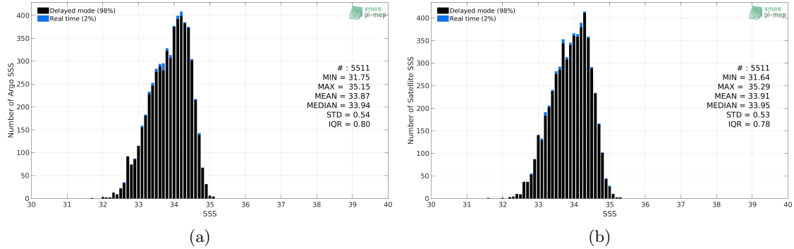
Figure 2: Histograms of SSS from Argo (a) and SMOS SSS L3 v4 - 9 Days (CATDS-CECOS-LOCEAN) (b) considering all match-up pairs per bins of 0.1 over the SPURS 2 Pi-MEP region and for the full satellite product period.
