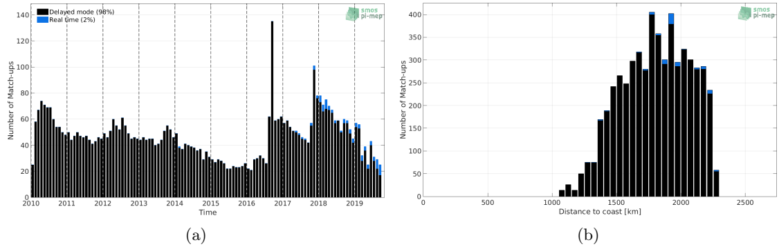
Figure 1: Number of match-ups between Argo and SMOS SSS L3 v4 - 9 Days (CATDS-CECOS-LOCEAN) SSS as a function of time (a) and as function of the distance to coast (b) over the SPURS 2 Pi-MEP region and for the full satellite product period.
