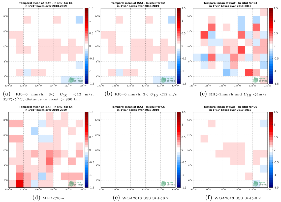
Figure 12: Temporal mean gridded over spatial boxes of size 1^\circ \times 1^\circ of \Delta SSS (SMOS-L3-CATDS-CECOS-LOCEAN-V4-9DAYS-25KM - Argo) for 6 different subdatasets corresponding to:RR=0 mm/h, 3 < U_{10} < 12 m/s, SST >5^\circ C, distance to coast > 800 km (a), RR=0 mm/h, 3 < U_{10} < 12 m/s (b), RR >1 mm/h and U_{10} < 4 m/s (c),MLD <20 m (d),WOA2013 SSS Std <0.2 (e),WOA2013 SSS Std >0.2 (f).
