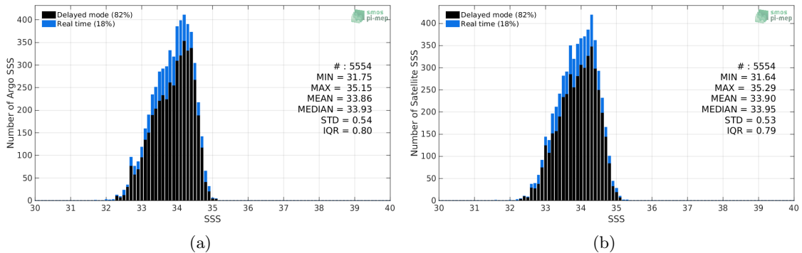
Figure 2: Histograms of SSS from Argo (a) and SMOS-L3-CATDS-CECOS-LOCEAN-V4-9DAYS-25KM (b) considering all match-up pairs per bins of 0.1 over the SPURS 2 Pi-MEP region and for the full satellite product period.
