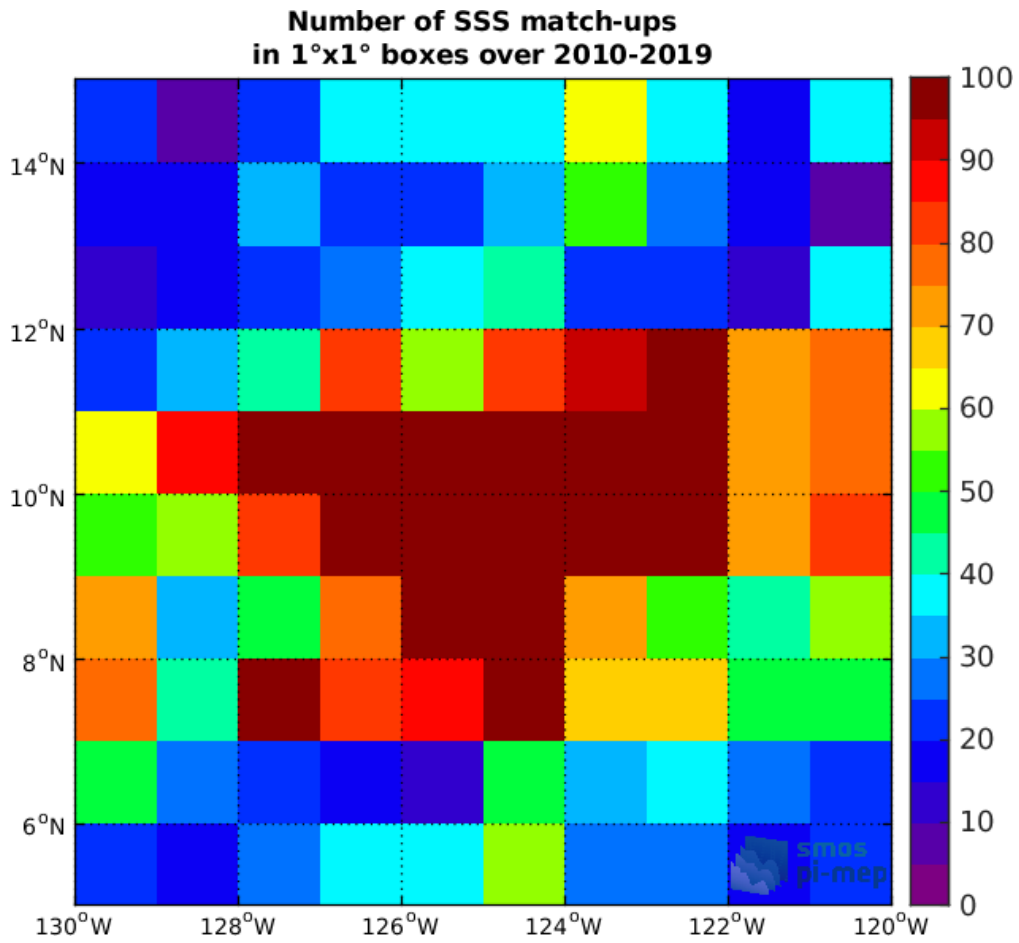
Figure 4: Number of SSS match-ups between Argo SSS and the SMOS-L3-CATDS-CECOS-LOCEAN-V4-9DAYS-25KM SSS product for the SPURS 2 Pi-MEP region over 1°x1° boxes and for the full satellite product period.
