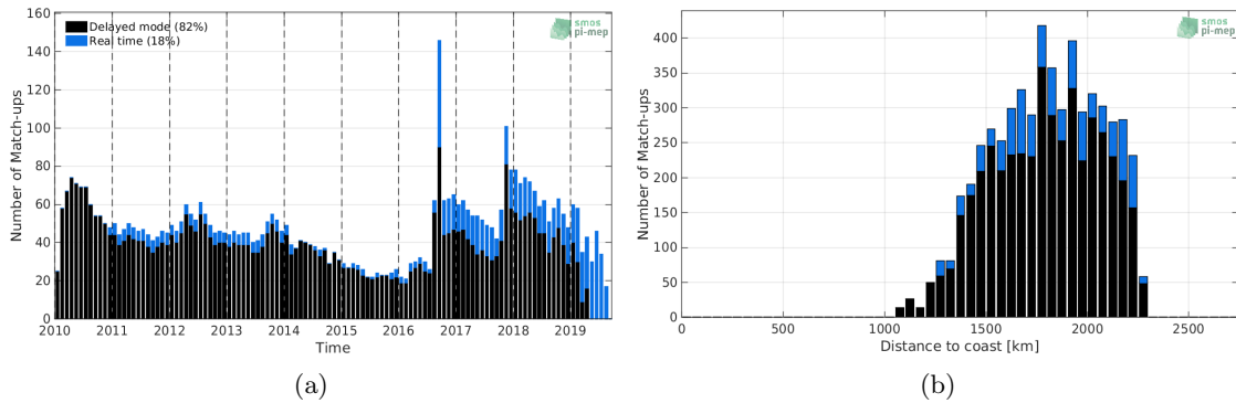
Figure 1: Number of match-ups between Argo and SMOS-L3-CATDS-CECOS-LOCEAN-V4-9DAYS-25KM SSS as a function of time (a) and as function of the distance to coast (b) over the SPURS 2 Pi-MEP region and for the full satellite product period.
