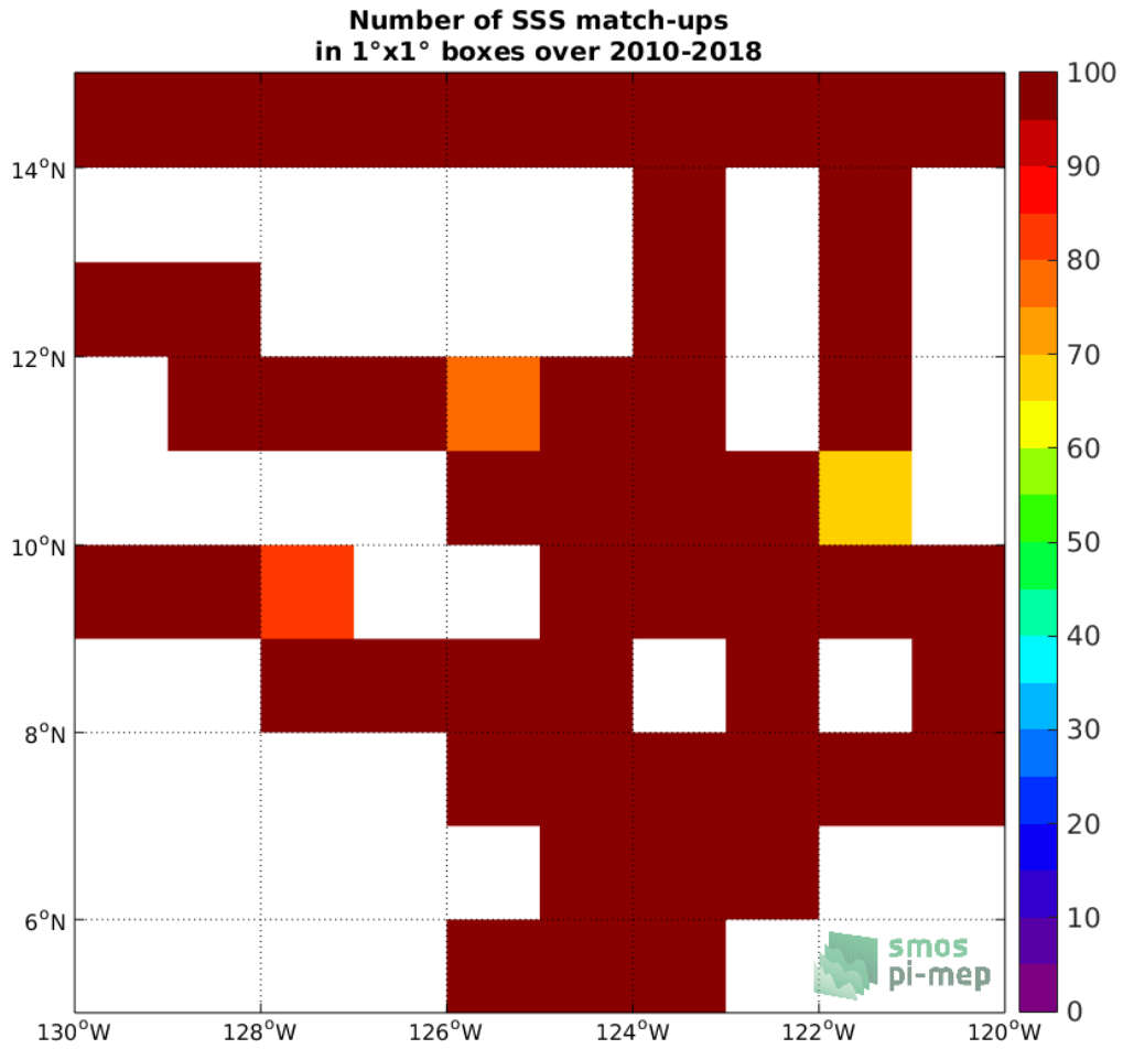
Figure 4: Number of SSS match-ups between TSG-SAMOS SSS and the SMOS-L3-CATDS-CECOS-LOCEAN-V4-18DAYS-25KM SSS product for the SPURS 2 Pi-MEP region over 1°x1° boxes and for the full satellite product period.
