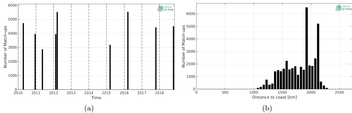
Figure 1: Number of match-ups between TSG-SAMOS and SMOS-L3-CATDS-CECOS-LOCEAN-V4-18DAYS-25KM SSS as a function of time (a) and as function of the distance to coast (b) over the SPURS 2 Pi-MEP region and for the full satellite product period.
