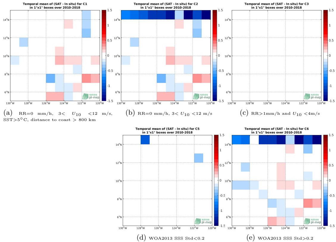
Figure 12: Temporal mean gridded over spatial boxes of size 1^\circ \times 1^\circ of \Delta SSS (SMOS-L3-CATDS-CECOS-LOCEAN-V4-18DAYS-25KM - TSG-SAMOS) for 5 different subdatasets corresponding to:RR=0 mm/h, 3 < U_{10} < 12 m/s, SST > 5^\circ\text{C} , distance to coast > 800 km (a), RR=0 mm/h, 3 < U_{10} < 12 m/s (b), RR > 1 mm/h and U_{10} < 4 m/s (c), WOA2013 SSS Std < 0.2 (d), WOA2013 SSS Std > 0.2 (e).
