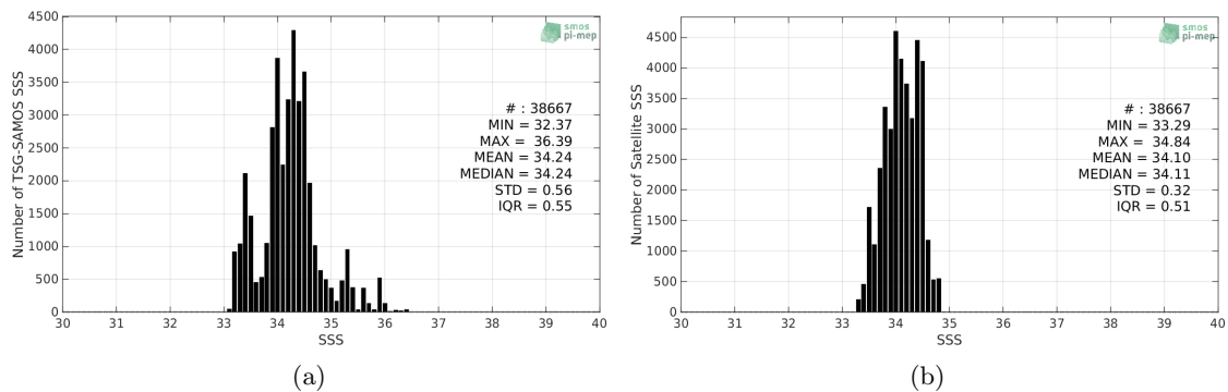
Figure 2: Histograms of SSS from TSG-SAMOS (a) and SMOS-L3-CATDS-CECOS-LOCEAN-V4-18DAYS-25KM (b) considering all match-up pairs per bins of 0.1 over the SPURS 2 Pi-MEP region and for the full satellite product period.
