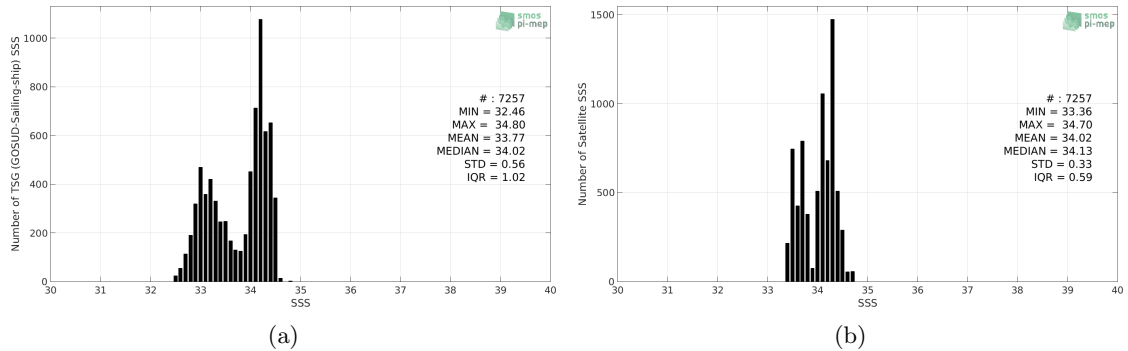
Figure 2: Histograms of SSS from TSG (GOSUD-Sailing-ship) (a) and SMOS SSS L3 v4 - 18 Days (CATDS-CECOS-LOCEAN) (b) considering all match-up pairs per bins of 0.1 over the SPURS 2 Pi-MEP region and for the full satellite product period.
