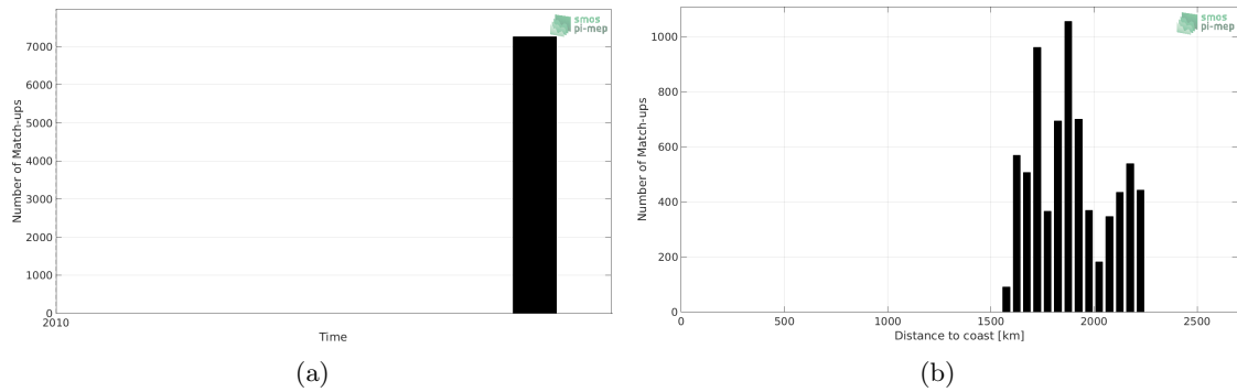
Figure 1: Number of match-ups between TSG (GOSUD-Sailing-ship) and SMOS SSS L3 v4 - 18 Days (CATDS-CECOS-LOCEAN) SSS as a function of time (a) and as function of the distance to coast (b) over the SPURS 2 Pi-MEP region and for the full satellite product period.
