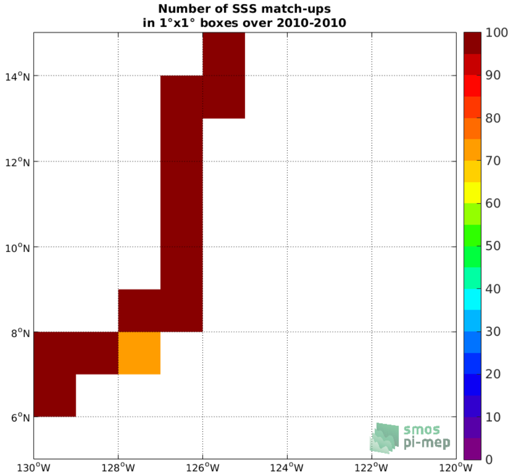
Figure 4: Number of SSS match-ups between TSG (GOSUD-Sailing-ship) SSS and the SMOS SSS L3 v4 - 18 Days (CATDS-CECOS-LOCEAN) SSS product for the SPURS 2 Pi-MEP region over 1°x1° boxes and for the full satellite product period.
