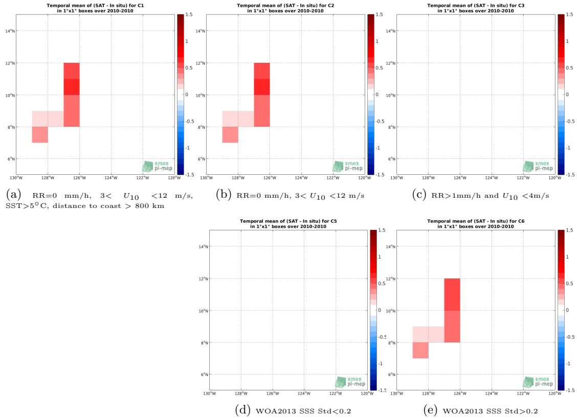
Figure 12: Temporal mean gridded over spatial boxes of size 1°x1° of \Delta SSS (SMOS SSS L3 v4 - 18 Days (CATDS-CECOS-LOCEAN) - TSG (GOSUD-Sailing-ship)) for 5 different subdatasets corresponding to:RR=0 mm/h, 3 < U_{10} < 12 m/s, SST>5°C, distance to coast > 800 km (a), RR=0 mm/h, 3 < U_{10} < 12 m/s (b), RR>1mm/h and U_{10} < 4 m/s (c), WOA2013 SSS Std<0.2 (d), WOA2013 SSS Std>0.2 (e).
