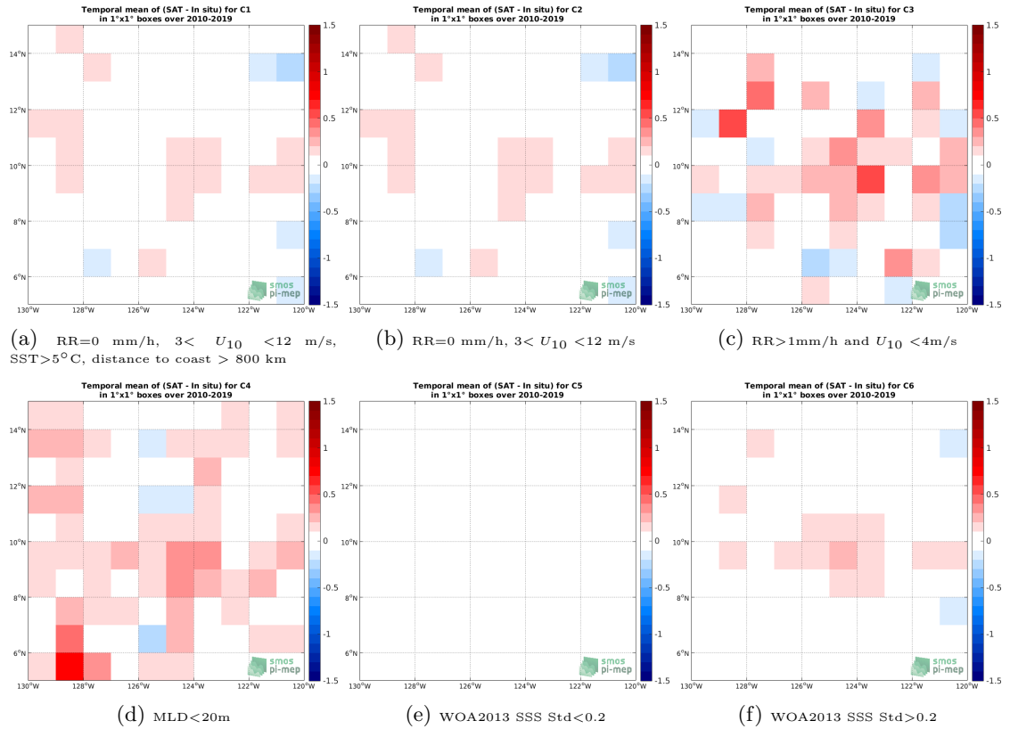
Figure 12: Temporal mean gridded over spatial boxes of size 1^\circ \times 1^\circ of \Delta SSS (SMOS SSS L3 v4 - 18 Days (CATDS-CECOS-LOCEAN) - Argo) for 6 different subdatasets corresponding to:RR=0 mm/h, 3 < U_{10} < 12 m/s, SST >5^\circ C, distance to coast > 800 km (a), RR=0 mm/h, 3 < U_{10} < 12 m/s (b), RR >1 mm/h and U_{10} < 4 m/s (c),MLD <20 m (d),WOA2013 SSS Std <0.2 (e),WOA2013 SSS Std >0.2 (f).
