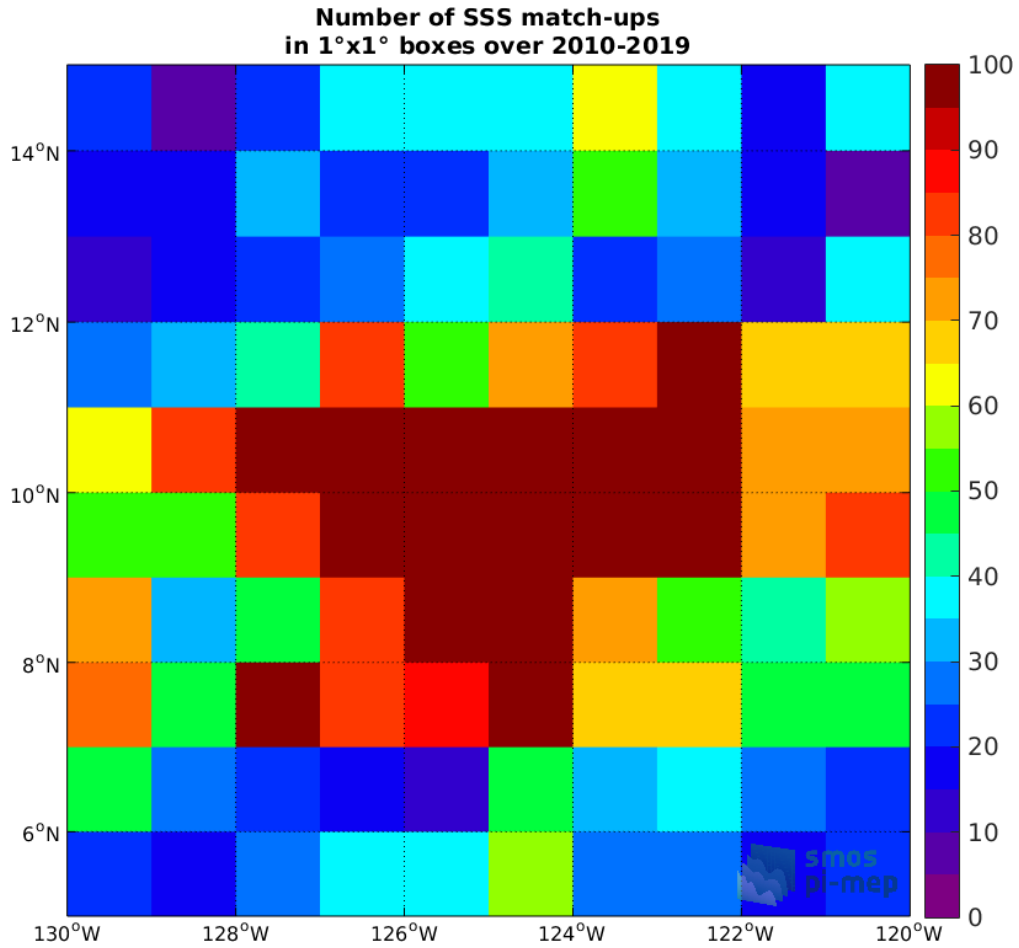
Figure 4: Number of SSS match-ups between Argo SSS and the SMOS SSS L3 v4 - 18 Days (CATDS-CECOS-LOCEAN) SSS product for the SPURS 2 Pi-MEP region over 1°x1° boxes and for the full satellite product period.
