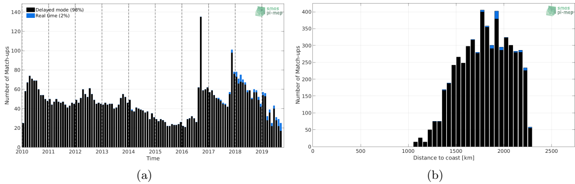
Figure 1: Number of match-ups between Argo and SMOS SSS L3 v4 - 18 Days (CATDS-CECOS-LOCEAN) SSS as a function of time (a) and as function of the distance to coast (b) over the SPURS 2 Pi-MEP region and for the full satellite product period.
