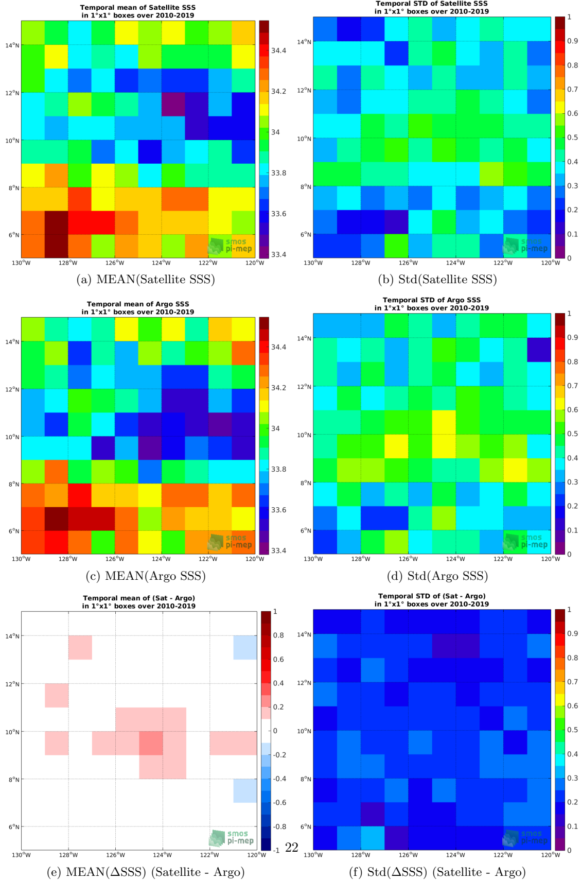
Figure 6: Temporal mean (left) and Std (right) of SSS from SMOS SSS L3 v4 - 18 Days (CATDS-CECOS-LOCEAN) (top), Argo (middle), and of \Delta SSS (Satellite - Argo). Only match-up pairs are used to generate these maps.
