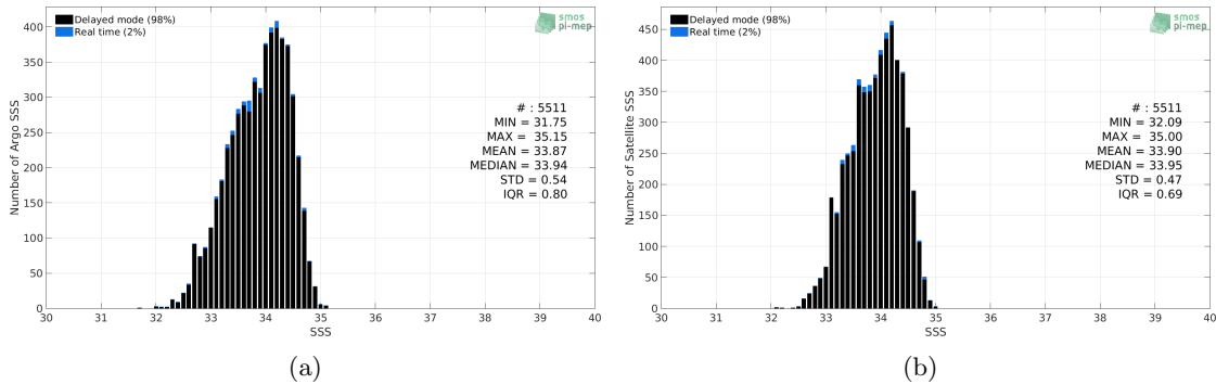
Figure 2: Histograms of SSS from Argo (a) and SMOS SSS L3 v4 - 18 Days (CATDS-CECOS-LOCEAN) (b) considering all match-up pairs per bins of 0.1 over the SPURS 2 Pi-MEP region and for the full satellite product period.
