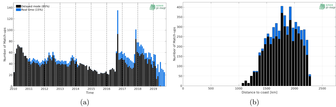
Figure 1: Number of match-ups between Argo and SMOS-L3-CATDS-CECOS-LOCEAN-V4-18DAYS-25KM SSS as a function of time (a) and as function of the distance to coast (b) over the SPURS 2 Pi-MEP region and for the full satellite product period.
