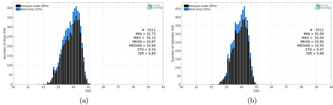
Figure 2: Histograms of SSS from Argo (a) and SMOS-L3-CATDS-CECOS-LOCEAN-V4-18DAYS-25KM (b) considering all match-up pairs per bins of 0.1 over the SPURS 2 Pi-MEP region and for the full satellite product period.
