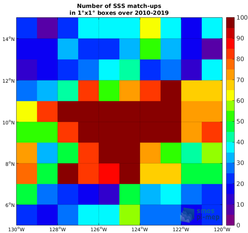
Figure 4: Number of SSS match-ups between Argo SSS and the SMOS-L3-CATDS-CECOS-LOCEAN-V4-18DAYS-25KM SSS product for the SPURS 2 Pi-MEP region over 1°x1° boxes and for the full satellite product period.
