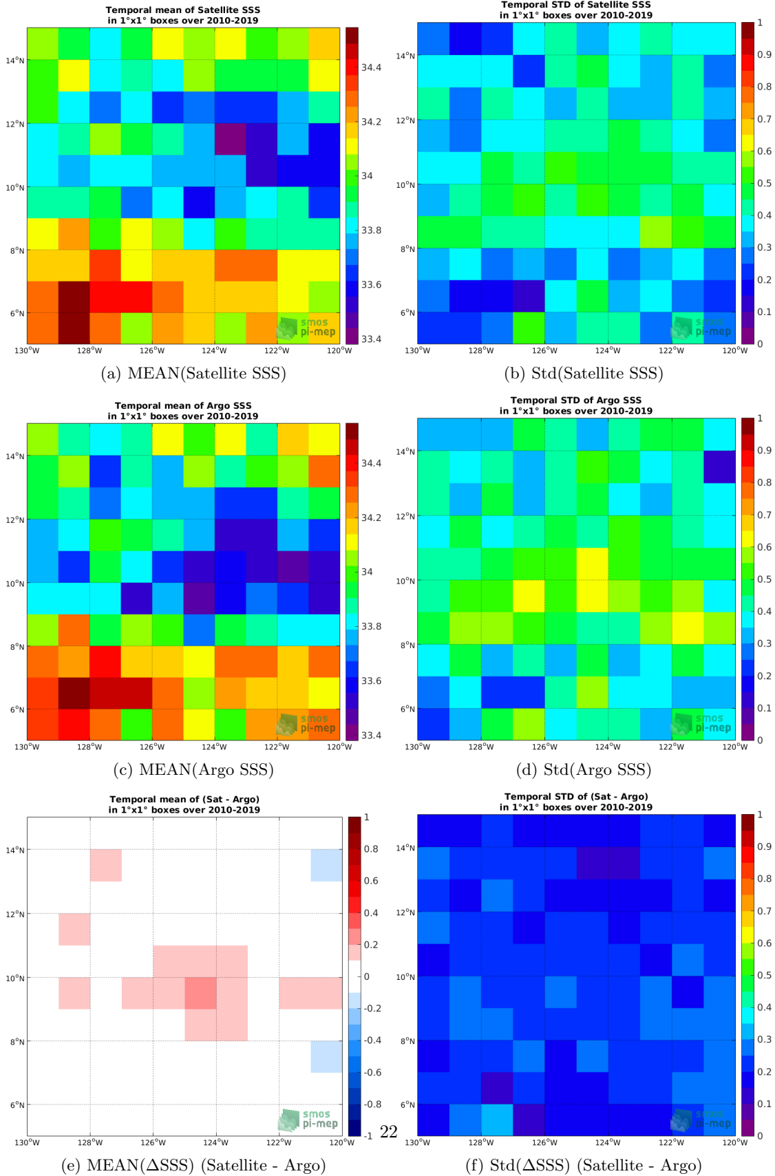
Figure 6: Temporal mean (left) and Std (right) of SSS from SMOS-L3-CATDS-CECOS-LOCEAN-V4-18DAYS-25KM (top), Argo (middle), and of \Delta SSS (Satellite - Argo). Only match-up pairs are used to generate these maps.
