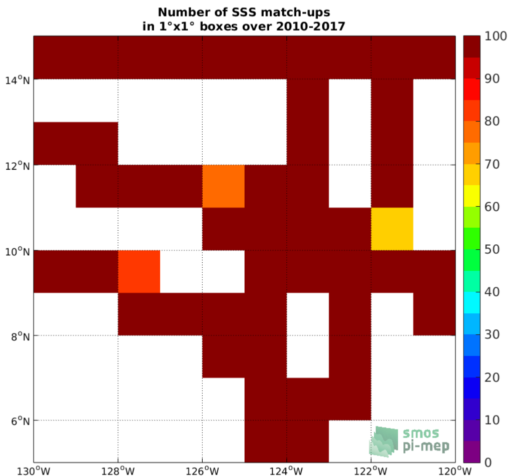
Figure 4: Number of SSS match-ups between TSG-SAMOS SSS and the SMOS-L3-CATDS-CECOS-LOCEAN-V3-9DAYS-25KM SSS product for the SPURS 2 Pi-MEP region over 1°x1° boxes and for the full satellite product period.
