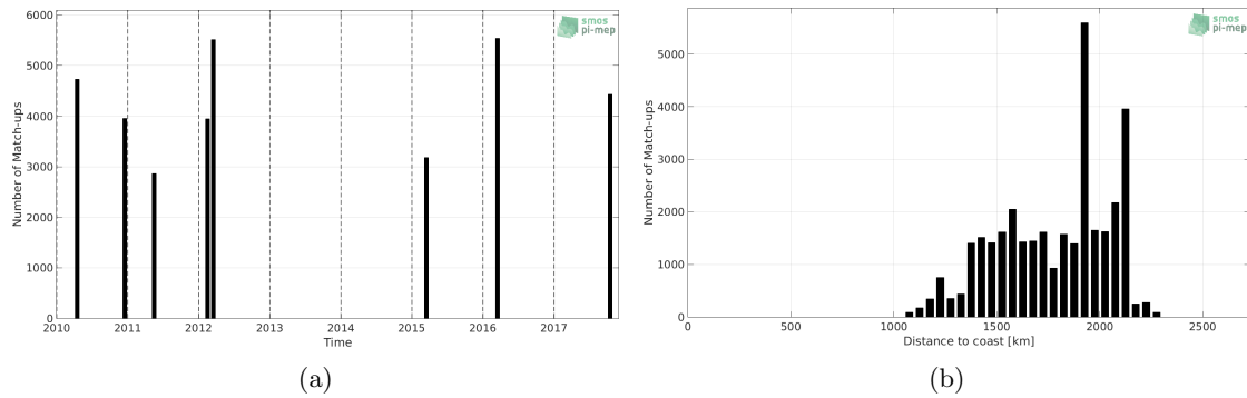
Figure 1: Number of match-ups between TSG-SAMOS and SMOS-L3-CATDS-CECOS-LOCEAN-V3-9DAYS-25KM SSS as a function of time (a) and as function of the distance to coast (b) over the SPURS 2 Pi-MEP region and for the full satellite product period.
