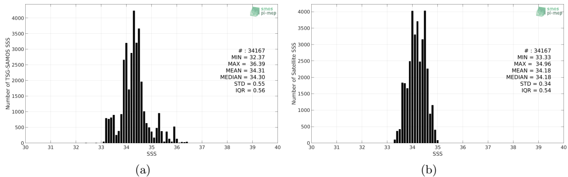
Figure 2: Histograms of SSS from TSG-SAMOS (a) and SMOS-L3-CATDS-CECOS-LOCEAN-V3-9DAYS-25KM (b) considering all match-up pairs per bins of 0.1 over the SPURS 2 Pi-MEP region and for the full satellite product period.
