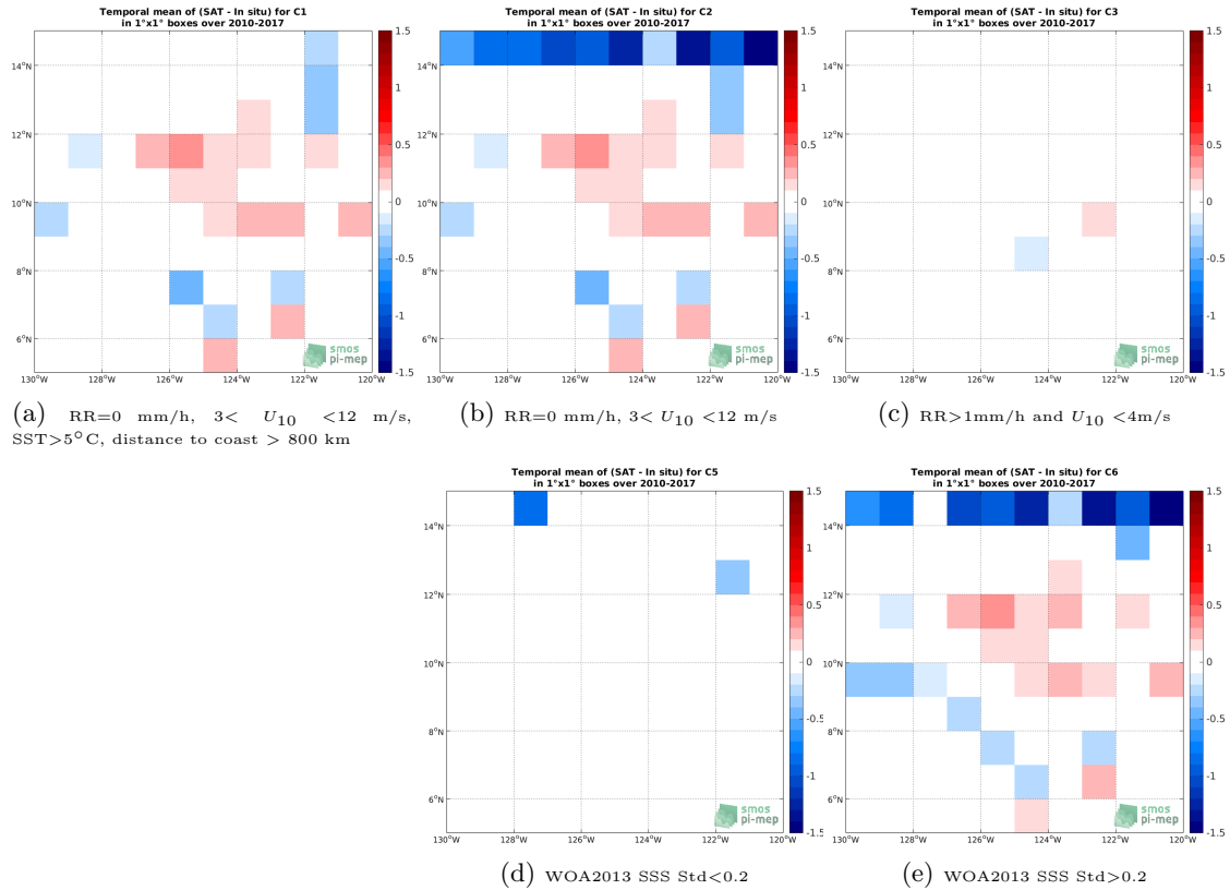
Figure 12: Temporal mean gridded over spatial boxes of size 1^\circ \times 1^\circ of \Delta SSS (SMOS-L3-CATDS-CECOS-LOCEAN-V3-9DAYS-25KM - TSG-SAMOS) for 5 different subdatasets corresponding to:RR=0 mm/h, 3 < U_{10} < 12 m/s, SST >5^\circ\text{C} , distance to coast > 800 km (a), RR=0 mm/h, 3 < U_{10} < 12 m/s (b), RR >1 mm/h and U_{10} < 4 m/s (c), WOA2013 SSS Std <0.2 (d), WOA2013 SSS Std >0.2 (e).
