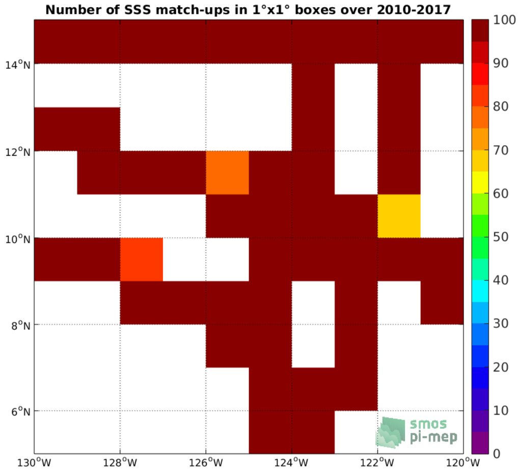
Figure 4: Number of SSS match-ups between TSG-SAMOS SSS and the SMOS-L3-CATDS-CECOS-LOCEAN-V3-9DAYS-25KM SSS product for the SPURS 2 Pi-MEP region over 1°x1° boxes and for the full satellite product period.
