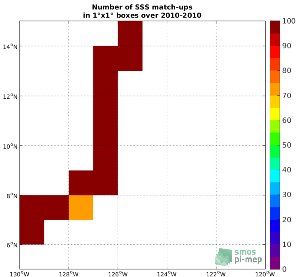
Figure 4: Number of SSS match-ups between TSG-GOSUD-Sailing-ship SSS and the SMOS-L3-CATDS-CECOS-LOCEAN-V3-9DAYS-25KM SSS product for the SPURS 2 Pi-MEP region over 1°x1° boxes and for the full satellite product period.
