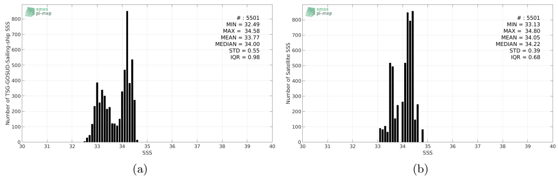
Figure 2: Histograms of SSS from TSG-GOSUD-Sailing-ship (a) and SMOS-L3-CATDS-CECOS-LOCEAN-V3-9DAYS-25KM (b) considering all match-up pairs per bins of 0.1 over the SPURS 2 Pi-MEP region and for the full satellite product period.
