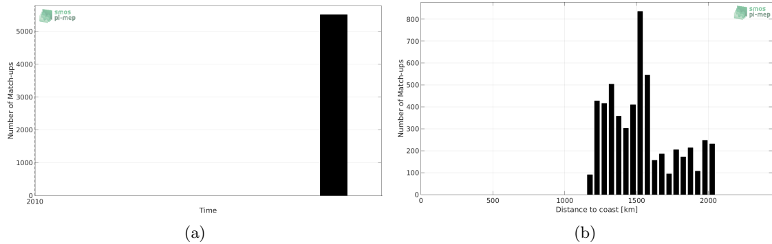
Figure 1: Number of match-ups between TSG-GOSUD-Sailing-ship and SMOS-L3-CATDS-CECOS-LOCEAN-V3-9DAYS-25KM SSS as a function of time (a) and as function of the distance to coast (b) over the SPURS 2 Pi-MEP region and for the full satellite product period.
