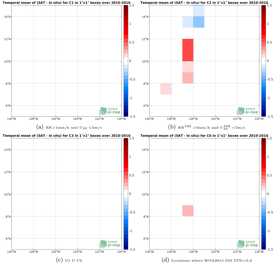
Figure 12: Temporal mean gridded over spatial boxes of size 1^\circ \times 1^\circ of \Delta SSS (SMOS-L3-CATDS-CECOS-LOCEAN-V3-9DAYS-25KM - TSG-GOSUD-Sailing-ship) for 4 different subdatasets corresponding to: RR > 1\text{mm/h} and U_{10} < 5\text{m/s} (a), RR^{10d} > 5\text{mm/h} and U_{10}^{10d} < 5\text{m/s} (b), C1 U C2 (c), Locations where WOA2013 SSS STD > 0.2 (d).
