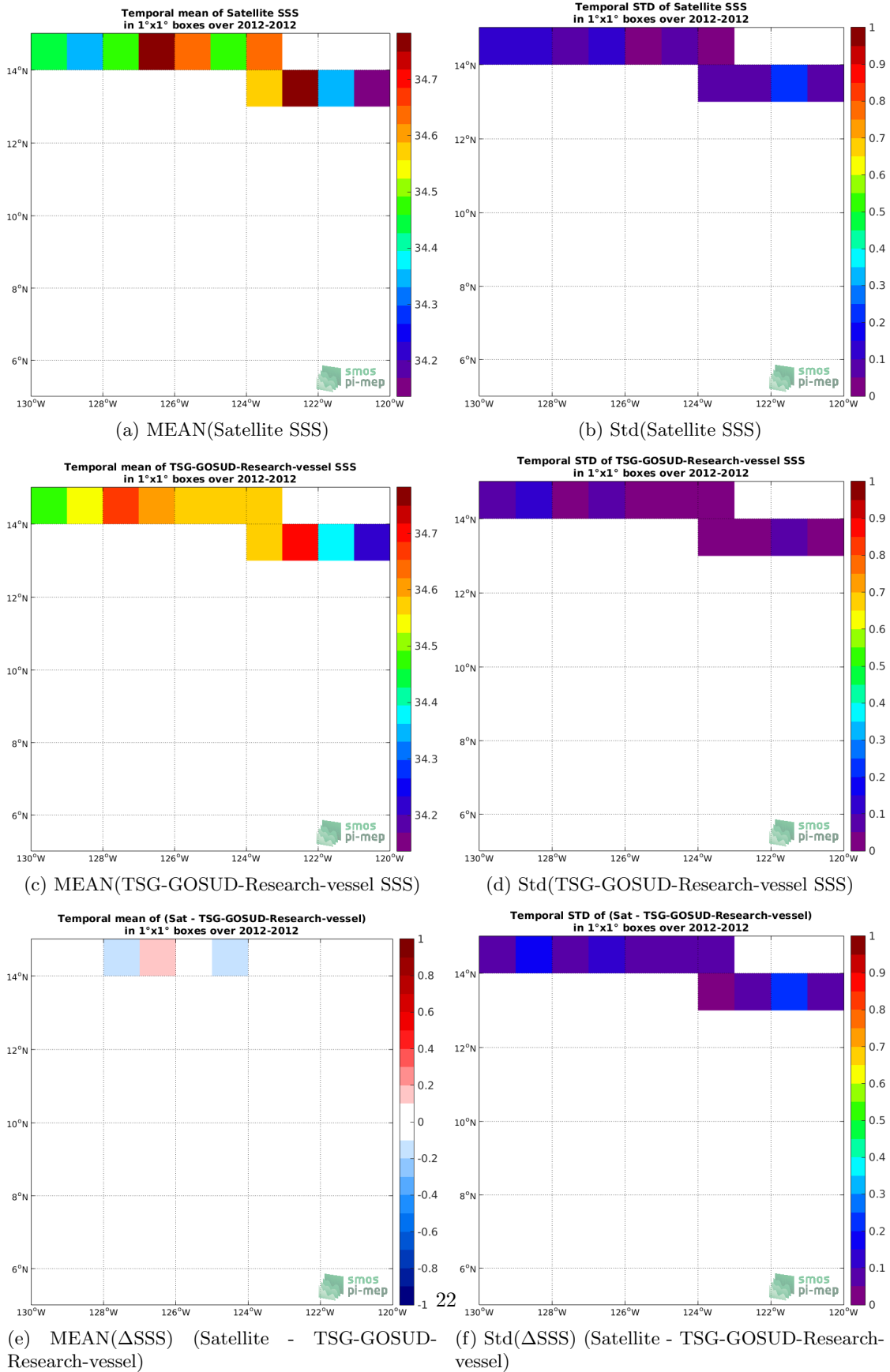
Figure 6: Temporal mean (left) and Std (right) of SSS from SMOS-L3-CATDS-CECOS-LOCEAN-V3-9DAYS-25KM (top), TSG-GOSUD-Research-vessel (middle), and of \Delta SSS (Satellite - TSG-GOSUD-Research-vessel). Only match-up pairs are used to generate these maps.
