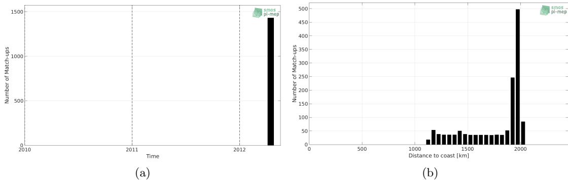
Figure 1: Number of match-ups between TSG-GOSUD-Research-vessel and SMOS-L3-CATDS-CECOS-LOCEAN-V3-9DAYS-25KM SSS as a function of time (a) and as function of the distance to coast (b) over the SPURS 2 Pi-MEP region and for the full satellite product period.
