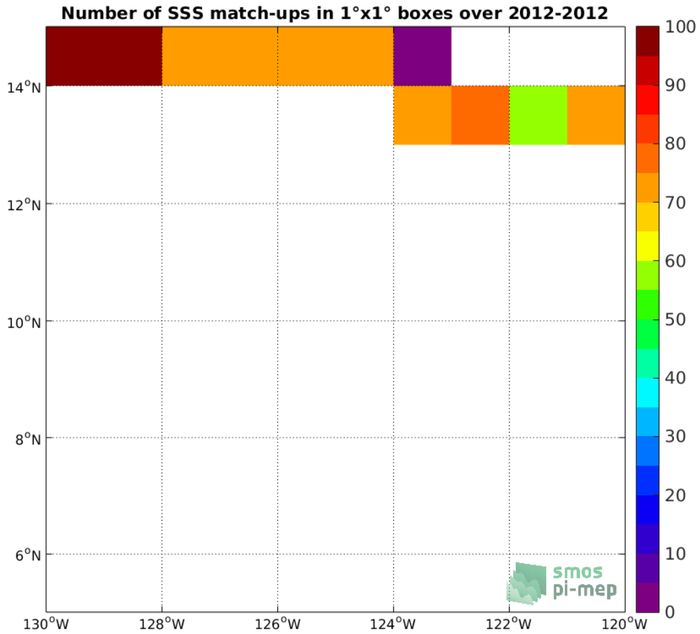
Figure 4: Number of SSS match-ups between TSG-GOSUD-Research-vessel SSS and the SMOS-L3-CATDS-CECOS-LOCEAN-V3-9DAYS-25KM SSS product for the SPURS 2 Pi-MEP region over 1°x1° boxes and for the full satellite product period.
