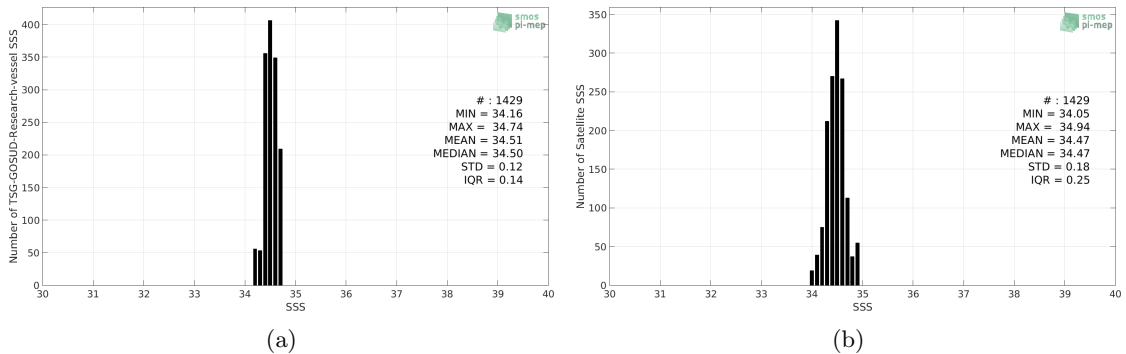
Figure 2: Histograms of SSS from TSG-GOSUD-Research-vessel (a) and SMOS-L3-CATDS-CECOS-LOCEAN-V3-9DAYS-25KM (b) considering all match-up pairs per bins of 0.1 over the SPURS 2 Pi-MEP region and for the full satellite product period.
