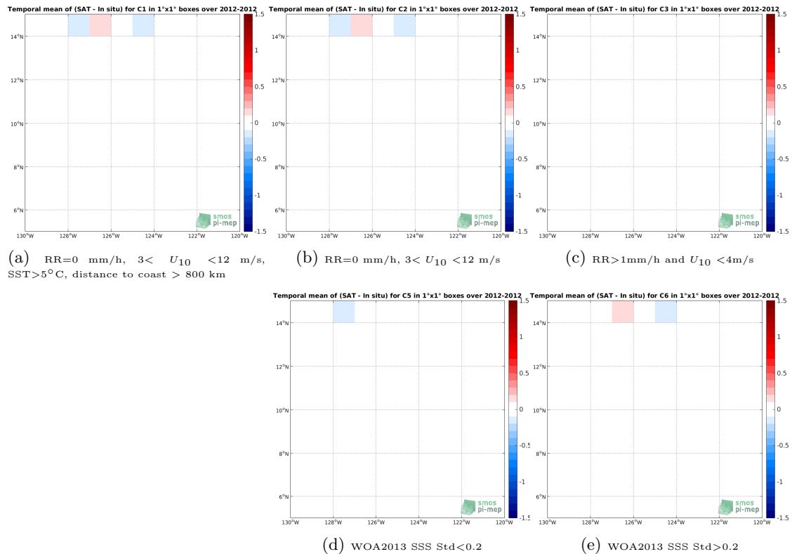
Figure 12: Temporal mean gridded over spatial boxes of size 1^\circ \times 1^\circ of \Delta SSS (SMOS-L3-CATDS-CECOS-LOCEAN-V3-9DAYS-25KM - TSG-GOSUD-Research-vessel) for 5 different subdatasets corresponding to:RR=0 mm/h, 3 < U_{10} < 12 m/s, SST >5^\circ C, distance to coast > 800 km (a), RR=0 mm/h, 3 < U_{10} < 12 m/s (b), RR >1 mm/h and U_{10} < 4 m/s (c), WOA2013 SSS Std <0.2 (d), WOA2013 SSS Std >0.2 (e).
