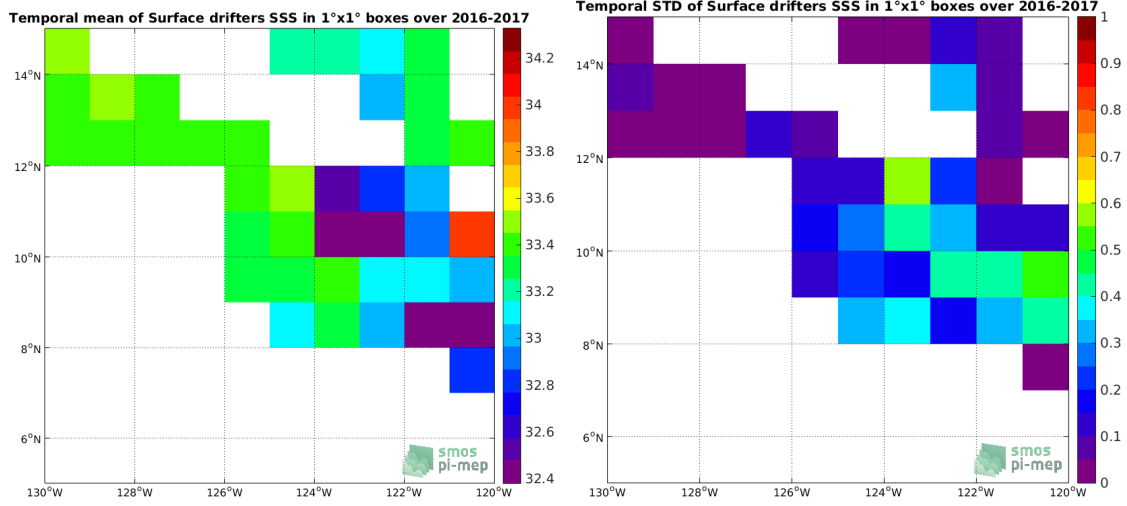
(c) MEAN(Surface drifters SSS)
