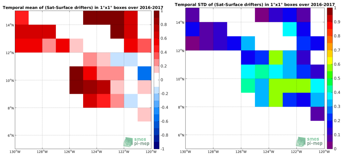
(e) MEAN( \Delta SSS) (Satellite - Surface drifters) 17 (f) STD( \Delta SSS) (Satellite - Surface drifters)
