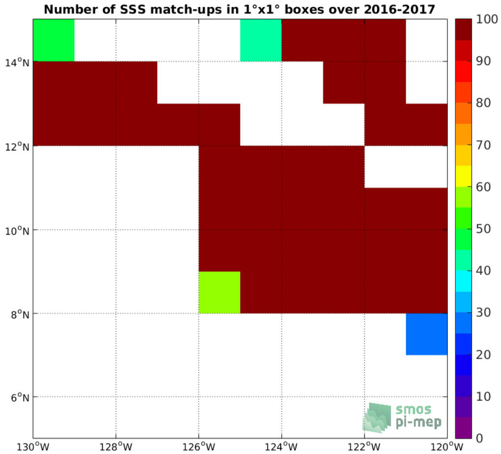
Figure 3: Number of SSS match-ups between Surface drifters SSS and the SMOS-L3-CATDS-CECOS-LOCEAN-V3-9DAYS-25KM SSS product for the SPURS 2 Pi-MEP region over 1°x1° boxes and for the full satellite product period.
