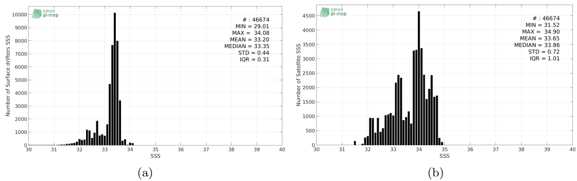
Figure 2: Histograms of SSS from Surface drifters (a) and SMOS-L3-CATDS-CECOS-LOCEAN-V3-9DAYS-25KM (b) considering all match-up pairs per bins of 0.1 over the SPURS 2 Pi-MEP region and for the full satellite product period.
