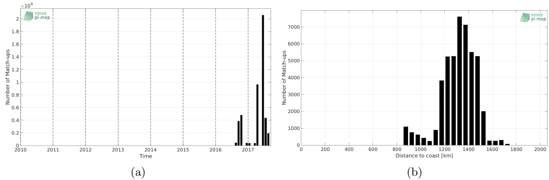
Figure 1: Number of match-ups between Surface drifters and SMOS-L3-CATDS-CECOS-LOCEAN-V3-9DAYS-25KM SSS as a function of time (a) and as function of the distance to coast (b) over the SPURS 2 Pi-MEP region and for the full satellite product period.
