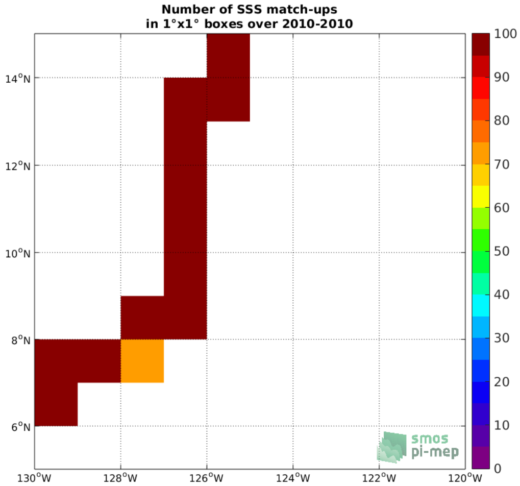
Figure 4: Number of SSS match-ups between TSG-GOSUD-Sailing-ship SSS and the SMOS-L3-CATDS-CECOS-LOCEAN-V3-18DAYS-25KM SSS product for the SPURS 2 Pi-MEP region over 1°x1° boxes and for the full satellite product period.
