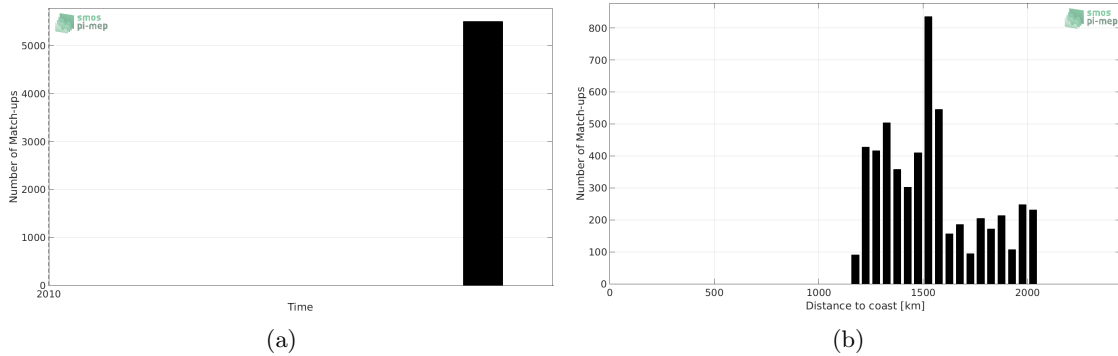
Figure 1: Number of match-ups between TSG-GOSUD-Sailing-ship and SMOS-L3-CATDS-CECOS-LOCEAN-V3-18DAYS-25KM SSS as a function of time (a) and as function of the distance to coast (b) over the SPURS 2 Pi-MEP region and for the full satellite product period.
