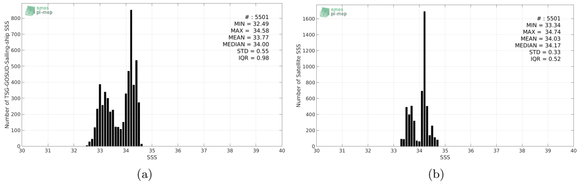
Figure 2: Histograms of SSS from TSG-GOSUD-Sailing-ship (a) and SMOS-L3-CATDS-CECOS-LOCEAN-V3-18DAYS-25KM (b) considering all match-up pairs per bins of 0.1 over the SPURS 2 Pi-MEP region and for the full satellite product period.
