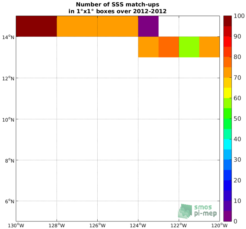
Figure 4: Number of SSS match-ups between TSG-GOSUD-Research-vessel SSS and the SMOS-L3-CATDS-CECOS-LOCEAN-V3-18DAYS-25KM SSS product for the SPURS 2 Pi-MEP region over 1°x1° boxes and for the full satellite product period.
