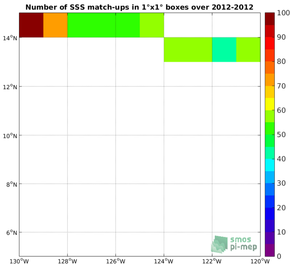
Figure 4: Number of SSS match-ups between TSG-GOSUD-Research-vessel SSS and the SMOS-L3-CATDS-CECOS-LOCEAN-V3-18DAYS-25KM SSS product for the SPURS 2 Pi-MEP region over 1°x1° boxes and for the full satellite product period.
