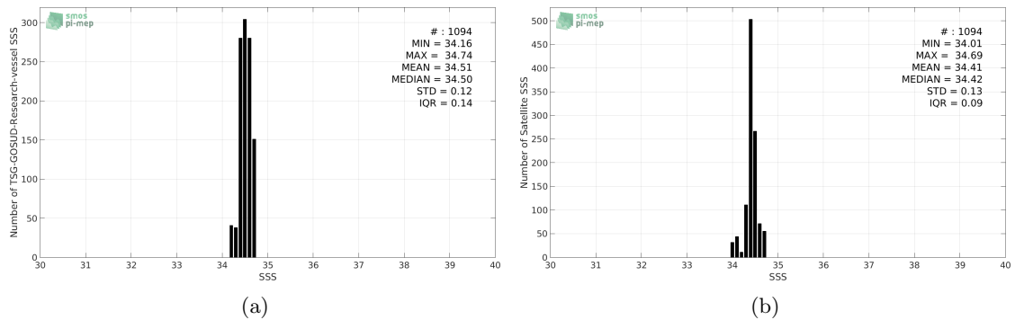
Figure 2: Histograms of SSS from TSG-GOSUD-Research-vessel (a) and SMOS-L3-CATDS-CECOS-LOCEAN-V3-18DAYS-25KM (b) considering all match-up pairs per bins of 0.1 over the SPURS 2 Pi-MEP region and for the full satellite product period.
