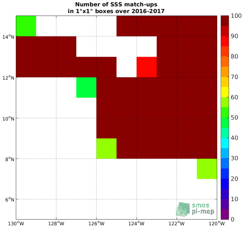
Figure 3: Number of SSS match-ups between Surface drifters SSS and the SMOS-L3-CATDS-CECOS-LOCEAN-V3-18DAYS-25KM SSS product for the SPURS 2 Pi-MEP region over 1°x1° boxes and for the full satellite product period.
