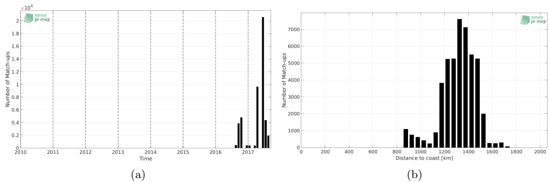
Figure 1: Number of match-ups between Surface drifters and SMOS-L3-CATDS-CECOS-LOCEAN-V3-18DAYS-25KM SSS as a function of time (a) and as function of the distance to coast (b) over the SPURS 2 Pi-MEP region and for the full satellite product period.
