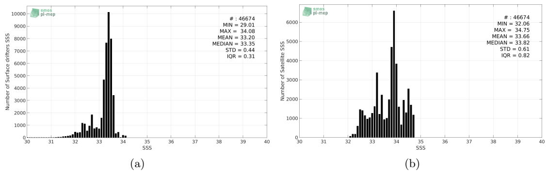
Figure 2: Histograms of SSS from Surface drifters (a) and SMOS-L3-CATDS-CECOS-LOCEAN-V3-18DAYS-25KM (b) considering all match-up pairs per bins of 0.1 over the SPURS 2 Pi-MEP region and for the full satellite product period.
