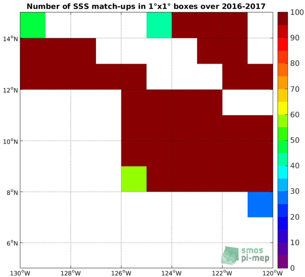
Figure 3: Number of SSS match-ups between Surface drifters SSS and the SMOS-L3-CATDS-CECOS-LOCEAN-V3-18DAYS-25KM SSS product for the SPURS 2 Pi-MEP region over 1°x1° boxes and for the full satellite product period.
