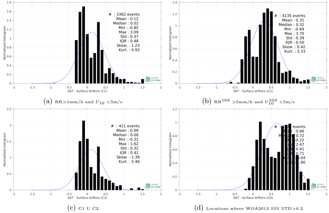
Figure 12: Normalized histogram of \Delta SSS (SMOS-L3-CATDS-CECOS-LOCEAN-V3-18DAYS-25KM - Surface drifters) for 6 different subdatasets corresponding to: RR > 1\text{mm/h} and U_{10} < 5\text{m/s} (a), RR^{10d} > 5\text{mm/h} and U_{10}^{10d} < 5\text{m/s} (b), C1 U C2 (c), Locations where WOA2013 SSS STD > 0.2 (d).
