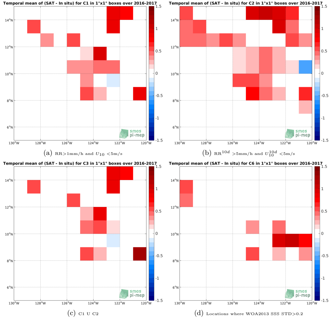
Figure 11: Temporal mean gridded over spatial boxes of size 1^\circ \times 1^\circ of \Delta SSS (SMOS-L3-CATDS-CECOS-LOCEAN-V3-18DAYS-25KM - Surface drifters) for 4 different subdatasets corresponding to: RR > 1 mm/h and U_{10} < 5 m/s (a), RR 10d > 5 mm/h and U_{10}^{10d} < 5 m/s (b), C1 U C2 (c), Locations where WOA2013 SSS STD > 0.2 (d).
