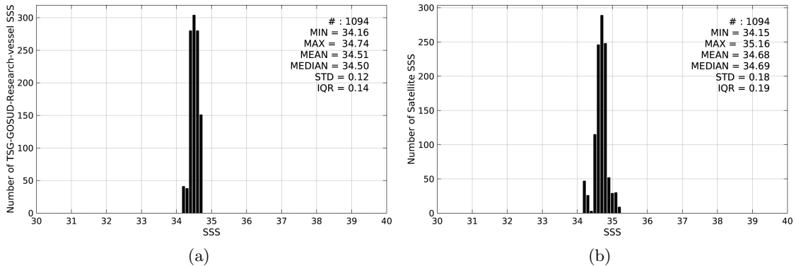
Figure 2: Histograms of SSS from TSG-GOSUD-Research-vessel (a) and SMOS-L3-CATDS-CECOS-LOCEAN-V2.1-9DAYS-25KM (b) considering all match-up pairs per bins of 0.1 over the SPURS 2 Pi-MEP region and for the full satellite product period.
