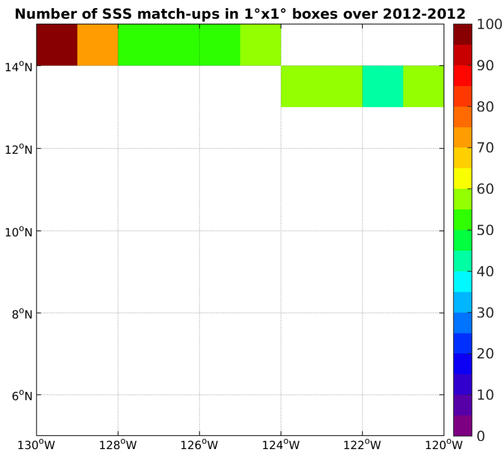
Figure 4: Number of SSS match-ups between TSG-GOSUD-Research-vessel SSS and the SMOS-L3-CATDS-CECOS-LOCEAN-V2-9DAYS-25KM SSS product for the SPURS 2 Pi-MEP region over 1°x1° boxes and for the full satellite product period.
