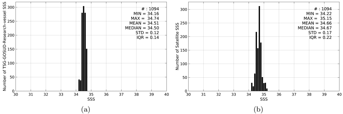
Figure 2: Histograms of SSS from TSG-GOSUD-Research-vessel (a) and SMOS-L3-CATDS-CECOS-LOCEAN-V2-9DAYS-25KM (b) considering all match-up pairs per bins of 0.1 over the SPURS 2 Pi-MEP region and for the full satellite product period.
