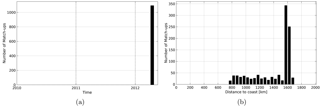
Figure 1: Number of match-ups between TSG-GOSUD-Research-vessel and SMOS-L3-CATDS-CECOS-LOCEAN-V2-9DAYS-25KM SSS as a function of time (a) and as function of the distance to coast (b) over the SPURS 2 Pi-MEP region and for the full satellite product period.
