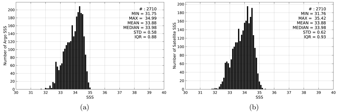
Figure 2: Histograms of SSS from Argo (a) and SMOS-L3-CATDS-CECOS-LOCEAN-V2-9DAYS-25KM (b) considering all match-up pairs per bins of 0.1 over the SPURS 2 Pi-MEP region and for the full satellite product period.
