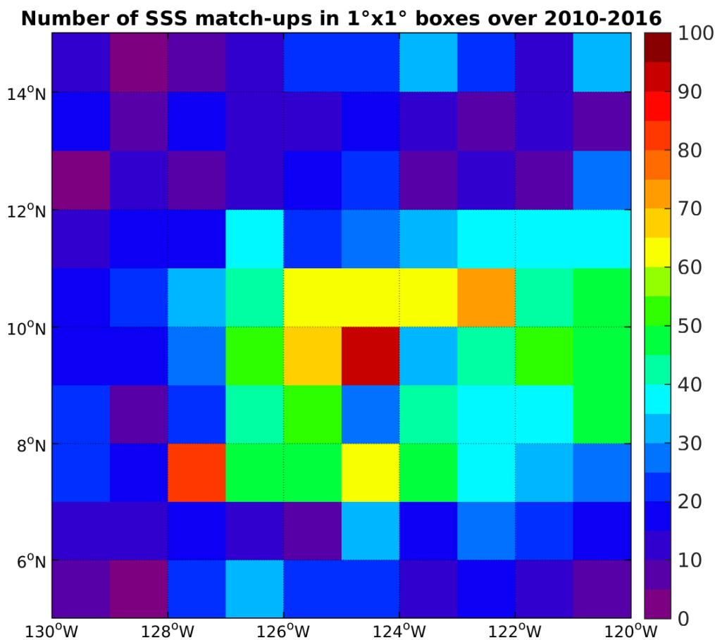
Figure 4: Number of SSS match-ups between Argo SSS and the SMOS-L3-CATDS-CECOS-LOCEAN-V2-9DAYS-25KM SSS product for the SPURS 2 Pi-MEP region over 1°x1° boxes and for the full satellite product period.
