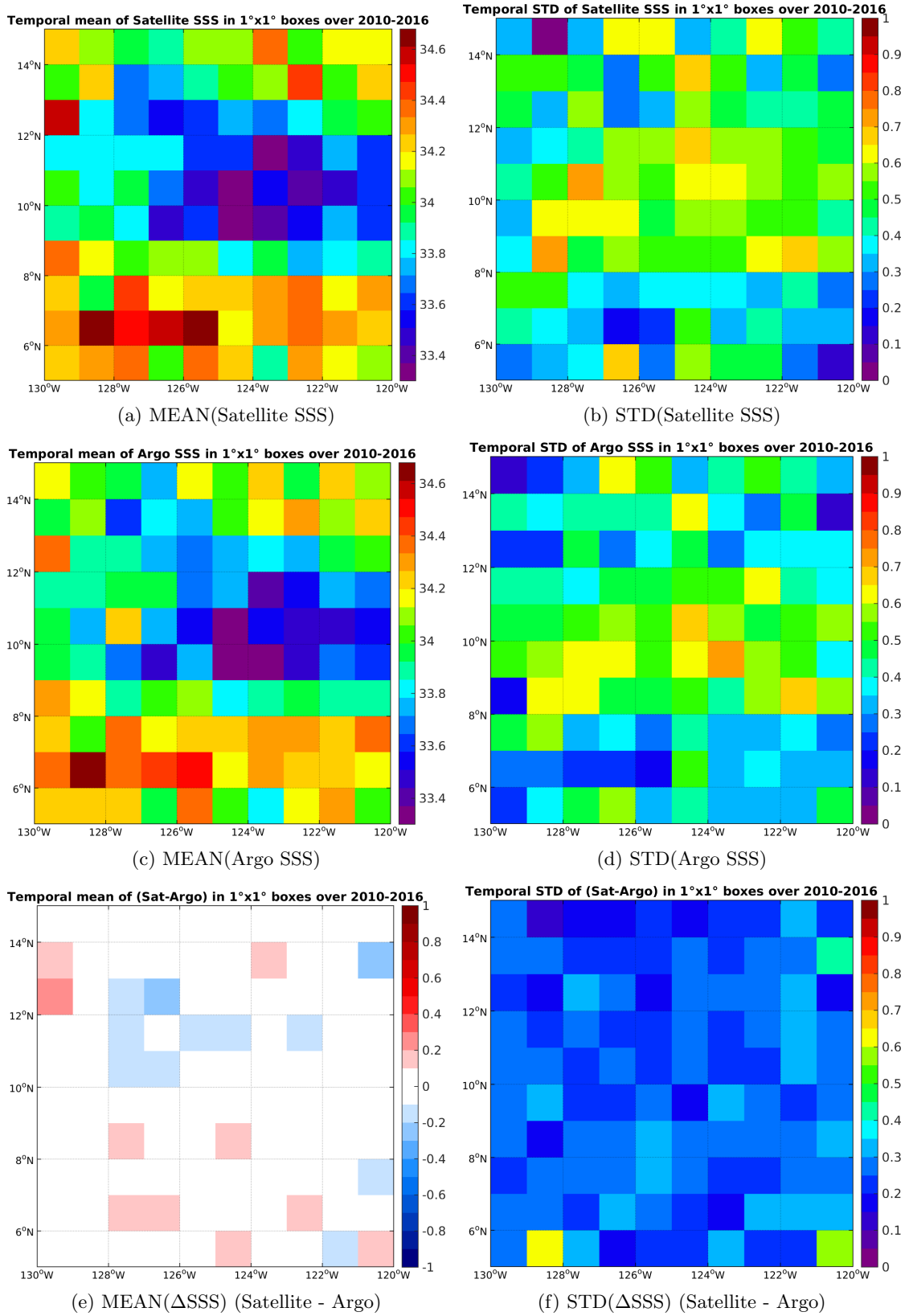
Figure 6: Temporal mean (left) and STD (right) of SSS from SMOS-L3-CATDS-CECOS-LOCEAN-V2-9DAYS-25KM (top), Argo (middle), and of \Delta SSS (Satellite - Argo). Only match-up pairs are used to generate these maps.
