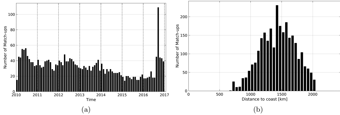
Figure 1: Number of match-ups between Argo and SMOS-L3-CATDS-CECOS-LOCEAN-V2-9DAYS-25KM SSS as a function of time (a) and as function of the distance to coast (b) over the SPURS 2 Pi-MEP region and for the full satellite product period.
