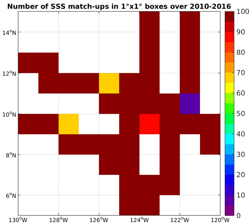
Figure 4: Number of SSS match-ups between TSG-SAMOS SSS and the SMOS-L3-CATDS-CECOS-LOCEAN-V2-18DAYS-25KM SSS product for the SPURS 2 Pi-MEP region over 1°x1° boxes and for the full satellite product period.
