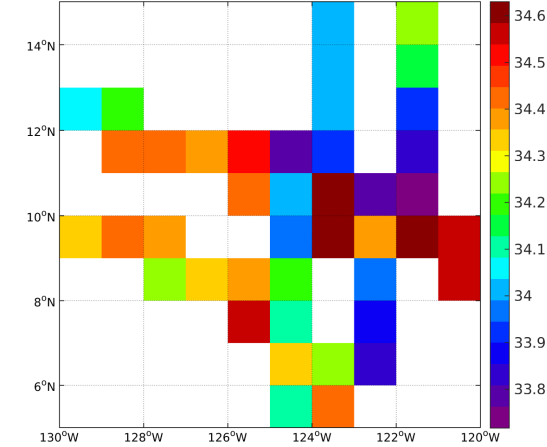
(c) MEAN(TSG-SAMOS SSS)
