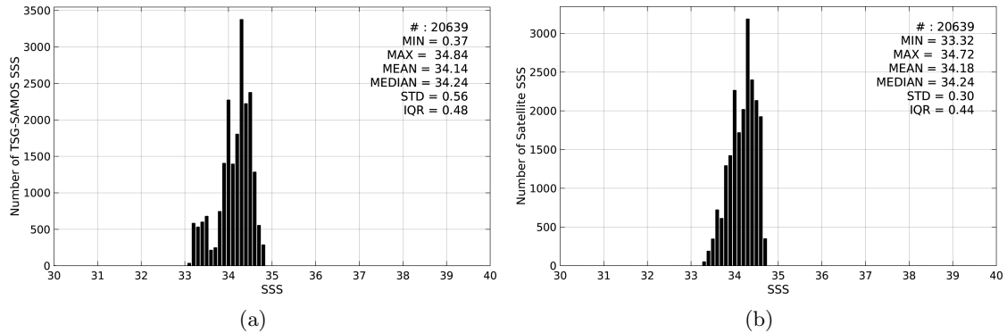
Figure 2: Histograms of SSS from TSG-SAMOS (a) and SMOS-L3-CATDS-CECOS-LOCEAN-V2-18DAYS-25KM (b) considering all match-up pairs per bins of 0.1 over the SPURS 2 Pi-MEP region and for the full satellite product period.
