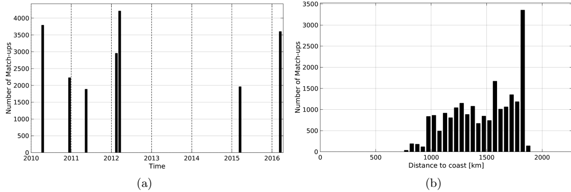
Figure 1: Number of match-ups between TSG-SAMOS and SMOS-L3-CATDS-CECOS-LOCEAN-V2-18DAYS-25KM SSS as a function of time (a) and as function of the distance to coast (b) over the SPURS 2 Pi-MEP region and for the full satellite product period.
