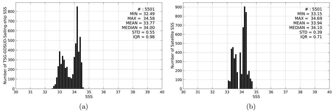
Figure 2: Histograms of SSS from TSG-GOSUD-Sailing-ship (a) and SMOS-L3-CATDS-CECOS-LOCEAN-V2-18DAYS-25KM (b) considering all match-up pairs per bins of 0.1 over the SPURS 2 Pi-MEP region and for the full satellite product period.
