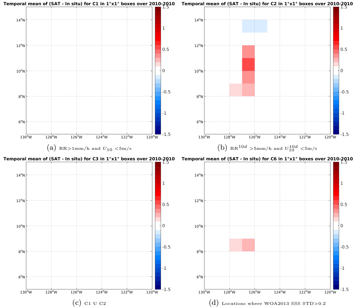
Figure 12: Temporal mean gridded over spatial boxes of size 1^\circ \times 1^\circ of \Delta SSS (SMOS-L3-CATDS-CECOS-LOCEAN-V2-18DAYS-25KM - TSG-GOSUD-Sailing-ship) for 4 different subdatasets corresponding to: RR > 1\text{mm/h} and U_{10} < 5\text{m/s} (a), RR^{10d} > 5\text{mm/h} and U_{10}^{10d} < 5\text{m/s} (b), C1 U C2 (c), Locations where WOA2013 SSS STD > 0.2 (d).
