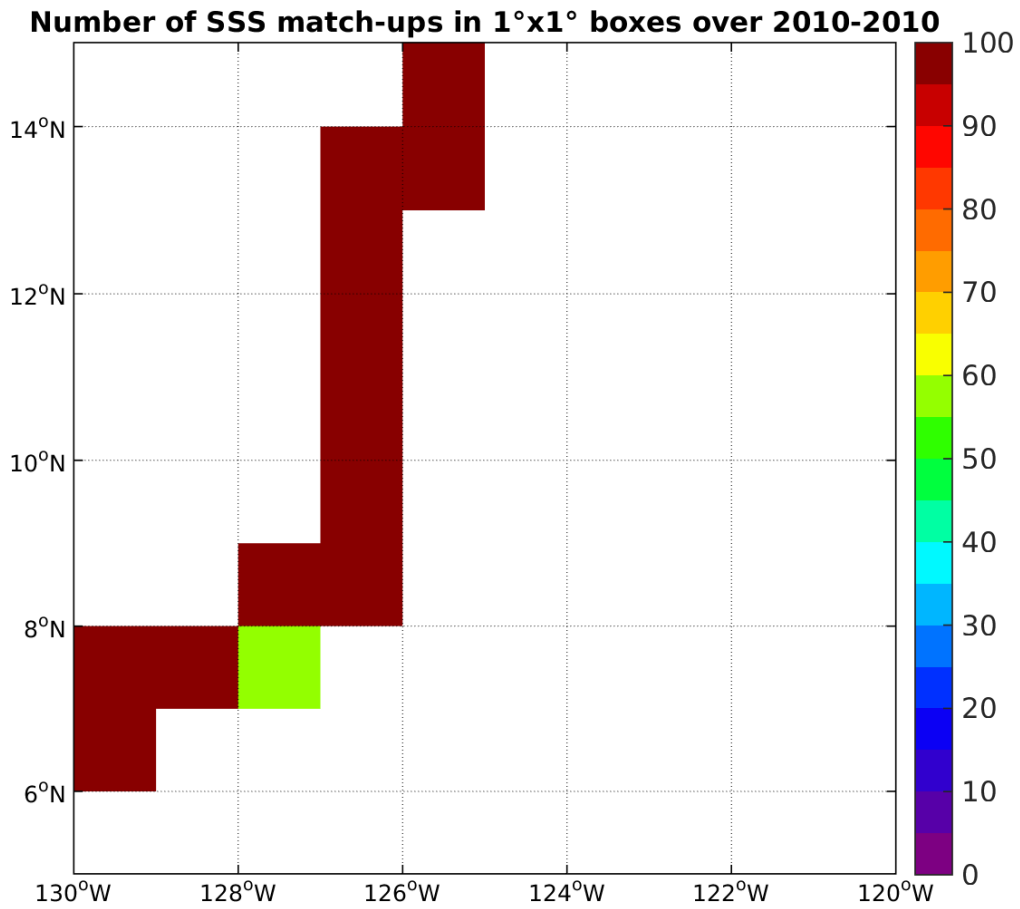
Figure 4: Number of SSS match-ups between TSG-GOSUD-Sailing-ship SSS and the SMOS-L3-CATDS-CECOS-LOCEAN-V2-18DAYS-25KM SSS product for the SPURS 2 Pi-MEP region over 1°x1° boxes and for the full satellite product period.
