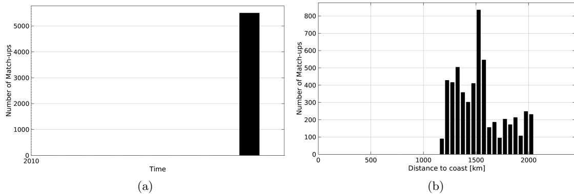
Figure 1: Number of match-ups between TSG-GOSUD-Sailing-ship and SMOS-L3-CATDS-CECOS-LOCEAN-V2-18DAYS-25KM SSS as a function of time (a) and as function of the distance to coast (b) over the SPURS 2 Pi-MEP region and for the full satellite product period.
