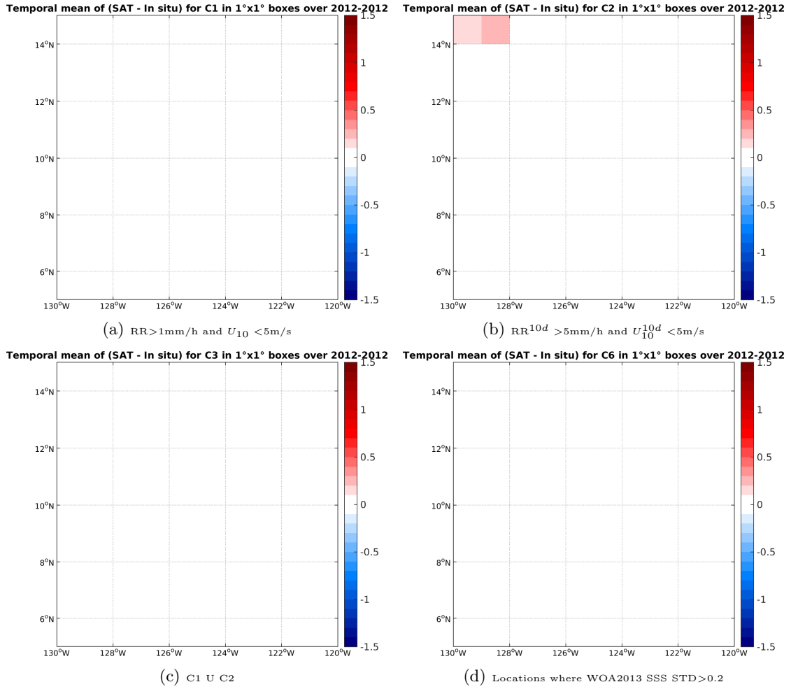
Figure 12: Temporal mean gridded over spatial boxes of size 1°x1° of \Delta SSS (SMOS-L3-CATDS-CECOS-LOCEAN-V2-18DAYS-25KM - TSG-GOSUD-Research-vessel) for 4 different subdatasets corresponding to: RR > 1\text{mm/h} and U_{10} < 5\text{m/s} (a), RR^{10d} > 5\text{mm/h} and U_{10}^{10d} < 5\text{m/s} (b), C1 U C2 (c), Locations where WOA2013 SSS STD > 0.2 (d).
