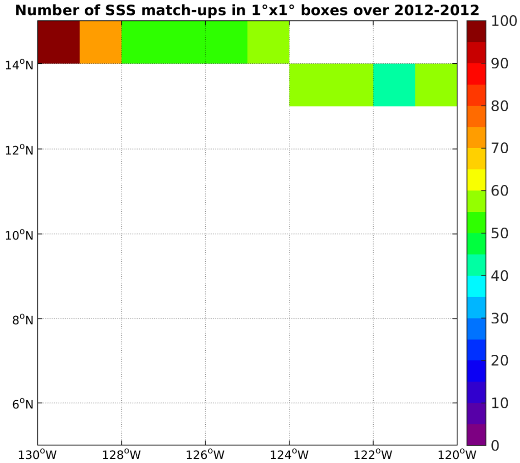
Figure 4: Number of SSS match-ups between TSG-GOSUD-Research-vessel SSS and the SMOS-L3-CATDS-CECOS-LOCEAN-V2-18DAYS-25KM SSS product for the SPURS 2 Pi-MEP region over 1°x1° boxes and for the full satellite product period.
