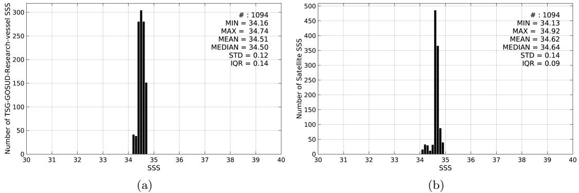
Figure 2: Histograms of SSS from TSG-GOSUD-Research-vessel (a) and SMOS-L3-CATDS-CECOS-LOCEAN-V2-18DAYS-25KM (b) considering all match-up pairs per bins of 0.1 over the SPURS 2 Pi-MEP region and for the full satellite product period.
