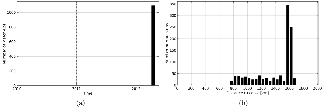
Figure 1: Number of match-ups between TSG-GOSUD-Research-vessel and SMOS-L3-CATDS-CECOS-LOCEAN-V2-18DAYS-25KM SSS as a function of time (a) and as function of the distance to coast (b) over the SPURS 2 Pi-MEP region and for the full satellite product period.
