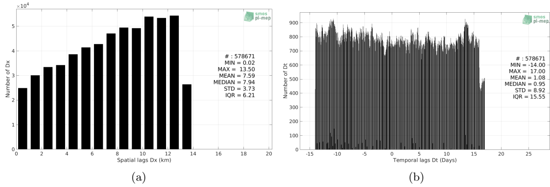
Figure 4: Histograms of the spatial (a) and temporal (b) lags between the location/time of the Waveglider measurement and the date of the corresponding SMOS SSS L3 v2 - Monthly - 0.25 Deg (CATDS-CECOS-IFREMER) SSS pixel.
