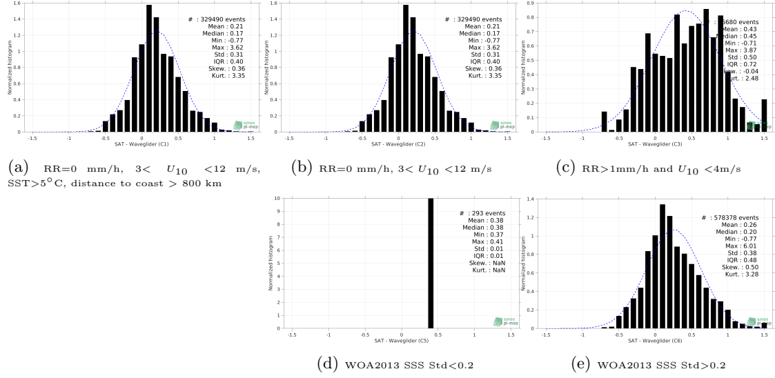
Figure 12: Normalized histogram of \Delta SSS (SMOS SSS L3 v2 - Monthly - 0.25 Deg (CATDS-CECOS-IFREMER) - Waveglider) for 5 different subdatasets corresponding to: RR=0 mm/h, 3 < U_{10} < 12 m/s, SST > 5°C, distance to coast > 800 km (a), RR=0 mm/h, 3 < U_{10} < 12 m/s (b), RR > 1mm/h and U_{10} < 4 m/s (c), WOA2013 SSS Std < 0.2 (d), WOA2013 SSS Std > 0.2 (e).
