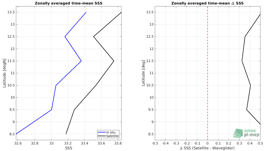
Figure 7: Left panel: Zonal mean SSS from SMOS SSS L3 v2 - Monthly - 0.25 Deg (CATDS-CECOS-IFREMER) satellite product (black) and from Waveglider (blue). Right panel: Zonal mean of \Delta SSS (Satellite - Waveglider) for all the collected Pi-MEP match-up pairs estimated over the full satellite product period.
