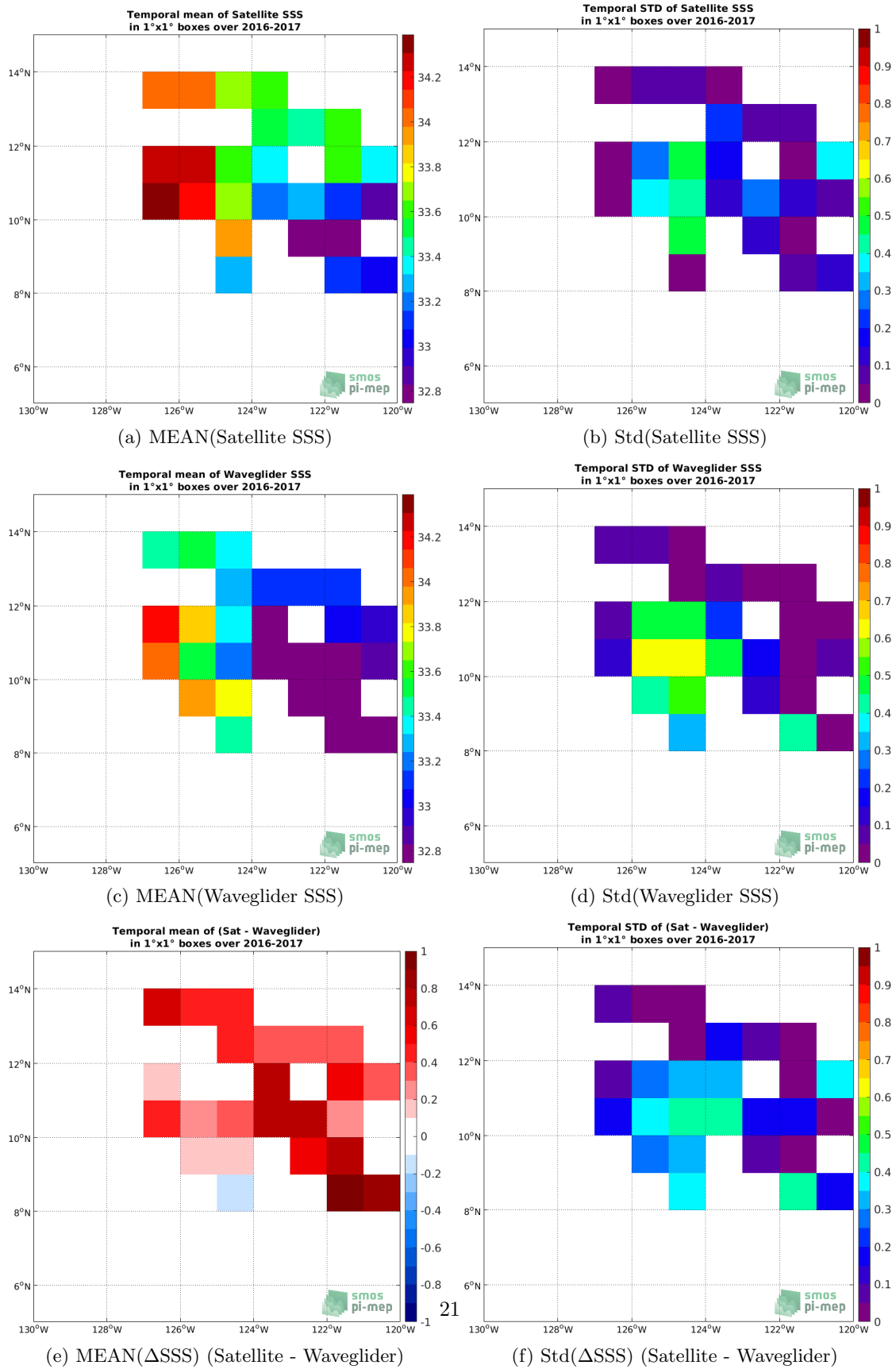
Figure 5: Temporal mean (left) and Std (right) of SSS from SMOS SSS L3 v2 - Monthly - 0.25 Deg (CATDS-CECOS-IFREMER) (top), Waveglider (middle), and of \Delta SSS (Satellite - Waveglider). Only match-up pairs are used to generate these maps.
