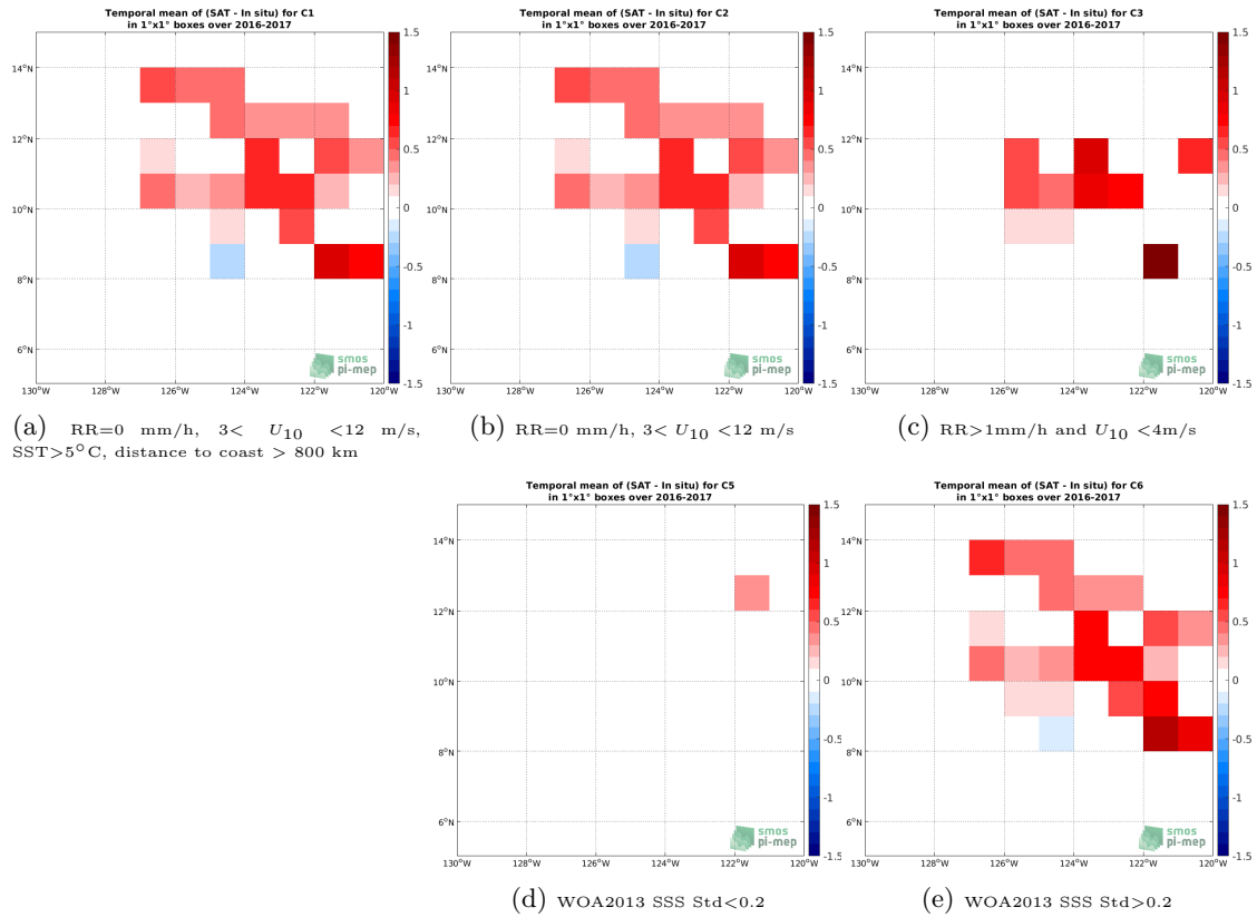
Figure 11: Temporal mean gridded over spatial boxes of size 1^{\circ}\times 1^{\circ} of \Delta\text{SSS} (SMOS SSS L3 v2 - Monthly - 0.25 Deg (CATDS-CECOS-IFREMER) - Waveglider) for 5 different subdatasets corresponding to:RR=0 mm/h, 3 < U_{10} < 12 m/s, SST >5^{\circ}\text{C} , distance to coast > 800 km (a), RR=0 mm/h, 3 < U_{10} < 12 m/s (b), RR >1 mm/h and U_{10} < 4 m/s (c), WOA2013 SSS Std <0.2 (d), WOA2013 SSS Std >0.2 (e).
