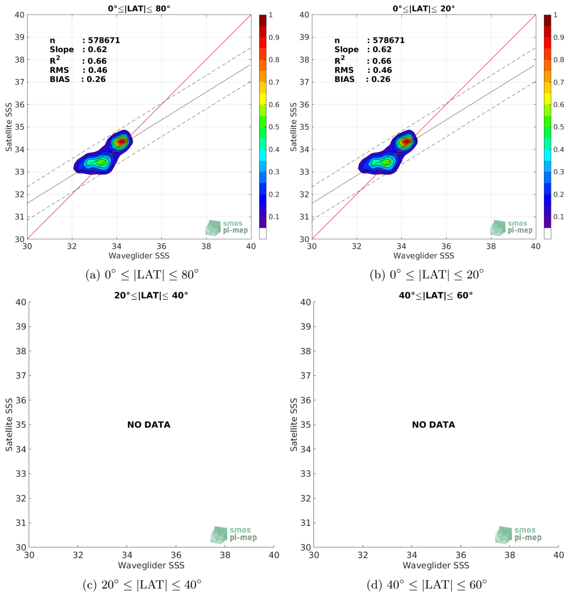
Figure 8: Contour maps of the concentration of SMOS SSS L3 v2 - Monthly - 0.25 Deg (CATDS-CECOS-IFREMER) SSS (y-axis) versus Waveglider SSS (x-axis) at match-up pairs for different latitude bands. For each plot, the red line shows x=y . The black thin and dashed lines indicate a linear fit through the data cloud and the \pm 95\% confidence levels, respectively. The number match-up pairs n , the slope and R^2 coefficient of the linear fit, the root mean square (RMS) and the mean bias between satellite and in situ data are indicated for each latitude band in each plots.
