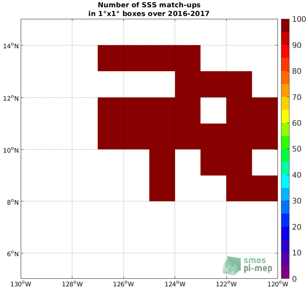
Figure 3: Number of SSS match-ups between Waveglider SSS and the SMOS SSS L3 v2 - Monthly - 0.25 Deg (CATDS-CECOS-IFREMER) SSS product for the SPURS 2 Pi-MEP region over 1^\circ \times 1^\circ boxes and for the full satellite product period.
