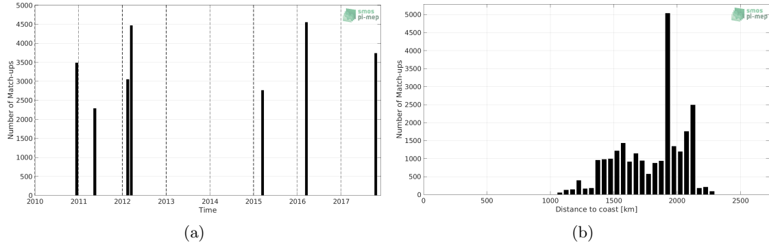
Figure 1: Number of match-ups between TSG (SAMOS) and SMOS SSS L3 v2 - Monthly - 0.25 Deg (CATDS-CECOS-IFREMER) SSS as a function of time (a) and as function of the distance to coast (b) over the SPURS 2 Pi-MEP region and for the full satellite product period.
