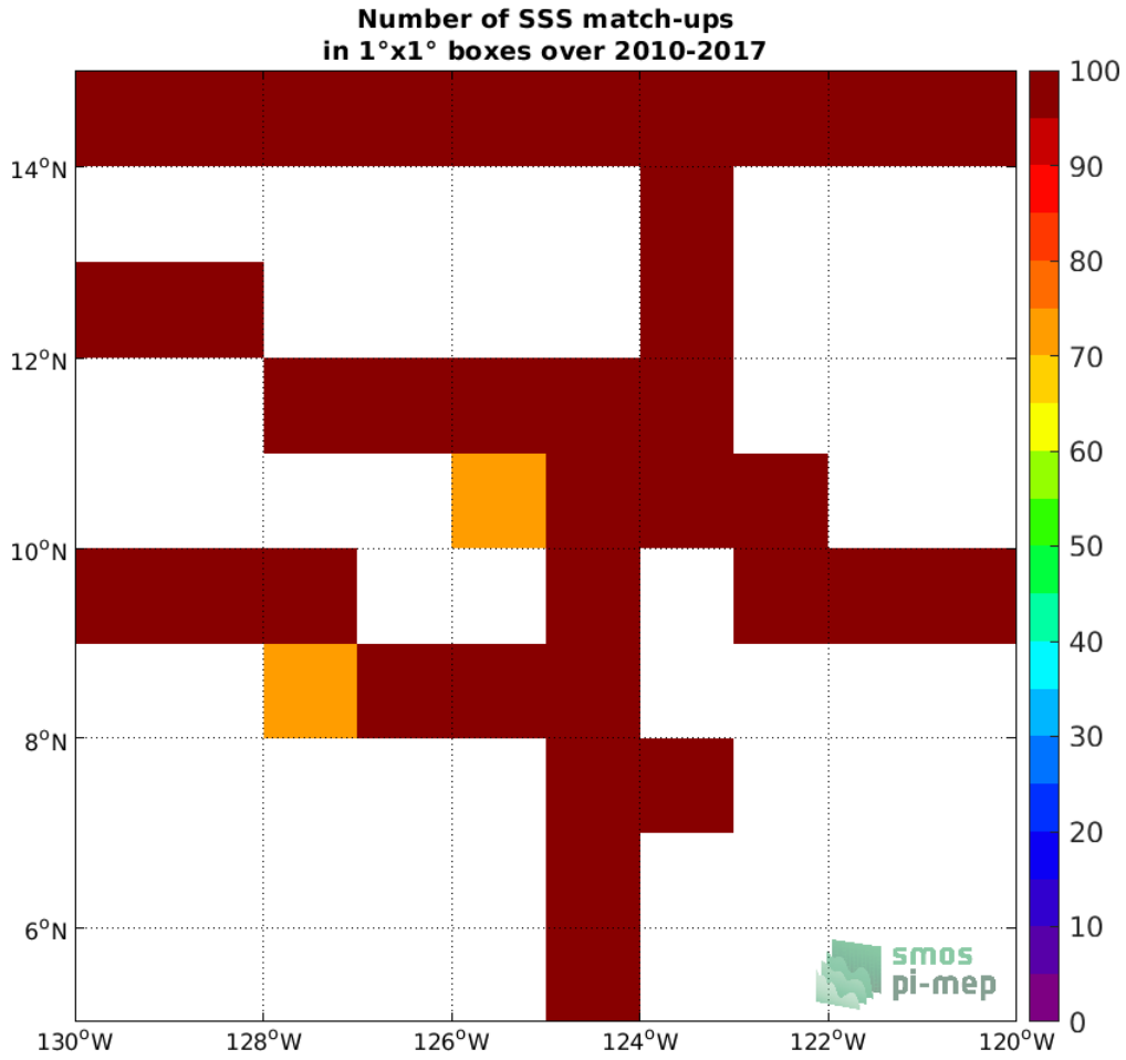
Figure 4: Number of SSS match-ups between TSG (SAMOS) SSS and the SMOS SSS L3 v2 - Monthly - 0.25 Deg (CATDS-CECOS-IFREMER) SSS product for the SPURS 2 Pi-MEP region over 1°x1° boxes and for the full satellite product period.
