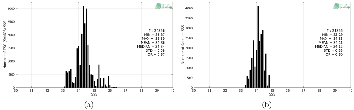
Figure 2: Histograms of SSS from TSG (SAMOS) (a) and SMOS SSS L3 v2 - Monthly - 0.25 Deg (CATDS-CECOS-IFREMER) (b) considering all match-up pairs per bins of 0.1 over the SPURS 2 Pi-MEP region and for the full satellite product period.
