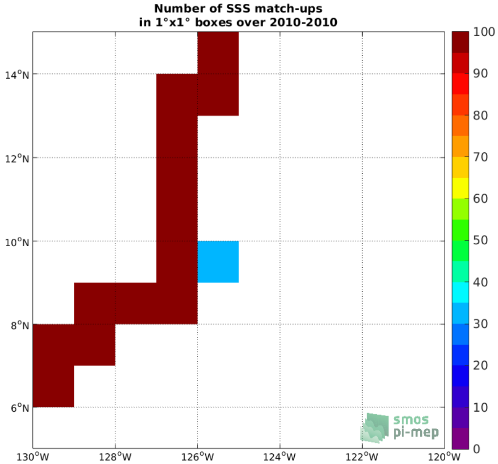
Figure 4: Number of SSS match-ups between TSG (GOSUD-Sailing-ship) SSS and the SMOS SSS L3 v2 - Monthly - 0.25 Deg (CATDS-CECOS-IFREMER) SSS product for the SPURS 2 Pi-MEP region over 1°x1° boxes and for the full satellite product period.
