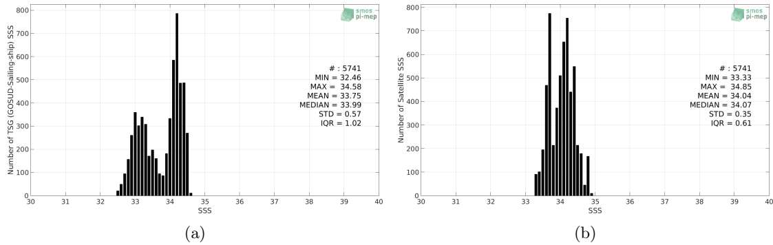
Figure 2: Histograms of SSS from TSG (GOSUD-Sailing-ship) (a) and SMOS SSS L3 v2 - Monthly - 0.25 Deg (CATDS-CECOS-IFREMER) (b) considering all match-up pairs per bins of 0.1 over the SPURS 2 Pi-MEP region and for the full satellite product period.
