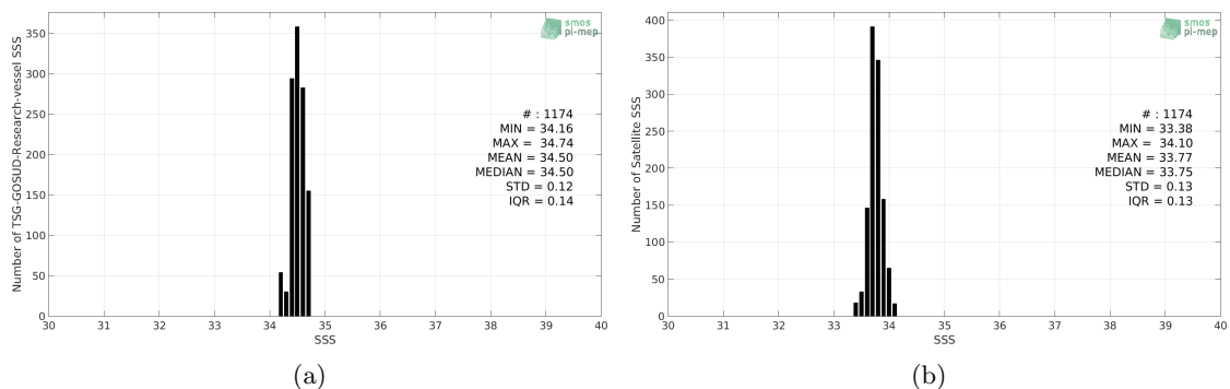
Figure 2: Histograms of SSS from TSG-GOSUD-Research-vessel (a) and SMOS-L3-CATDS-IFREMER-CECOS-V2-MONTHLY-0.25DEG (b) considering all match-up pairs per bins of 0.1 over the SPURS 2 Pi-MEP region and for the full satellite product period.
