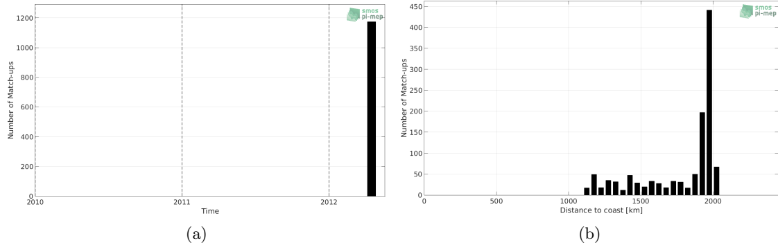
Figure 1: Number of match-ups between TSG-GOSUD-Research-vessel and SMOS-L3-CATDS-IFREMER-CECOS-V2-MONTHLY-0.25DEG SSS as a function of time (a) and as function of the distance to coast (b) over the SPURS 2 Pi-MEP region and for the full satellite product period.
