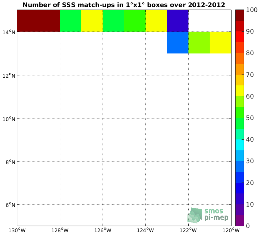
Figure 4: Number of SSS match-ups between TSG-GOSUD-Research-vessel SSS and the SMOS-L3-CATDS-IFREMER-CECOS-V2-MONTHLY-0.25DEG SSS product for the SPURS 2 Pi-MEP region over 1°x1° boxes and for the full satellite product period.
