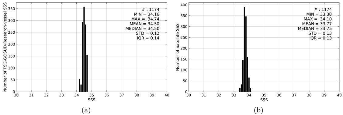
Figure 2: Histograms of SSS from TSG-GOSUD-Research-vessel (a) and SMOS-L3-CATDS-IFREMER-CECOS-V2-MONTHLY-0.25DEG (b) considering all match-up pairs per bins of 0.1 over the SPURS 2 Pi-MEP region and for the full satellite product period.
