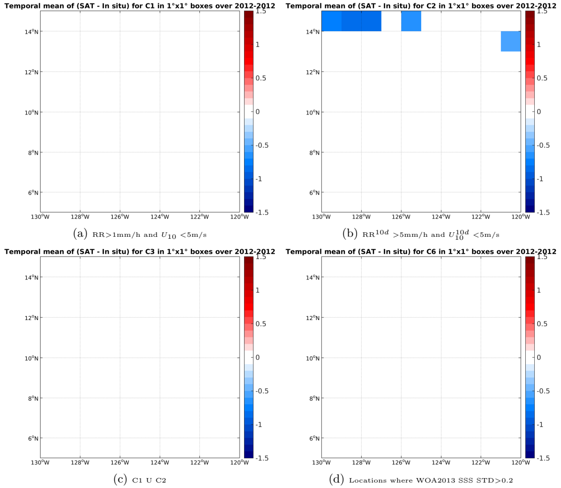
Figure 12: Temporal mean gridded over spatial boxes of size 1°x1° of \Delta SSS (SMOS-L3-CATDS-IFREMER-CECOS-V2-MONTHLY-0.25DEG - TSG-GOSUD-Research-vessel) for 4 different subdatasets corresponding to: RR > 1mm/h and U_{10} < 5\text{m/s} (a), RR^{10d} > 5\text{mm/h} and U_{10}^{10d} < 5\text{m/s} (b), C1 U C2 (c), Locations where WOA2013 SSS STD > 0.2 (d).
