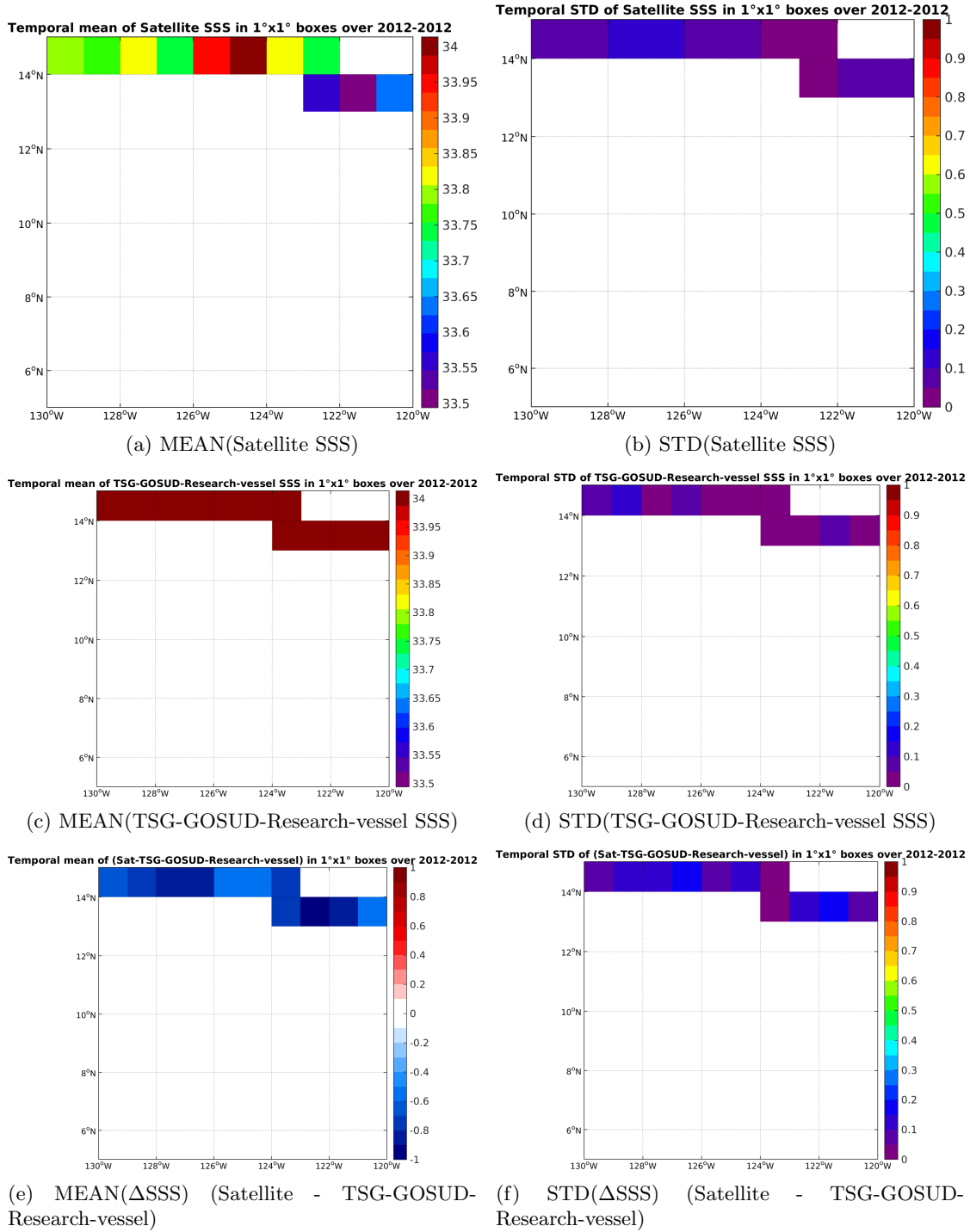
Figure 6: Temporal mean (left) and STD (right) of SSS from SMOS-L3-CATDS-IFREMER-CECOS-V2-MONTHLY-0.25DEG (top), TSG-GOSUD-Research-vessel (middle), and of \Delta SSS (Satellite - TSG-GOSUD-Research-vessel). Only match-up pairs are used to generate these maps.
