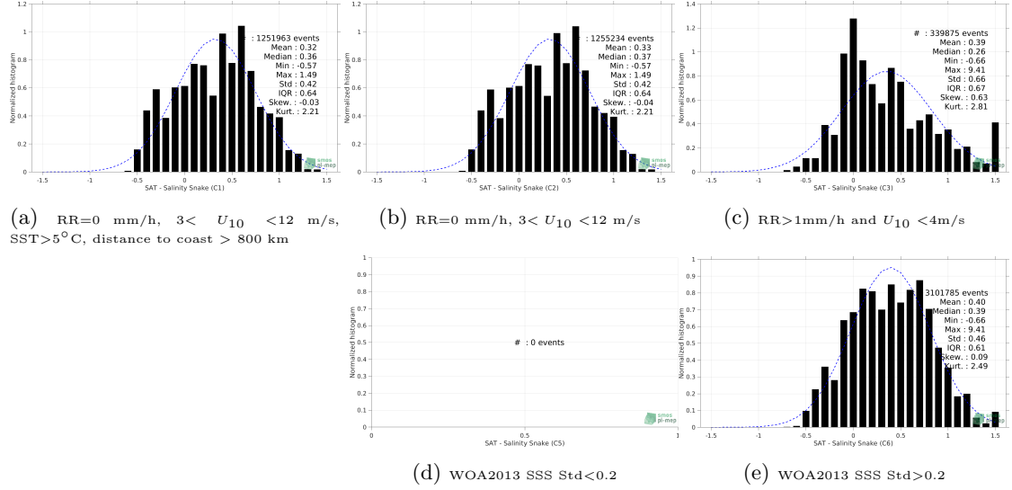
Figure 12: Normalized histogram of \Delta SSS (SMOS SSS L3 v2 - Monthly - 0.25 Deg (CATDS-CECOS-IFREMER) - Salinity Snake) for 5 different subdatasets corresponding to: RR=0 mm/h, 3 < U_{10} < 12 m/s, SST > 5°C, distance to coast > 800 km (a), RR=0 mm/h, 3 < U_{10} < 12 m/s (b), RR > 1mm/h and U_{10} < 4 m/s (c), WOA2013 SSS Std < 0.2 (d), WOA2013 SSS Std > 0.2 (e).
