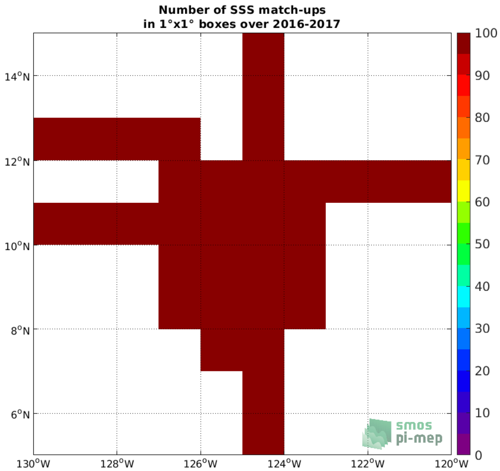
Figure 3: Number of SSS match-ups between Salinity Snake SSS and the SMOS SSS L3 v2 - Monthly - 0.25 Deg (CATDS-CECOS-IFREMER) SSS product for the SPURS 2 Pi-MEP region over 1°x1° boxes and for the full satellite product period.
