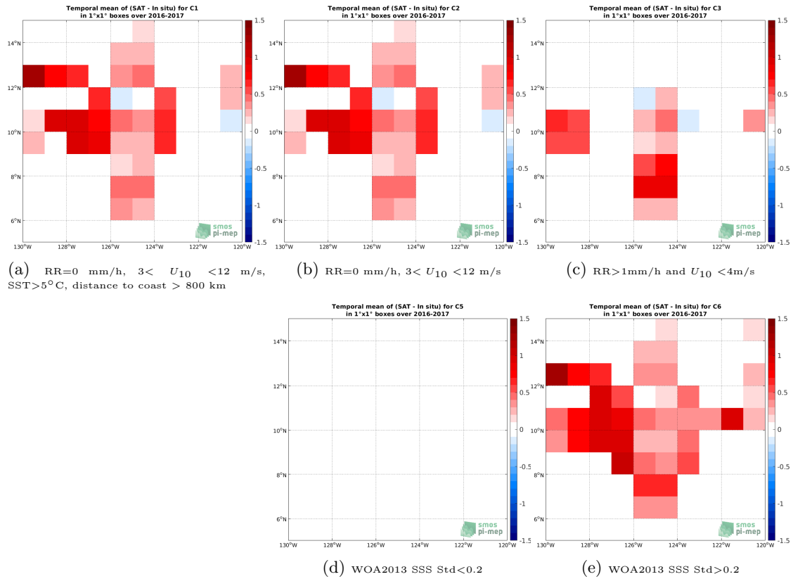
Figure 11: Temporal mean gridded over spatial boxes of size 1^{\circ}\times 1^{\circ} of \Delta\text{SSS} (SMOS SSS L3 v2 - Monthly - 0.25 Deg (CATDS-CECOS-IFREMER) - Salinity Snake) for 5 different subdatasets corresponding to:RR=0 mm/h, 3 < U_{10} < 12 m/s, SST >5^{\circ}\text{C} , distance to coast > 800 km (a), RR=0 mm/h, 3 < U_{10} < 12 m/s (b), RR >1 mm/h and U_{10} < 4 m/s (c), WOA2013 SSS Std <0.2 (d), WOA2013 SSS Std >0.2 (e).
