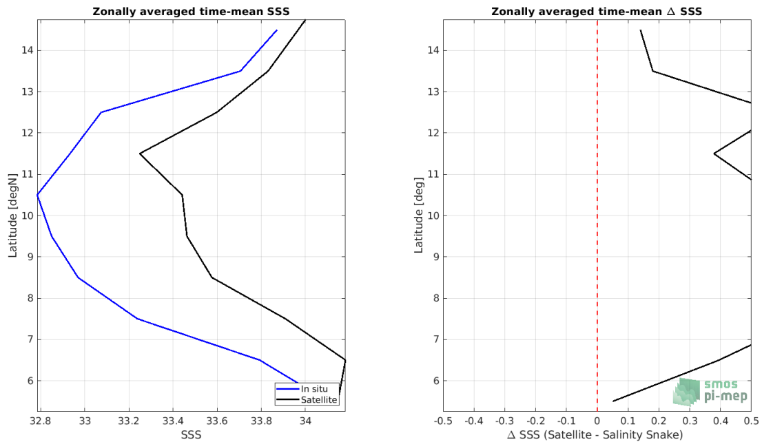
Figure 7: Left panel: Zonal mean SSS from SMOS SSS L3 v2 - Monthly - 0.25 Deg (CATDS-CECOS-IFREMER) satellite product (black) and from Salinity Snake (blue). Right panel: Zonal mean of \Delta SSS (Satellite - Salinity Snake) for all the collected Pi-MEP match-up pairs estimated over the full satellite product period.
