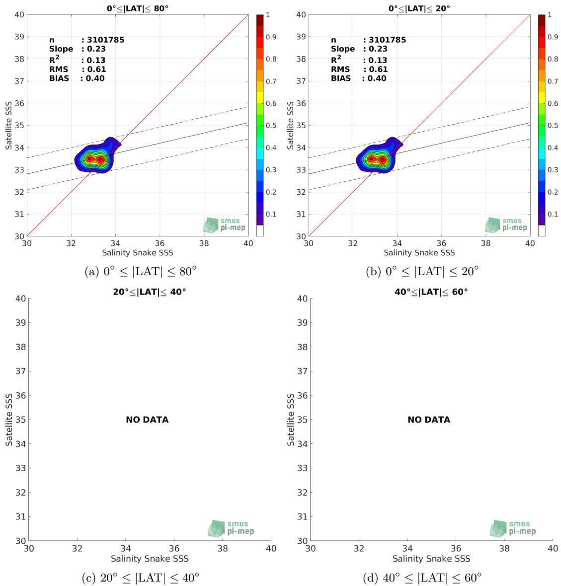
Figure 8: Contour maps of the concentration of SMOS SSS L3 v2 - Monthly - 0.25 Deg (CATDS-CECOS-IFREMER) SSS (y-axis) versus Salinity Snake SSS (x-axis) at match-up pairs for different latitude bands. For each plot, the red line shows x=y . The black thin and dashed lines indicate a linear fit through the data cloud and the \pm 95\% confidence levels, respectively. The number match-up pairs n , the slope and R^2 coefficient of the linear fit, the root mean square (RMS) and the mean bias between satellite and in situ data are indicated for each latitude band in each plots.
