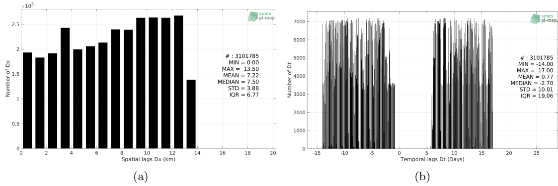
Figure 4: Histograms of the spatial (a) and temporal (b) lags between the location/time of the Salinity Snake measurement and the date of the corresponding SMOS SSS L3 v2 - Monthly - 0.25 Deg (CATDS-CECOS-IFREMER) SSS pixel.
