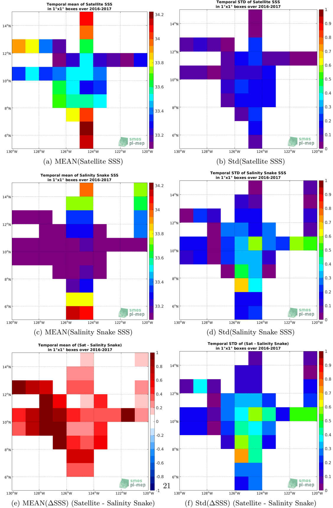
Figure 5: Temporal mean (left) and Std (right) of SSS from SMOS SSS L3 v2 - Monthly - 0.25 Deg (CATDS-CECOS-IFREMER) (top), Salinity Snake (middle), and of \Delta SSS (Satellite - Salinity Snake). Only match-up pairs are used to generate these maps.
