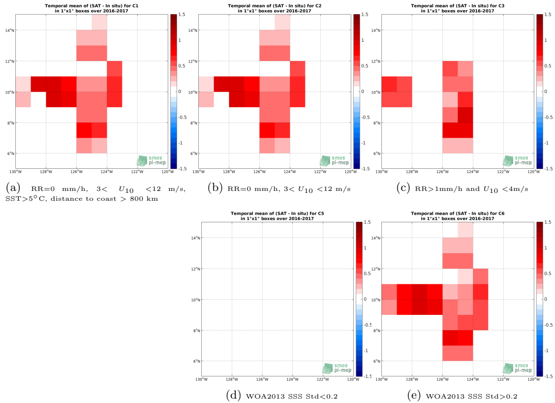
Figure 12: Temporal mean gridded over spatial boxes of size 1^{\circ}\times 1^{\circ} of \Delta\text{SSS} (SMOS SSS L3 v2 - Monthly - 0.25 Deg (CATDS-CECOS-IFREMER) - Salinity Snake) for 5 different subdatasets corresponding to:RR=0 mm/h, 3 < U_{10} < 12 m/s, SST >5^{\circ}\text{C} , distance to coast > 800 km (a), RR=0 mm/h, 3 < U_{10} < 12 m/s (b), RR >1 mm/h and U_{10} < 4 m/s (c), WOA2013 SSS Std <0.2 (d), WOA2013 SSS Std >0.2 (e).
