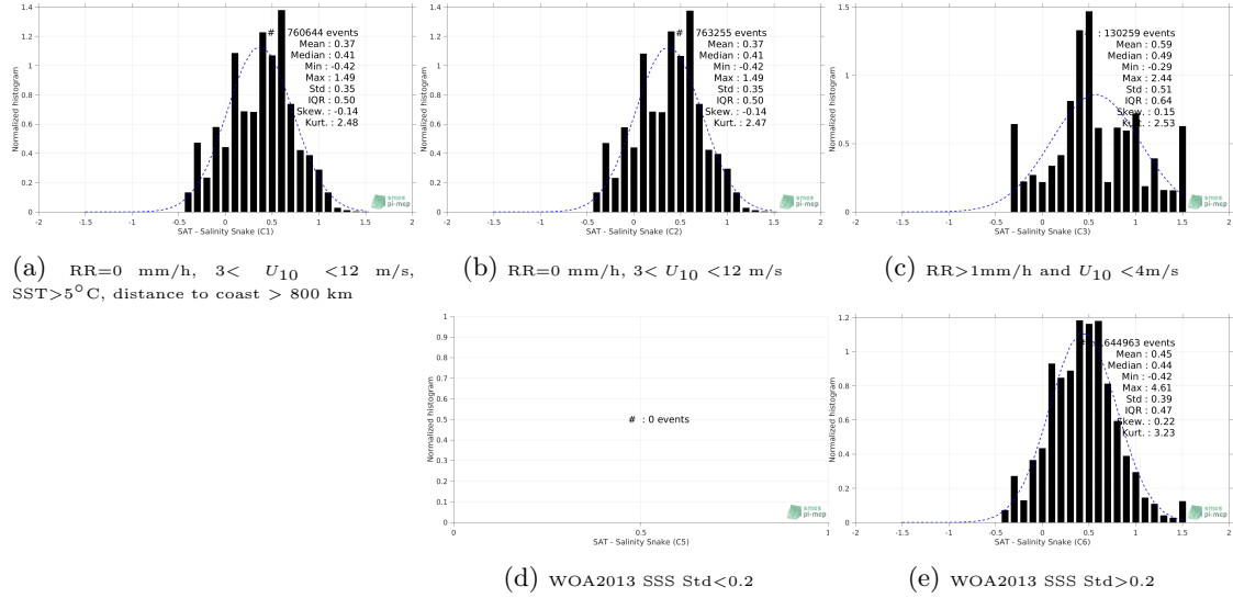
Figure 13: Normalized histogram of \Delta SSS (SMOS SSS L3 v2 - Monthly - 0.25 Deg (CATDS-CECOS-IFREMER) - Salinity Snake) for 5 different subdatasets corresponding to: RR=0 mm/h, 3 < U_{10} < 12 m/s, SST>5°C, distance to coast > 800 km (a), RR=0 mm/h, 3 < U_{10} < 12 m/s (b), RR>1mm/h and U_{10} < 4 m/s (c), WOA2013 SSS Std<0.2 (d), WOA2013 SSS Std>0.2 (e).
