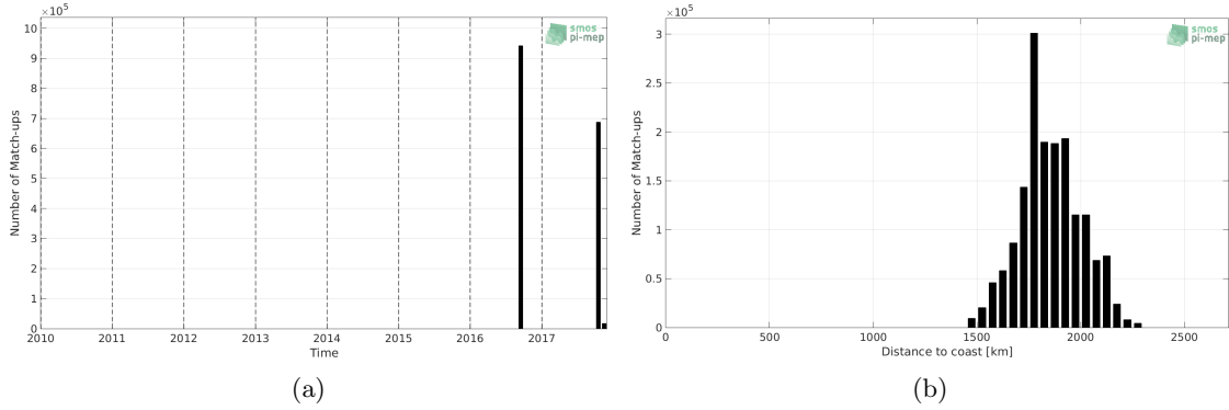
Figure 1: Number of match-ups between Salinity Snake and SMOS SSS L3 v2 - Monthly - 0.25 Deg (CATDS-CECOS-IFREMER) SSS as a function of time (a) and as function of the distance to coast (b) over the SPURS 2 Pi-MEP region and for the full satellite product period.
