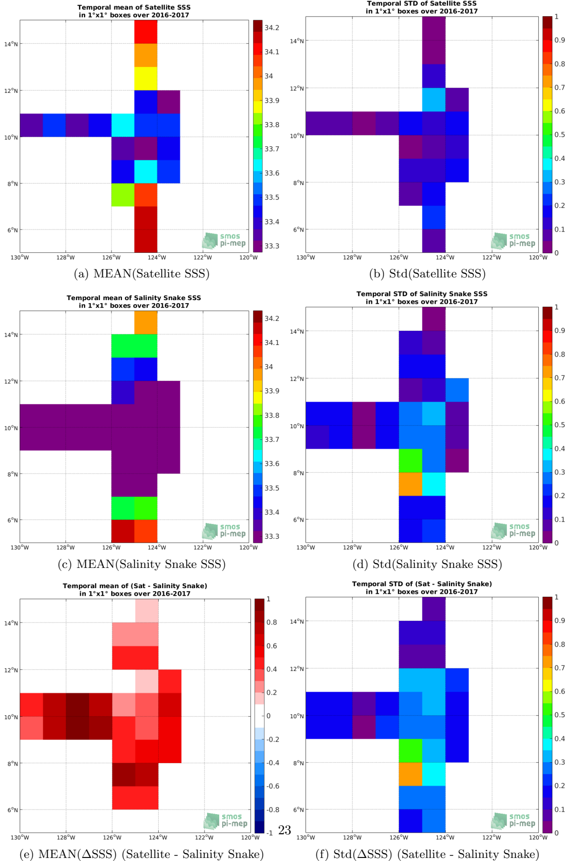
Figure 6: Temporal mean (left) and Std (right) of SSS from SMOS SSS L3 v2 - Monthly - 0.25 Deg (CATDS-CECOS-IFREMER) (top), Salinity Snake (middle), and of \Delta SSS (Satellite - Salinity Snake). Only match-up pairs are used to generate these maps.
