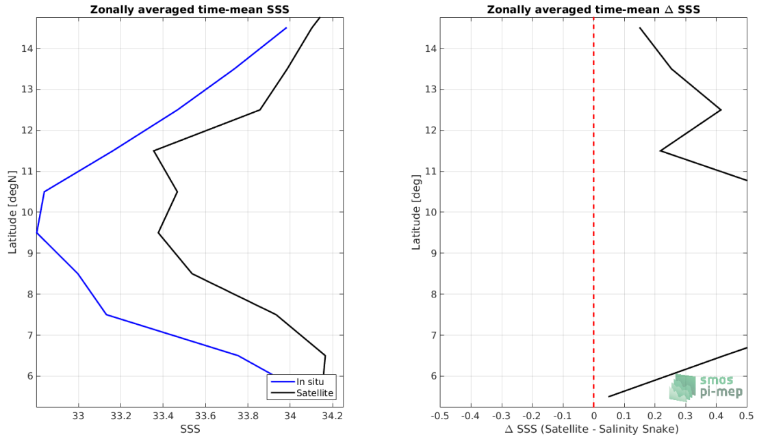
Figure 8: Left panel: Zonal mean SSS from SMOS SSS L3 v2 - Monthly - 0.25 Deg (CATDS-CECOS-IFREMER) satellite product (black) and from Salinity Snake (blue). Right panel: Zonal mean of \Delta SSS (Satellite - Salinity Snake) for all the collected Pi-MEP match-up pairs estimated over the full satellite product period.
