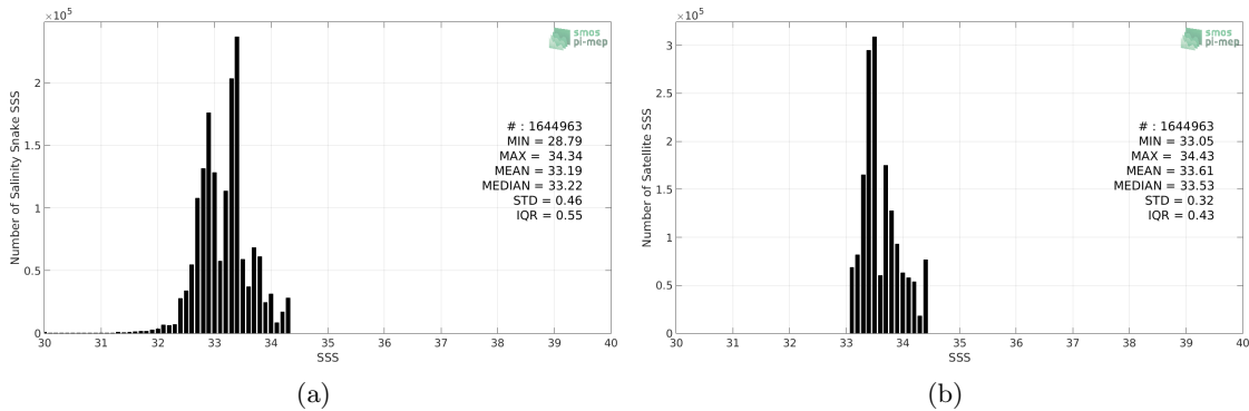
Figure 2: Histograms of SSS from Salinity Snake (a) and SMOS SSS L3 v2 - Monthly - 0.25 Deg (CATDS-CECOS-IFREMER) (b) considering all match-up pairs per bins of 0.1 over the SPURS 2 Pi-MEP region and for the full satellite product period.
