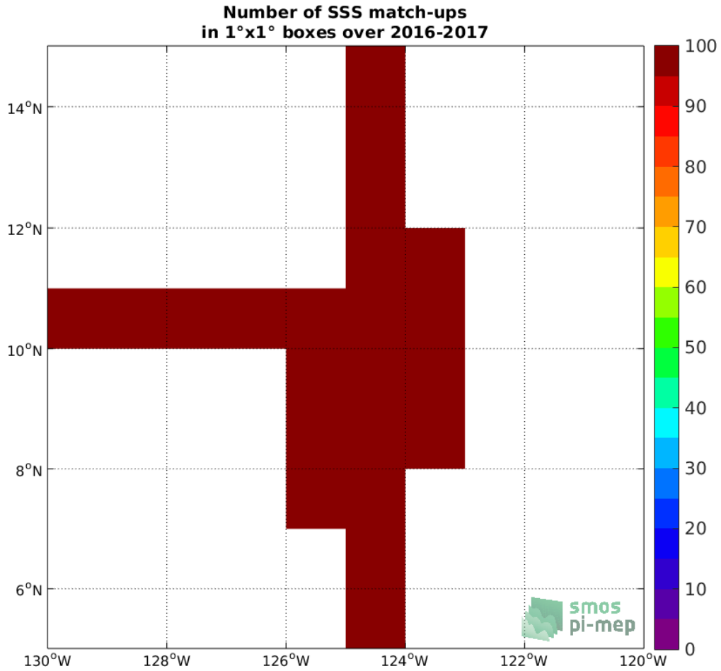
Figure 4: Number of SSS match-ups between Salinity Snake SSS and the SMOS SSS L3 v2 - Monthly - 0.25 Deg (CATDS-CECOS-IFREMER) SSS product for the SPURS 2 Pi-MEP region over 1°x1° boxes and for the full satellite product period.
