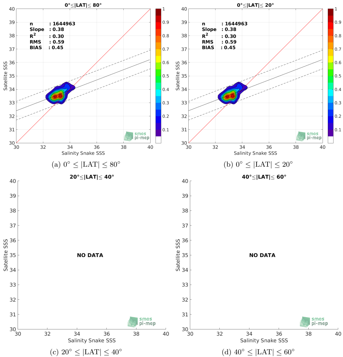
Figure 9: Contour maps of the concentration of SMOS SSS L3 v2 - Monthly - 0.25 Deg (CATDS-CECOS-IFREMER) SSS (y-axis) versus Salinity Snake SSS (x-axis) at match-up pairs for different latitude bands. For each plot, the red line shows x=y . The black thin and dashed lines indicate a linear fit through the data cloud and the \pm 95\% confidence levels, respectively. The number match-up pairs n , the slope and R^2 coefficient of the linear fit, the root mean square (RMS) and the mean bias between satellite and in situ data are indicated for each latitude band in each plots.
