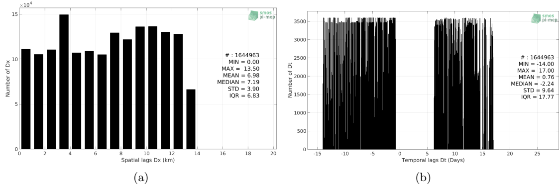
Figure 5: Histograms of the spatial (a) and temporal (b) lags between the time of the Salinity Snake measurements and the date of the corresponding SMOS SSS L3 v2 - Monthly - 0.25 Deg (CATDS-CECOS-IFREMER) SSS product.
