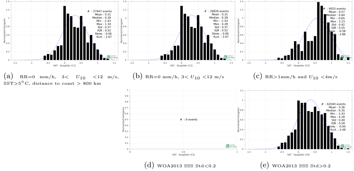
Figure 12: Normalized histogram of \Delta SSS (SMOS SSS L3 v2 - Monthly - 0.25 Deg (CATDS-CECOS-IFREMER) - Seaglider) for 5 different subdatasets corresponding to: RR=0 mm/h, 3 < U_{10} < 12 m/s, SST > 5°C, distance to coast > 800 km (a), RR=0 mm/h, 3 < U_{10} < 12 m/s (b), RR > 1mm/h and U_{10} < 4 m/s (c), WOA2013 SSS Std < 0.2 (d), WOA2013 SSS Std > 0.2 (e).
