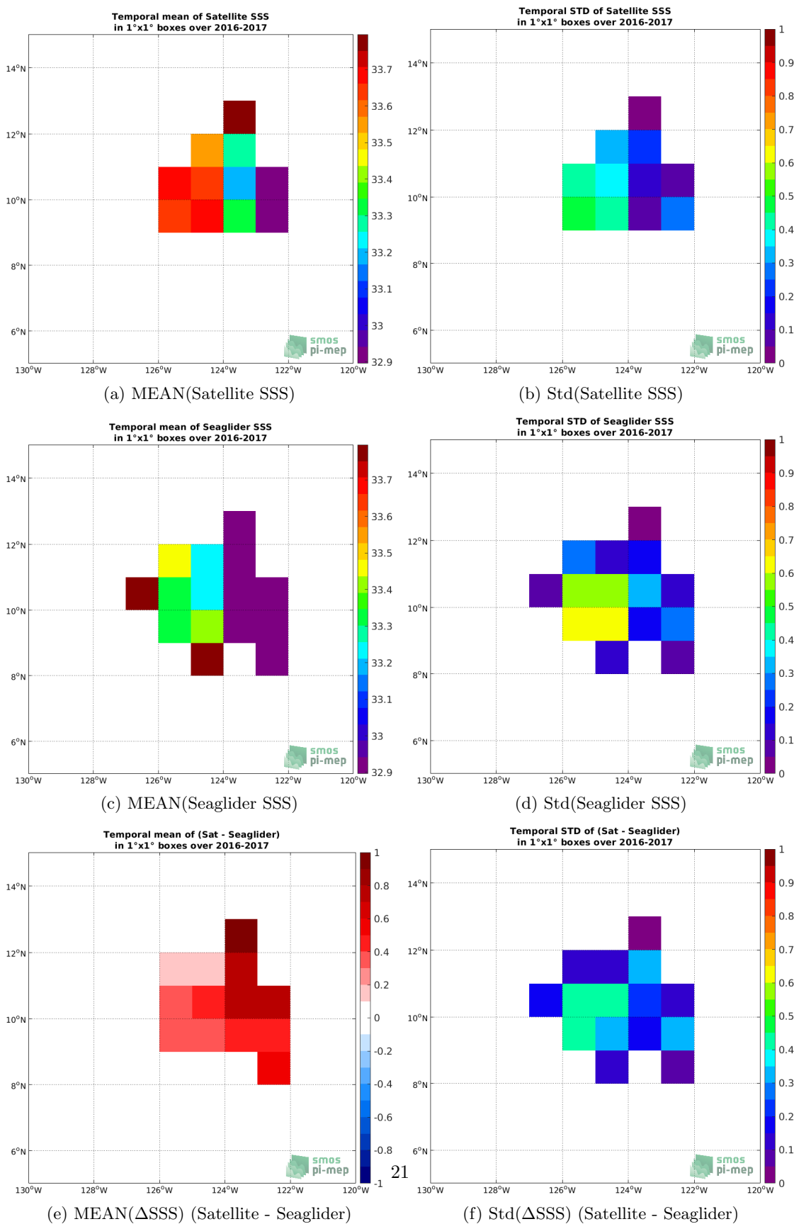
Figure 5: Temporal mean (left) and Std (right) of SSS from SMOS SSS L3 v2 - Monthly - 0.25 Deg (CATDS-CECOS-IFREMER) (top), Seaglider (middle), and of \Delta SSS (Satellite - Seaglider). Only match-up pairs are used to generate these maps.
