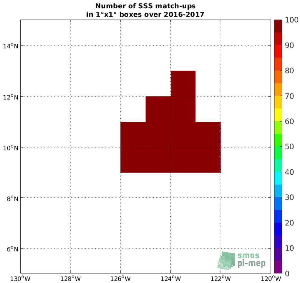
Figure 3: Number of SSS match-ups between Seaglider SSS and the SMOS SSS L3 v2 - Monthly - 0.25 Deg (CATDS-CECOS-IFREMER) SSS product for the SPURS 2 Pi-MEP region over 1°x1° boxes and for the full satellite product period.
