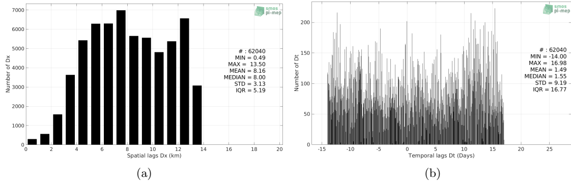
Figure 4: Histograms of the spatial (a) and temporal (b) lags between the location/time of the Seaglider measurement and the date of the corresponding SMOS SSS L3 v2 - Monthly - 0.25 Deg (CATDS-CECOS-IFREMER) SSS pixel.
