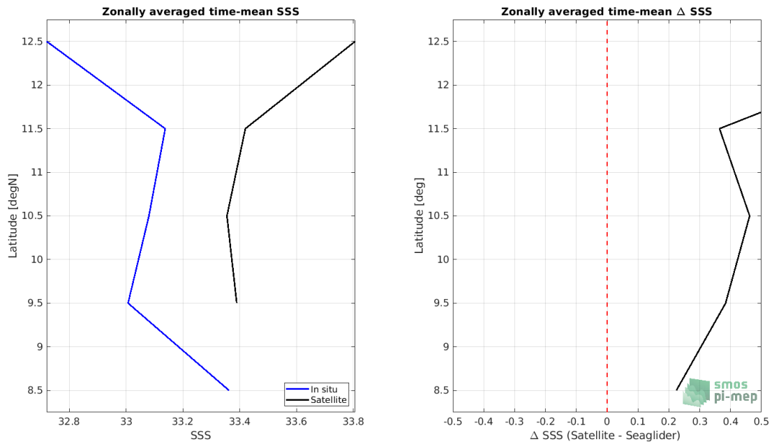
Figure 7: Left panel: Zonal mean SSS from SMOS SSS L3 v2 - Monthly - 0.25 Deg (CATDS-CECOS-IFREMER) satellite product (black) and from Seaglider (blue). Right panel: Zonal mean of \Delta SSS (Satellite - Seaglider) for all the collected Pi-MEP match-up pairs estimated over the full satellite product period.
