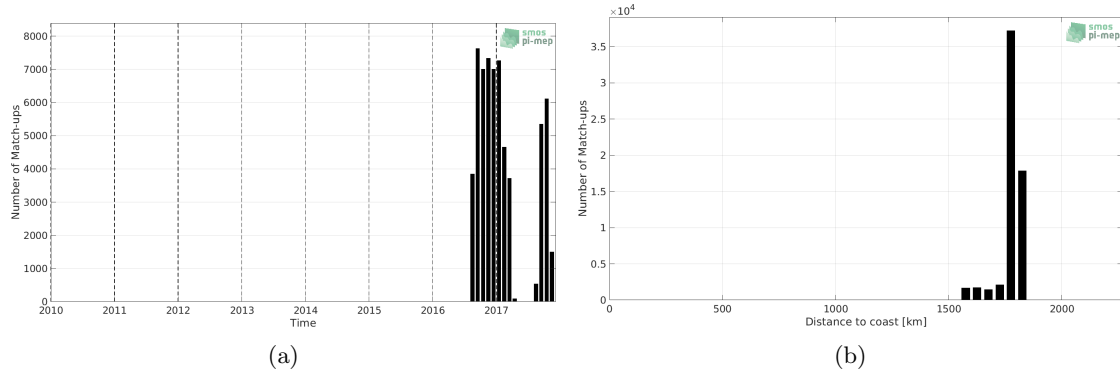
Figure 1: Number of match-ups between Seaglider and SMOS SSS L3 v2 - Monthly - 0.25 Deg (CATDS-CECOS-IFREMER) SSS as a function of time (a) and as function of the distance to coast (b) over the SPURS 2 Pi-MEP region and for the full satellite product period.
