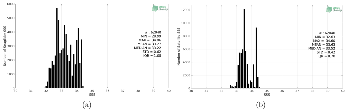
Figure 2: Histograms of SSS from Seaglider (a) and SMOS SSS L3 v2 - Monthly - 0.25 Deg (CATDS-CECOS-IFREMER) (b) considering all match-up pairs per bins of 0.1 over the SPURS 2 Pi-MEP region and for the full satellite product period.
