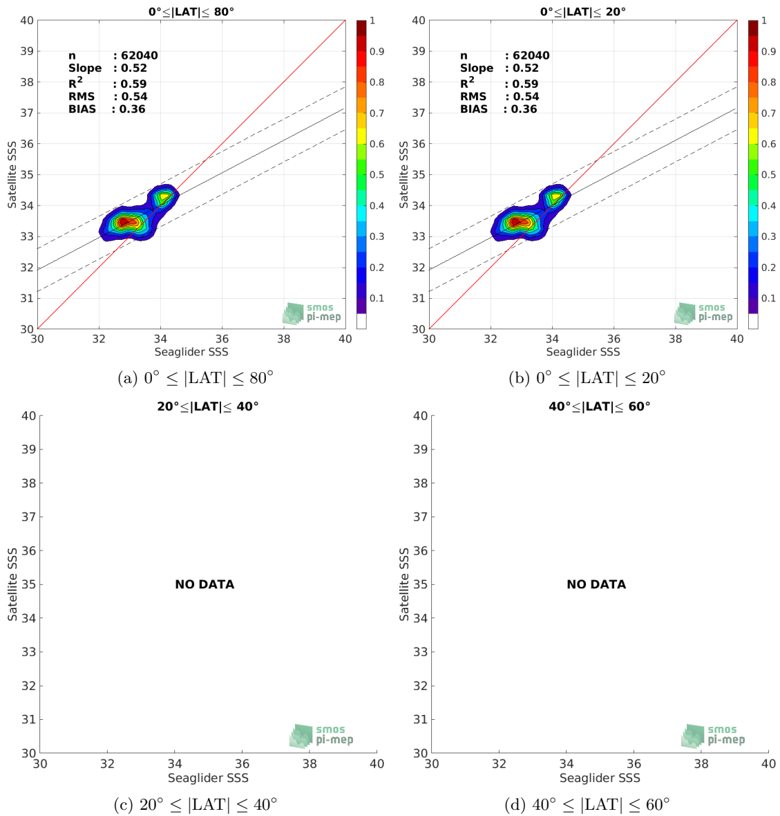
Figure 8: Contour maps of the concentration of SMOS SSS L3 v2 - Monthly - 0.25 Deg (CATDS-CECOS-IFREMER) SSS (y-axis) versus Seaglider SSS (x-axis) at match-up pairs for different latitude bands. For each plot, the red line shows x=y . The black thin and dashed lines indicate a linear fit through the data cloud and the \pm 95\% confidence levels, respectively. The number match-up pairs n , the slope and R^2 coefficient of the linear fit, the root mean square (RMS) and the mean bias between satellite and in situ data are indicated for each latitude band in each plots.
