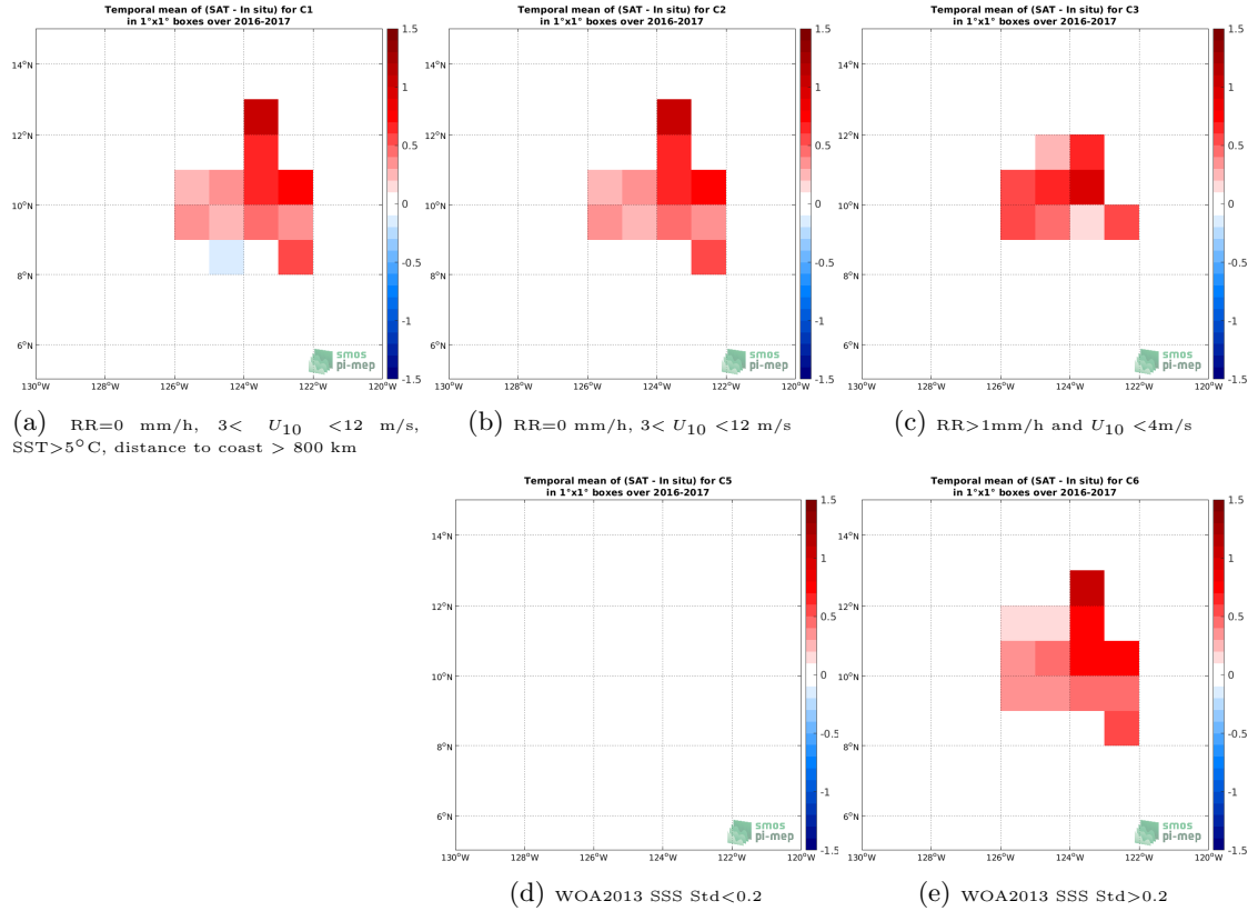
Figure 11: Temporal mean gridded over spatial boxes of size 1^{\circ}\times 1^{\circ} of \Delta\text{SSS} (SMOS SSS L3 v2 - Monthly - 0.25 Deg (CATDS-CECOS-IFREMER) - Seaglider) for 5 different subdatasets corresponding to:RR=0 mm/h, 3 < U_{10} < 12 m/s, SST >5^{\circ}\text{C} , distance to coast > 800 km (a), RR=0 mm/h, 3 < U_{10} < 12 m/s (b), RR >1 mm/h and U_{10} < 4 m/s (c), WOA2013 SSS Std <0.2 (d), WOA2013 SSS Std >0.2 (e).
