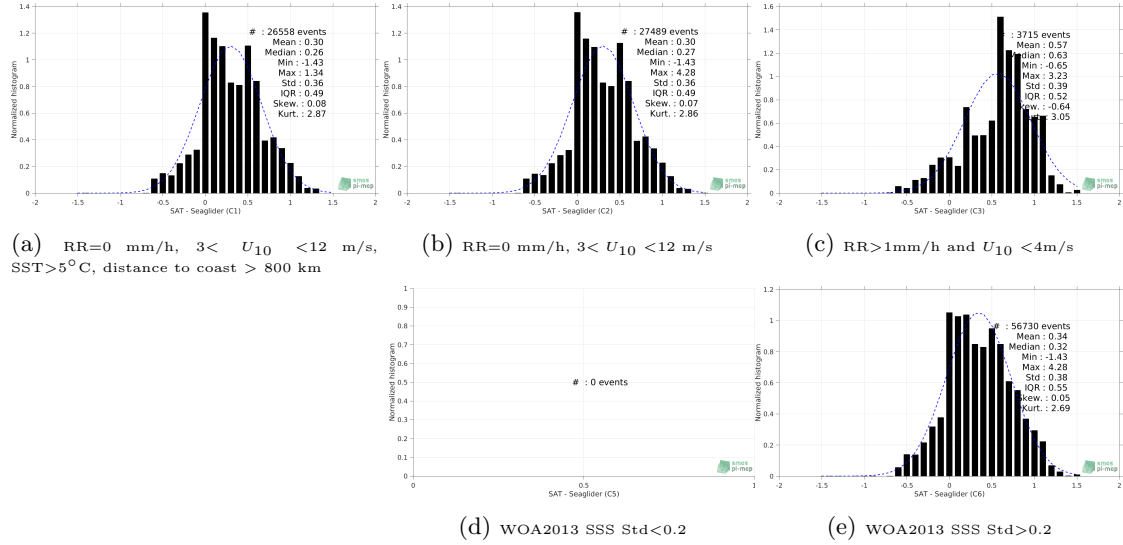
Figure 13: Normalized histogram of \Delta SSS (SMOS SSS L3 v2 - Monthly - 0.25 Deg (CATDS-CECOS-IFREMER) - Seaglider) for 5 different subdatasets corresponding to: RR=0 mm/h, 3 < U_{10} < 12 m/s, SST > 5°C, distance to coast > 800 km (a), RR=0 mm/h, 3 < U_{10} < 12 m/s (b), RR > 1mm/h and U_{10} < 4 m/s (c), WOA2013 SSS Std < 0.2 (d), WOA2013 SSS Std > 0.2 (e).
