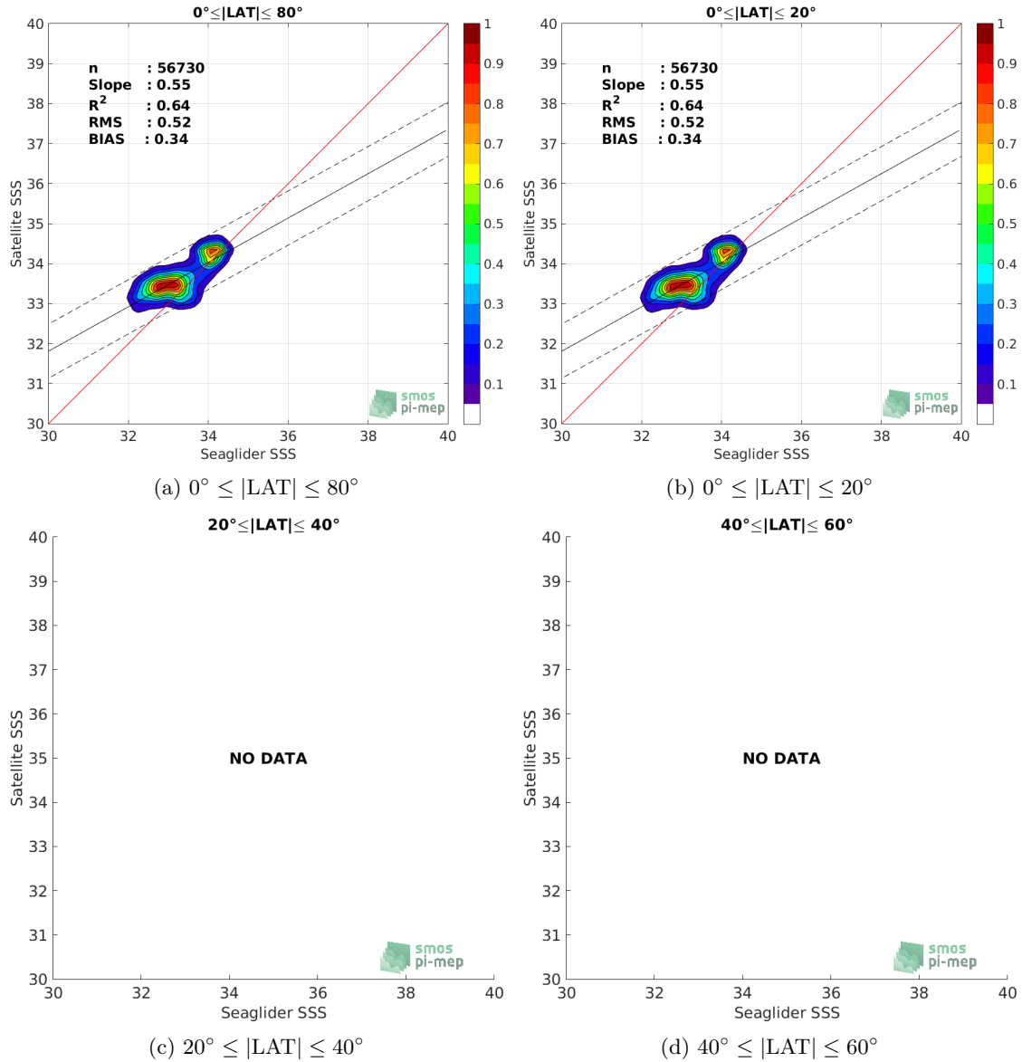
Figure 9: Contour maps of the concentration of SMOS SSS L3 v2 - Monthly - 0.25 Deg (CATDS-CECOS-IFREMER) SSS (y-axis) versus Seaglider SSS (x-axis) at match-up pairs for different latitude bands. For each plot, the red line shows x=y . The black thin and dashed lines indicate a linear fit through the data cloud and the \pm 95\% confidence levels, respectively. The number match-up pairs n , the slope and R^2 coefficient of the linear fit, the root mean square (RMS) and the mean bias between satellite and in situ data are indicated for each latitude band in each plots.
