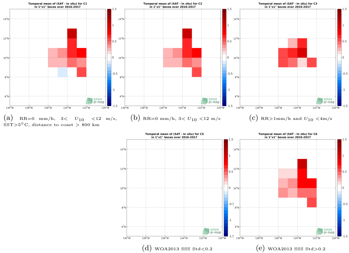
Figure 12: Temporal mean gridded over spatial boxes of size 1^{\circ}\times 1^{\circ} of \Delta\text{SSS} (SMOS SSS L3 v2 - Monthly - 0.25 Deg (CATDS-CECOS-IFREMER) - Seaglider) for 5 different subdatasets corresponding to:RR=0 mm/h, 3 < U_{10} < 12 m/s, SST >5^{\circ}\text{C} , distance to coast > 800 km (a), RR=0 mm/h, 3 < U_{10} < 12 m/s (b), RR >1 mm/h and U_{10} < 4 m/s (c), WOA2013 SSS Std <0.2 (d), WOA2013 SSS Std >0.2 (e).
