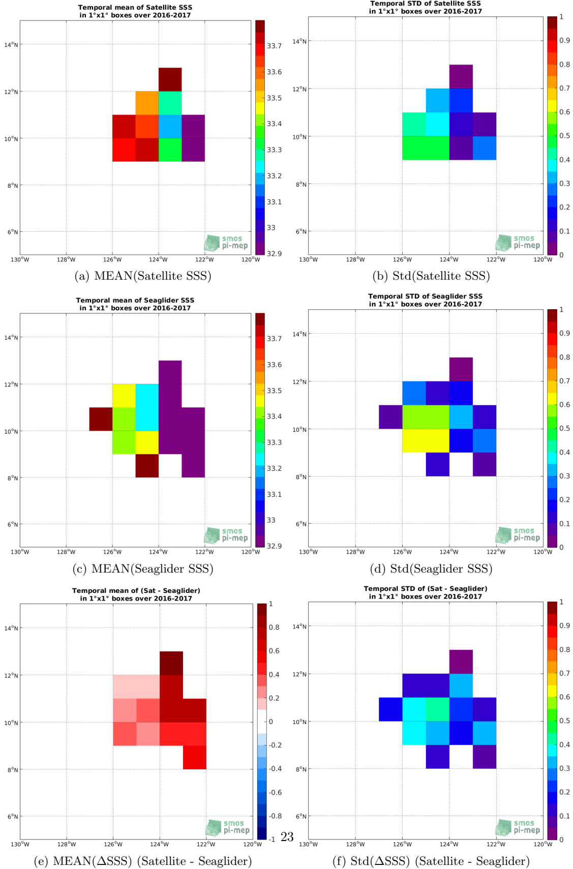
Figure 6: Temporal mean (left) and Std (right) of SSS from SMOS SSS L3 v2 - Monthly - 0.25 Deg (CATDS-CECOS-IFREMER) (top), Seaglider (middle), and of \Delta SSS (Satellite - Seaglider). Only match-up pairs are used to generate these maps.
