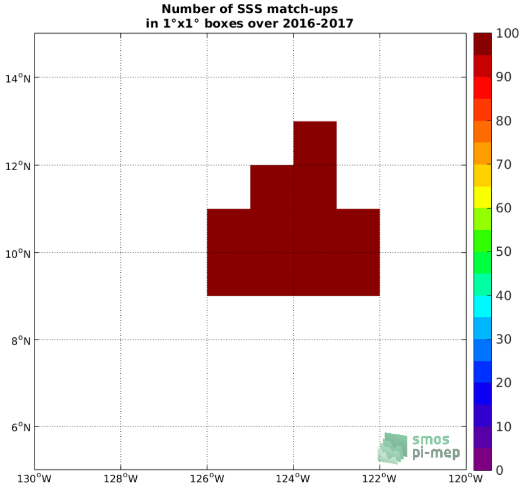
Figure 4: Number of SSS match-ups between Seagliders SSS and the SMOS SSS L3 v2 - Monthly - 0.25 Deg (CATDS-CECOS-IFREMER) SSS product for the SPURS 2 Pi-MEP region over 1°x1° boxes and for the full satellite product period.
