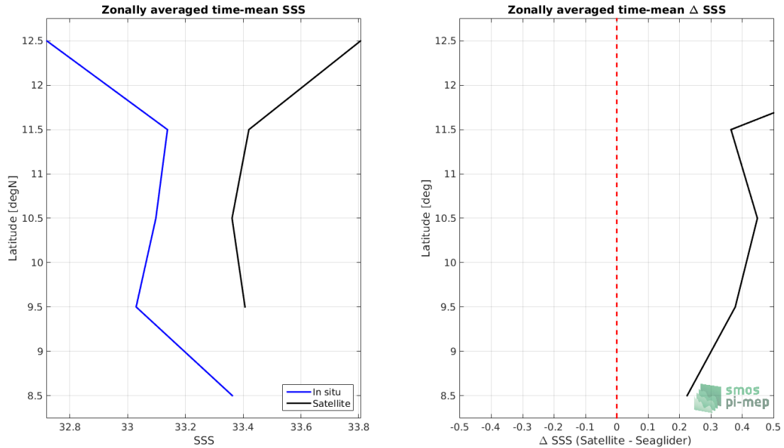
Figure 8: Left panel: Zonal mean SSS from SMOS SSS L3 v2 - Monthly - 0.25 Deg (CATDS-CECOS-IFREMER) satellite product (black) and from Seaglider (blue). Right panel: Zonal mean of \Delta SSS (Satellite - Seaglider) for all the collected Pi-MEP match-up pairs estimated over the full satellite product period.
