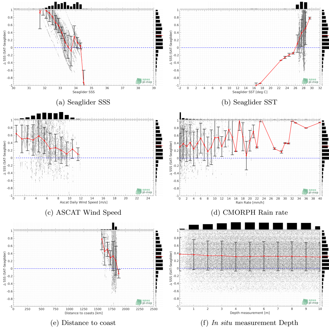
Figure 11: \Delta SSS (Satellite - Seaglider) sorted as function of Seaglider SSS a), Seaglider SST b), ASCAT Wind speed c), CMORPH rain rate d), distance to coast (e) and in situ measurement depth (f). In all plots the median and Std of \Delta SSS for each bin is indicated by the red curves and black vertical thick bars ( \pm 1 Std)
