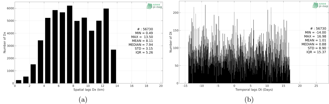
Figure 5: Histograms of the spatial (a) and temporal (b) lags between the time of the Seaglider measurements and the date of the corresponding SMOS SSS L3 v2 - Monthly - 0.25 Deg (CATDS-CECOS-IFREMER) SSS product.
