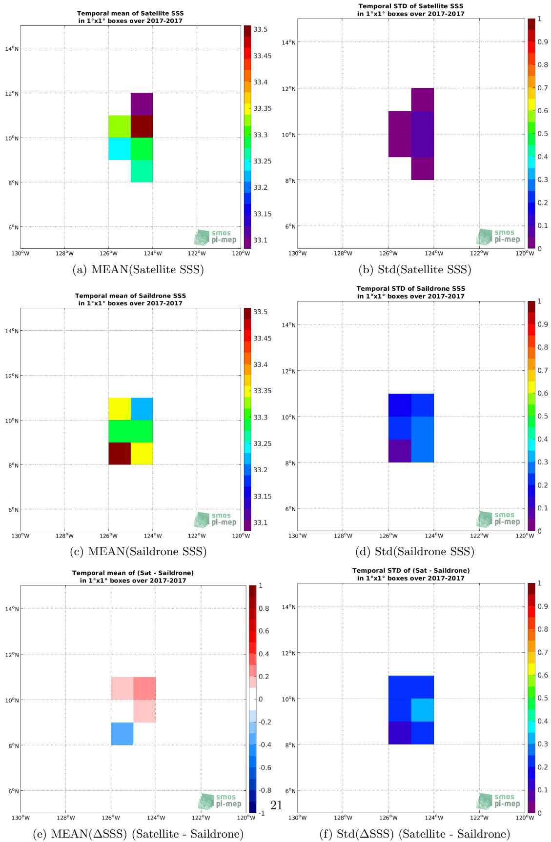
Figure 5: Temporal mean (left) and Std (right) of SSS from SMOS SSS L3 v2 - Monthly - 0.25 Deg (CATDS-CECOS-IFREMER) (top), Saildrone (middle), and of \Delta SSS (Satellite - Saildrone). Only match-up pairs are used to generate these maps.
