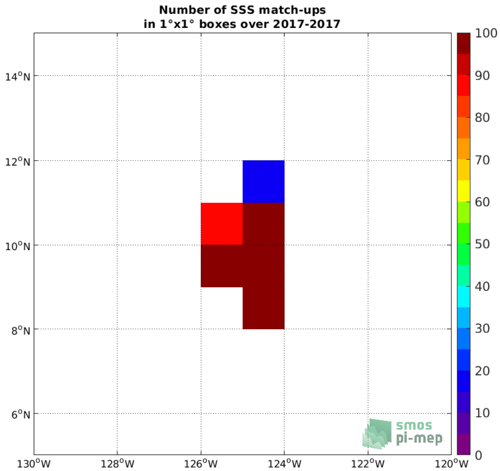
Figure 3: Number of SSS match-ups between Sairdrone SSS and the SMOS SSS L3 v2 - Monthly - 0.25 Deg (CATDS-CECOS-IFREMER) SSS product for the SPURS 2 Pi-MEP region over 1°x1° boxes and for the full satellite product period.
