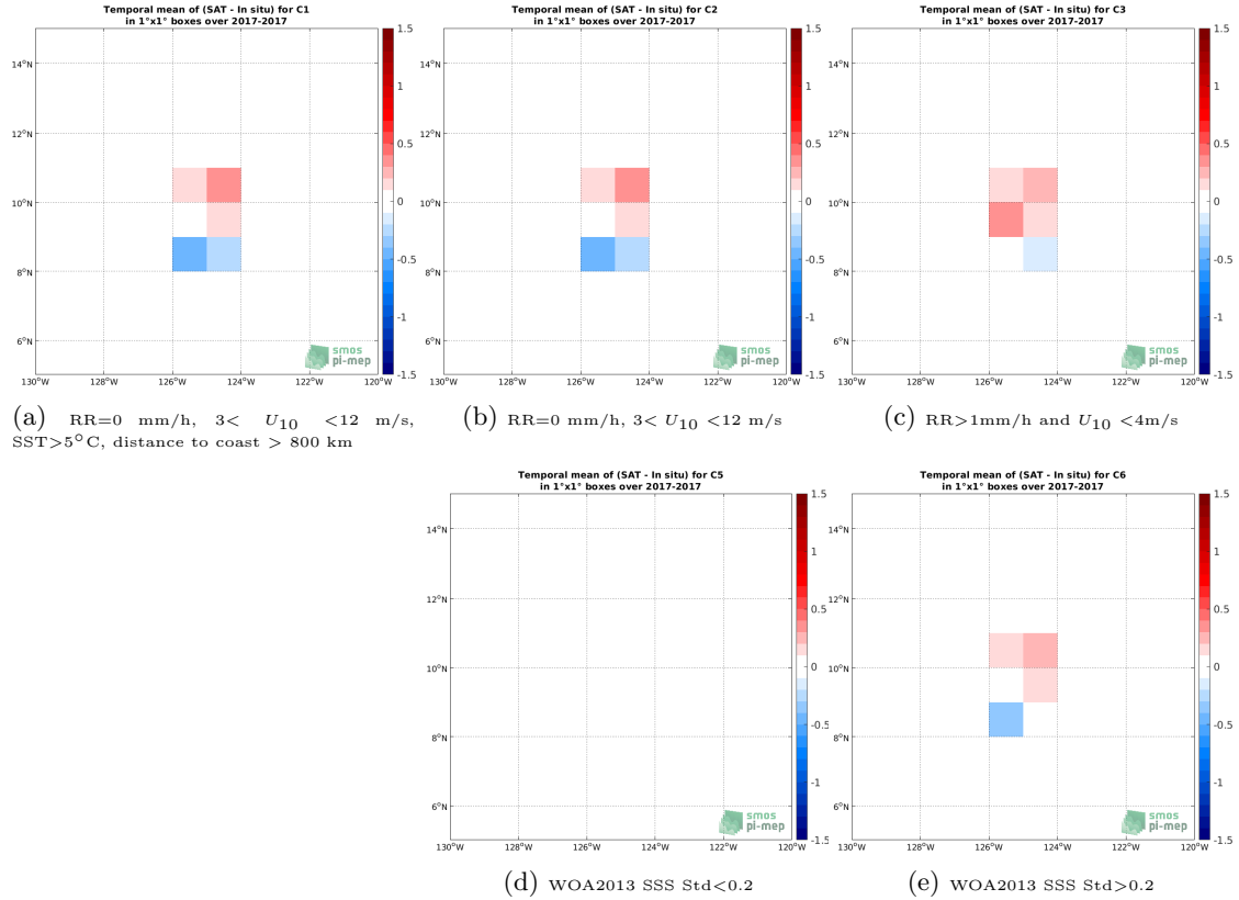
Figure 11: Temporal mean gridded over spatial boxes of size 1^{\circ}\times 1^{\circ} of \Delta\text{SSS} (SMOS SSS L3 v2 - Monthly - 0.25 Deg (CATDS-CECOS-IFREMER) - Saildrone) for 5 different subdatasets corresponding to:RR=0 mm/h, 3 < U_{10} < 12 m/s, SST >5^{\circ}\text{C} , distance to coast > 800 km (a), RR=0 mm/h, 3 < U_{10} < 12 m/s (b), RR >1 mm/h and U_{10} < 4 m/s (c), WOA2013 SSS Std <0.2 (d), WOA2013 SSS Std >0.2 (e).
