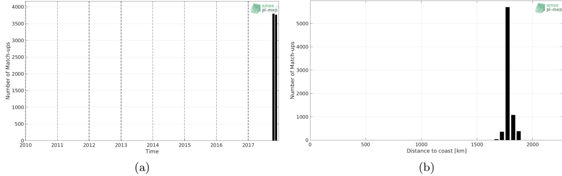
Figure 1: Number of match-ups between Saildrone and SMOS SSS L3 v2 - Monthly - 0.25 Deg (CATDS-CECOS-IFREMER) SSS as a function of time (a) and as function of the distance to coast (b) over the SPURS 2 Pi-MEP region and for the full satellite product period.
