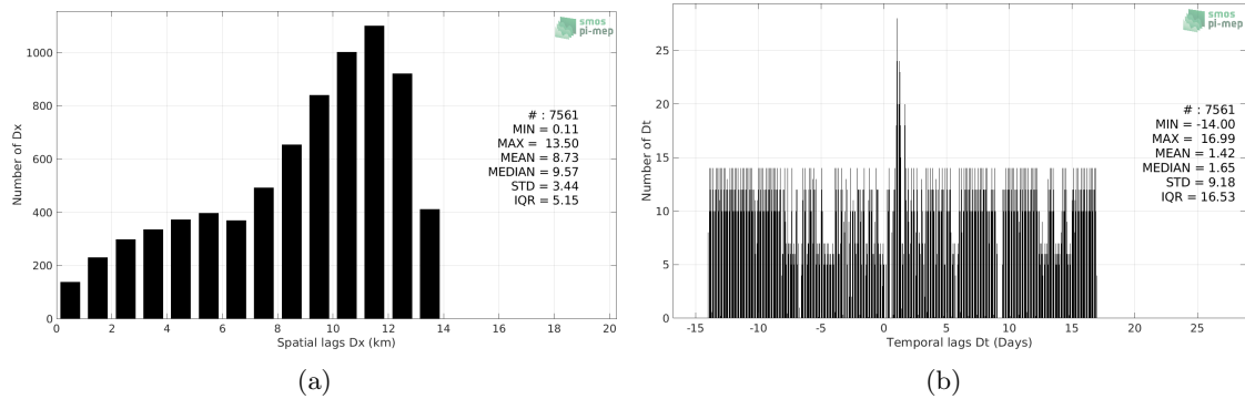
Figure 4: Histograms of the spatial (a) and temporal (b) lags between the location/time of the Saildrone measurement and the date of the corresponding SMOS SSS L3 v2 - Monthly - 0.25 Deg (CATDS-CECOS-IFREMER) SSS pixel.
