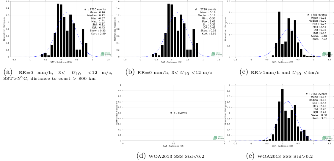
Figure 12: Normalized histogram of \Delta SSS (SMOS SSS L3 v2 - Monthly - 0.25 Deg (CATDS-CECOS-IFREMER) - Sairdrone) for 5 different subdatasets corresponding to: RR=0 mm/h, 3 < U_{10} < 12 m/s, SST > 5°C, distance to coast > 800 km (a), RR=0 mm/h, 3 < U_{10} < 12 m/s (b), RR > 1mm/h and U_{10} < 4 m/s (c), WOA2013 SSS Std < 0.2 (d), WOA2013 SSS Std > 0.2 (e).
