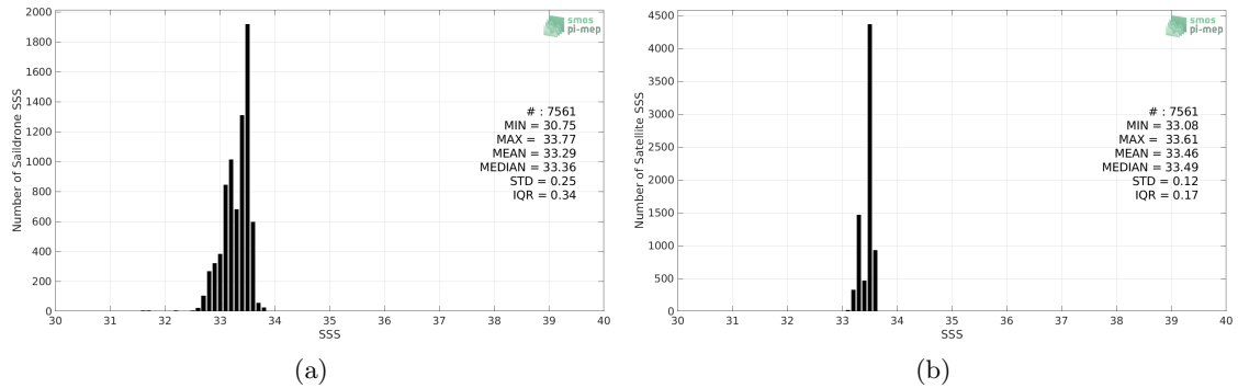
Figure 2: Histograms of SSS from Saildrone (a) and SMOS SSS L3 v2 - Monthly - 0.25 Deg (CATDS-CECOS-IFREMER) (b) considering all match-up pairs per bins of 0.1 over the SPURS 2 Pi-MEP region and for the full satellite product period.
