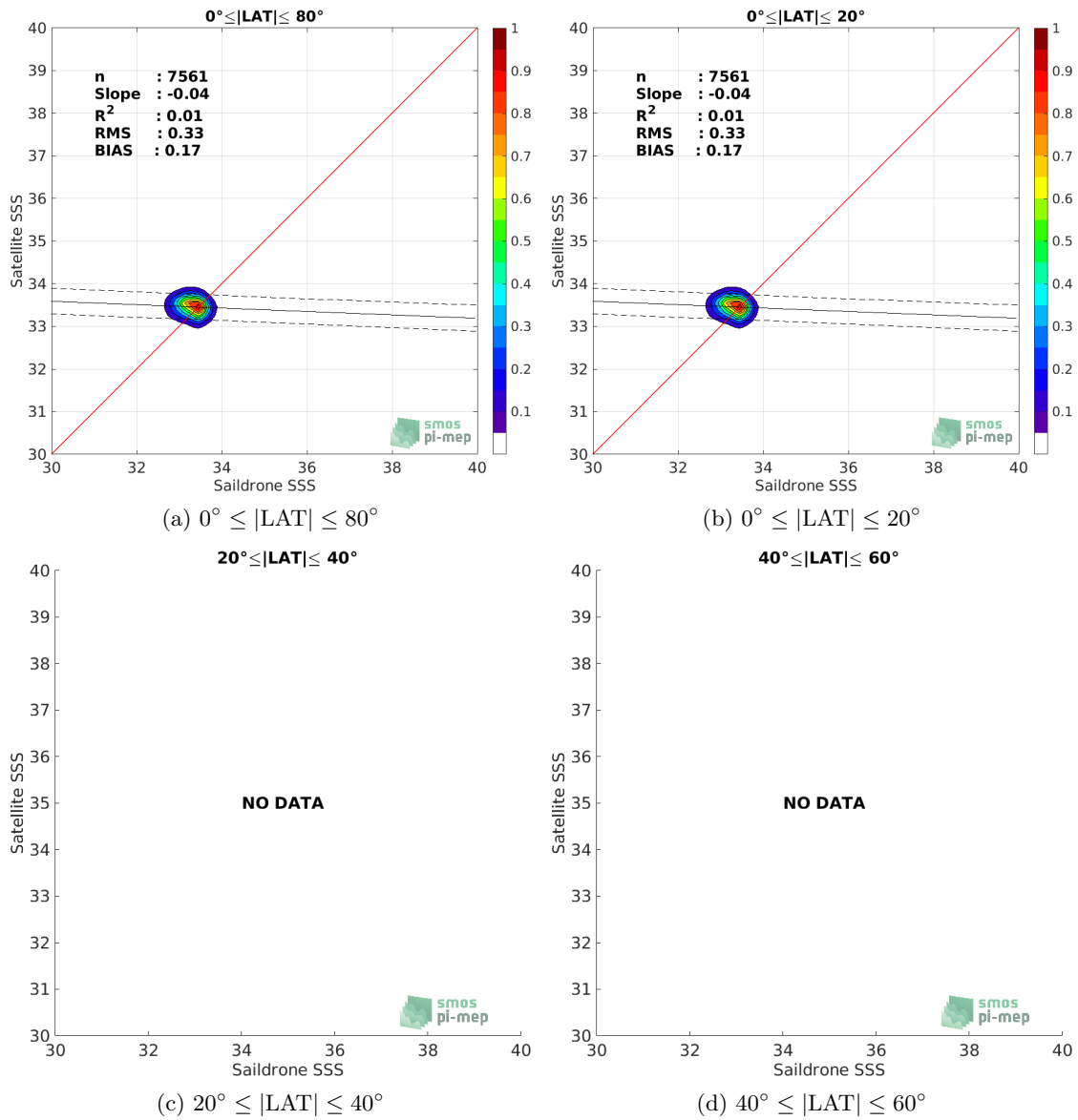
Figure 8: Contour maps of the concentration of SMOS SSS L3 v2 - Monthly - 0.25 Deg (CATDS-CECOS-IFREMER) SSS (y-axis) versus Saildrone SSS (x-axis) at match-up pairs for different latitude bands. For each plot, the red line shows x=y . The black thin and dashed lines indicate a linear fit through the data cloud and the \pm 95\% confidence levels, respectively. The number match-up pairs n , the slope and R^2 coefficient of the linear fit, the root mean square (RMS) and the mean bias between satellite and in situ data are indicated for each latitude band in each plots.
