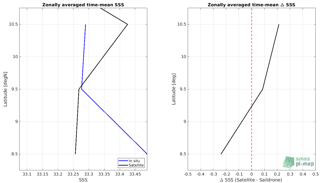
Figure 7: Left panel: Zonal mean SSS from SMOS SSS L3 v2 - Monthly - 0.25 Deg (CATDS-CECOS-IFREMER) satellite product (black) and from Sairdron (blue). Right panel: Zonal mean of \Delta SSS (Satellite - Sairdron) for all the collected Pi-MEP match-up pairs estimated over the full satellite product period.
