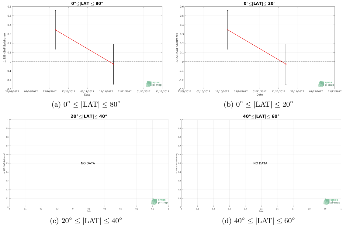
Figure 9: Monthly median (red curves) of \Delta SSS (Satellite - Sairdrone) and \pm 1 Std (black vertical thick bars) as function of time for all the collected Pi-MEP match-up pairs estimated over the SPURS 2 Pi-MEP region and for the full satellite product period are shown for different latitude bands: (a) 80^\circ\text{S}-80^\circ\text{N} , (b) 20^\circ\text{S}-20^\circ\text{N} , (c) 40^\circ\text{S}-20^\circ\text{S} and 20^\circ\text{N}-40^\circ\text{N} and (d) 60^\circ\text{S}-40^\circ\text{S} and 40^\circ\text{N}-60^\circ\text{N} .
