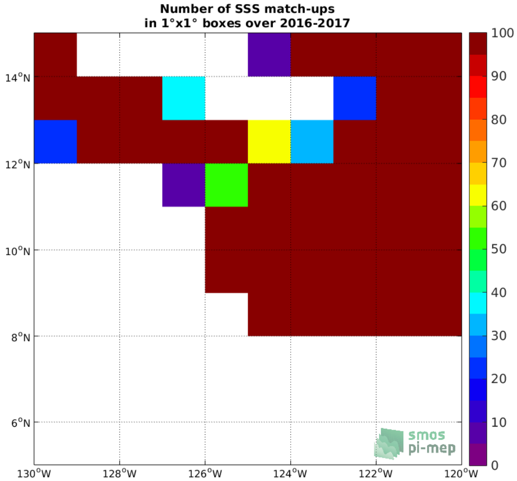
Figure 3: Number of SSS match-ups between Surface drifters SSS and the SMOS SSS L3 v2 - Monthly - 0.25 Deg (CATDS-CECOS-IFREMER) SSS product for the SPURS 2 Pi-MEP region over 1°x1° boxes and for the full satellite product period.
