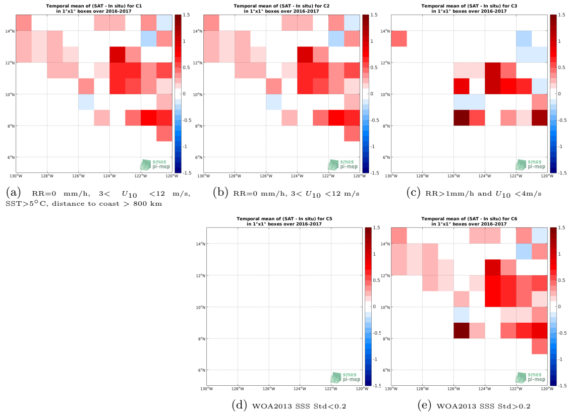
Figure 11: Temporal mean gridded over spatial boxes of size 1^{\circ}\times 1^{\circ} of \Delta\text{SSS} (SMOS SSS L3 v2 - Monthly - 0.25 Deg (CATDS-CECOS-IFREMER) - Surface drifters) for 5 different subdatasets corresponding to:RR=0 mm/h, 3 < U_{10} < 12 m/s, SST >5^{\circ}\text{C} , distance to coast > 800 km (a), RR=0 mm/h, 3 < U_{10} < 12 m/s (b), RR >1 mm/h and U_{10} < 4 m/s (c), WOA2013 SSS Std <0.2 (d), WOA2013 SSS Std >0.2 (e).
