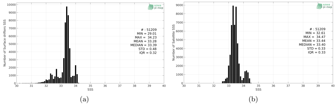
Figure 2: Histograms of SSS from Surface drifters (a) and SMOS SSS L3 v2 - Monthly - 0.25 Deg (CATDS-CECOS-IFREMER) (b) considering all match-up pairs per bins of 0.1 over the SPURS 2 Pi-MEP region and for the full satellite product period.
