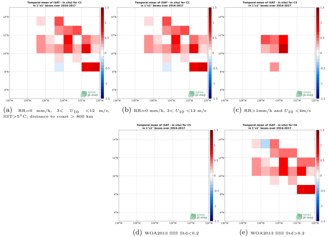
Figure 11: Temporal mean gridded over spatial boxes of size 1^{\circ}\times 1^{\circ} of \Delta\text{SSS} (SMOS SSS L3 v2 - Daily - 0.5 Deg (CATDS-CECOS-IFREMER) - Waveglider) for 5 different subdatasets corresponding to:RR=0 mm/h, 3 < U_{10} < 12 m/s, SST >5^{\circ}\text{C} , distance to coast > 800 km (a), RR=0 mm/h, 3 < U_{10} < 12 m/s (b), RR >1 mm/h and U_{10} < 4 m/s (c), WOA2013 SSS Std <0.2 (d), WOA2013 SSS Std >0.2 (e).
