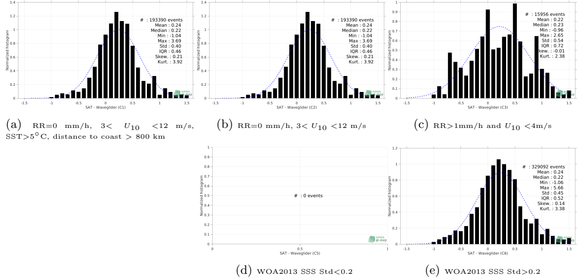
Figure 12: Normalized histogram of \Delta SSS (SMOS SSS L3 v2 - Daily - 0.5 Deg (CATDS-CECOS-IFREMER) - Waveglider) for 5 different subdatasets corresponding to: RR=0 mm/h, 3 < U_{10} < 12 m/s, SST > 5°C, distance to coast > 800 km (a), RR=0 mm/h, 3 < U_{10} < 12 m/s (b), RR > 1mm/h and U_{10} < 4 m/s (c), WOA2013 SSS Std < 0.2 (d), WOA2013 SSS Std > 0.2 (e).
