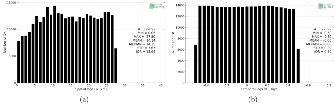
Figure 4: Histograms of the spatial (a) and temporal (b) lags between the location/time of the Waveglider measurement and the date of the corresponding SMOS SSS L3 v2 - Daily - 0.5 Deg (CATDS-CECOS-IFREMER) SSS pixel.
