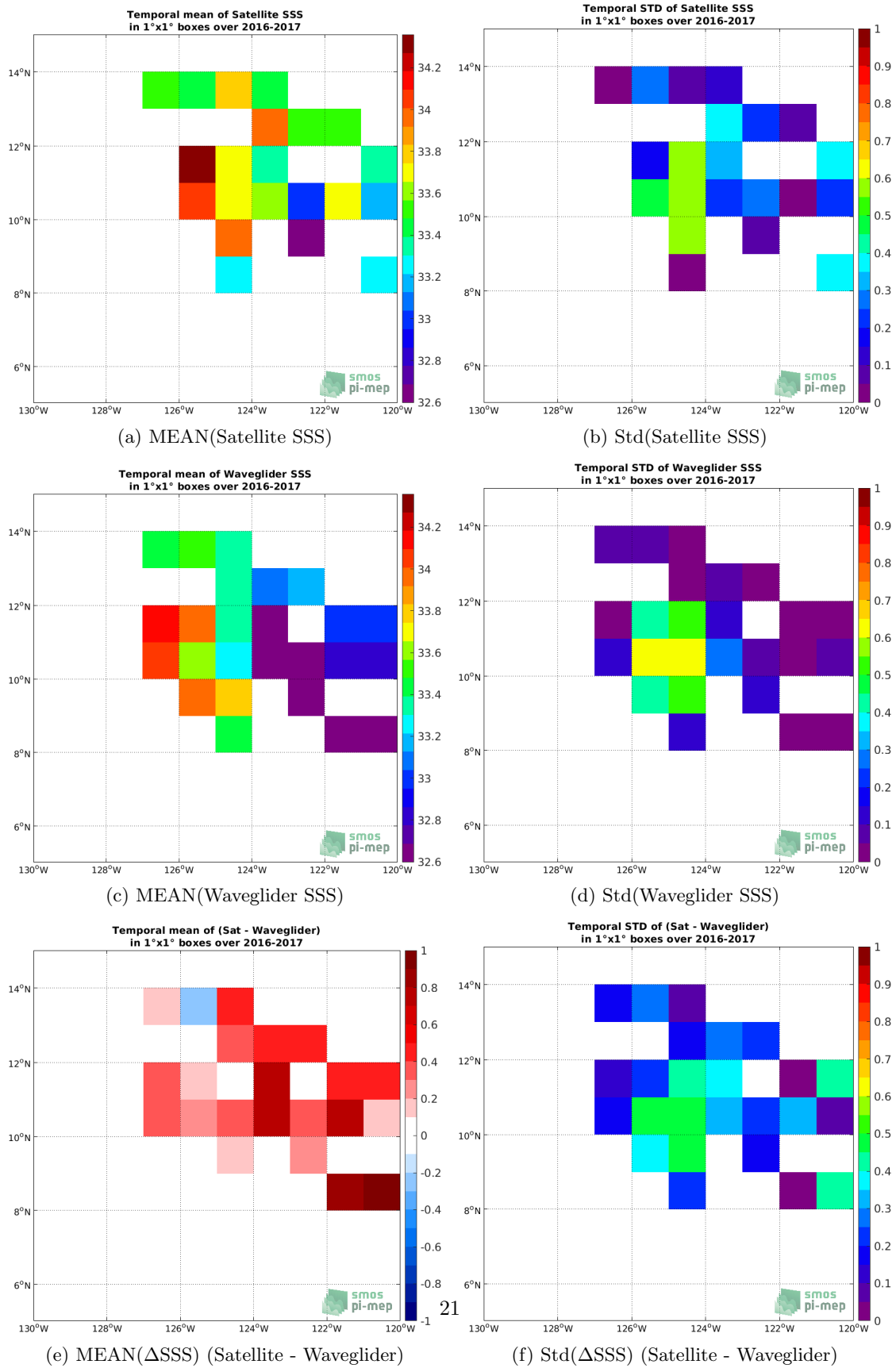
Figure 5: Temporal mean (left) and Std (right) of SSS from SMOS SSS L3 v2 - Daily - 0.5 Deg (CATDS-CECOS-IFREMER) (top), Waveglider (middle), and of \Delta SSS (Satellite - Waveglider). Only match-up pairs are used to generate these maps.
