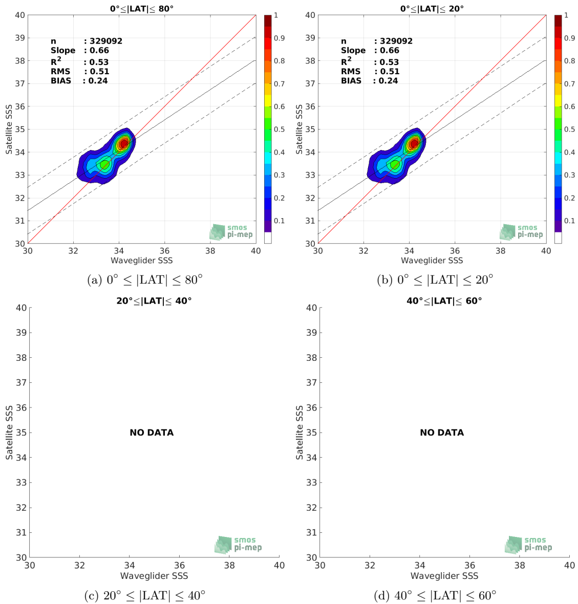
Figure 8: Contour maps of the concentration of SMOS SSS L3 v2 - Daily - 0.5 Deg (CATDS-CECOS-IFREMER) SSS ( y -axis) versus Waveglider SSS ( x -axis) at match-up pairs for different latitude bands. For each plot, the red line shows x=y . The black thin and dashed lines indicate a linear fit through the data cloud and the \pm 95\% confidence levels, respectively. The number match-up pairs n , the slope and R^2 coefficient of the linear fit, the root mean square (RMS) and the mean bias between satellite and in situ data are indicated for each latitude band in each plots.
