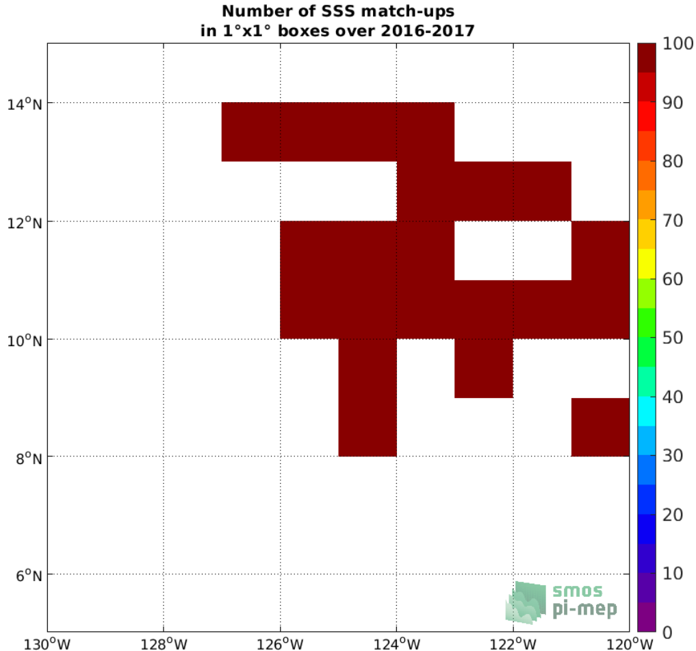
Figure 3: Number of SSS match-ups between Waveglider SSS and the SMOS SSS L3 v2 - Daily - 0.5 Deg (CATDS-CECOS-IFREMER) SSS product for the SPURS 2 Pi-MEP region over 1^\circ \times 1^\circ boxes and for the full satellite product period.
