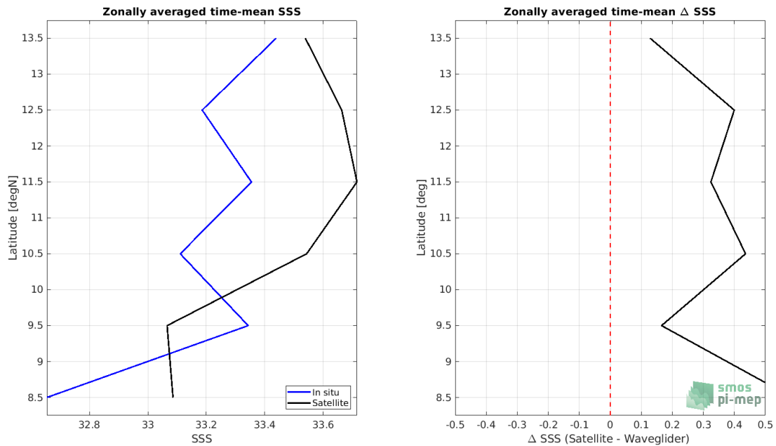
Figure 7: Left panel: Zonal mean SSS from SMOS SSS L3 v2 - Daily - 0.5 Deg (CATDS-CECOS-IFREMER) satellite product (black) and from Waveglider (blue). Right panel: Zonal mean of \Delta SSS (Satellite - Waveglider) for all the collected Pi-MEP match-up pairs estimated over the full satellite product period.
