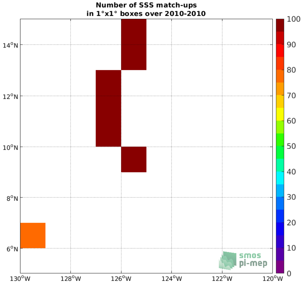
Figure 4: Number of SSS match-ups between TSG (GOSUD-Sailing-ship) SSS and the SMOS SSS L3 v2 - Daily - 0.5 Deg (CATDS-CECOS-IFREMER) SSS product for the SPURS 2 Pi-MEP region over 1°x1° boxes and for the full satellite product period.
