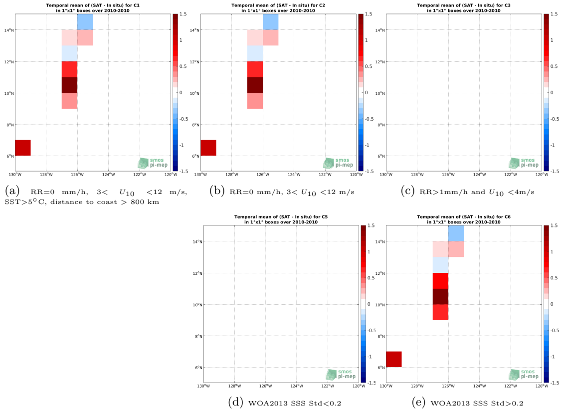
Figure 12: Temporal mean gridded over spatial boxes of size 1^\circ \times 1^\circ of \Delta SSS (SMOS SSS L3 v2 - Daily - 0.5 Deg (CATDS-CECOS-IFREMER) - TSG (GOSUD-Sailing-ship)) for 5 different subdatasets corresponding to: RR=0 mm/h, 3 < U_{10} < 12 m/s, SST>5°C, distance to coast > 800 km (a), RR=0 mm/h, 3 < U_{10} < 12 m/s (b), RR>1mm/h and U_{10} < 4 m/s (c), WOA2013 SSS Std<0.2 (d), WOA2013 SSS Std>0.2 (e).
