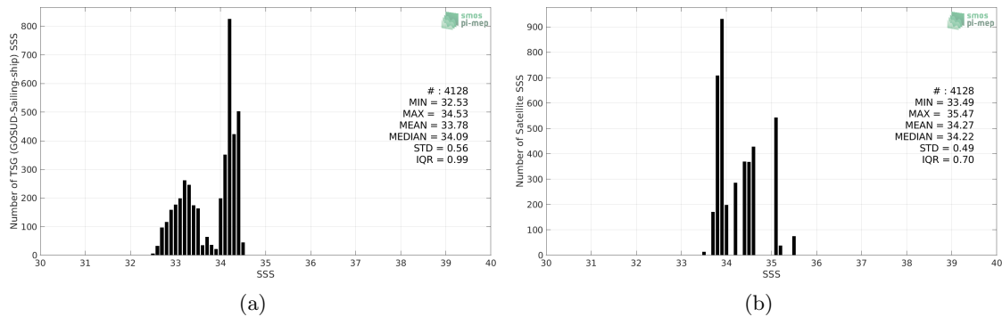
Figure 2: Histograms of SSS from TSG (GOSUD-Sailing-ship) (a) and SMOS SSS L3 v2 - Daily - 0.5 Deg (CATDS-CECOS-IFREMER) (b) considering all match-up pairs per bins of 0.1 over the SPURS 2 Pi-MEP region and for the full satellite product period.
