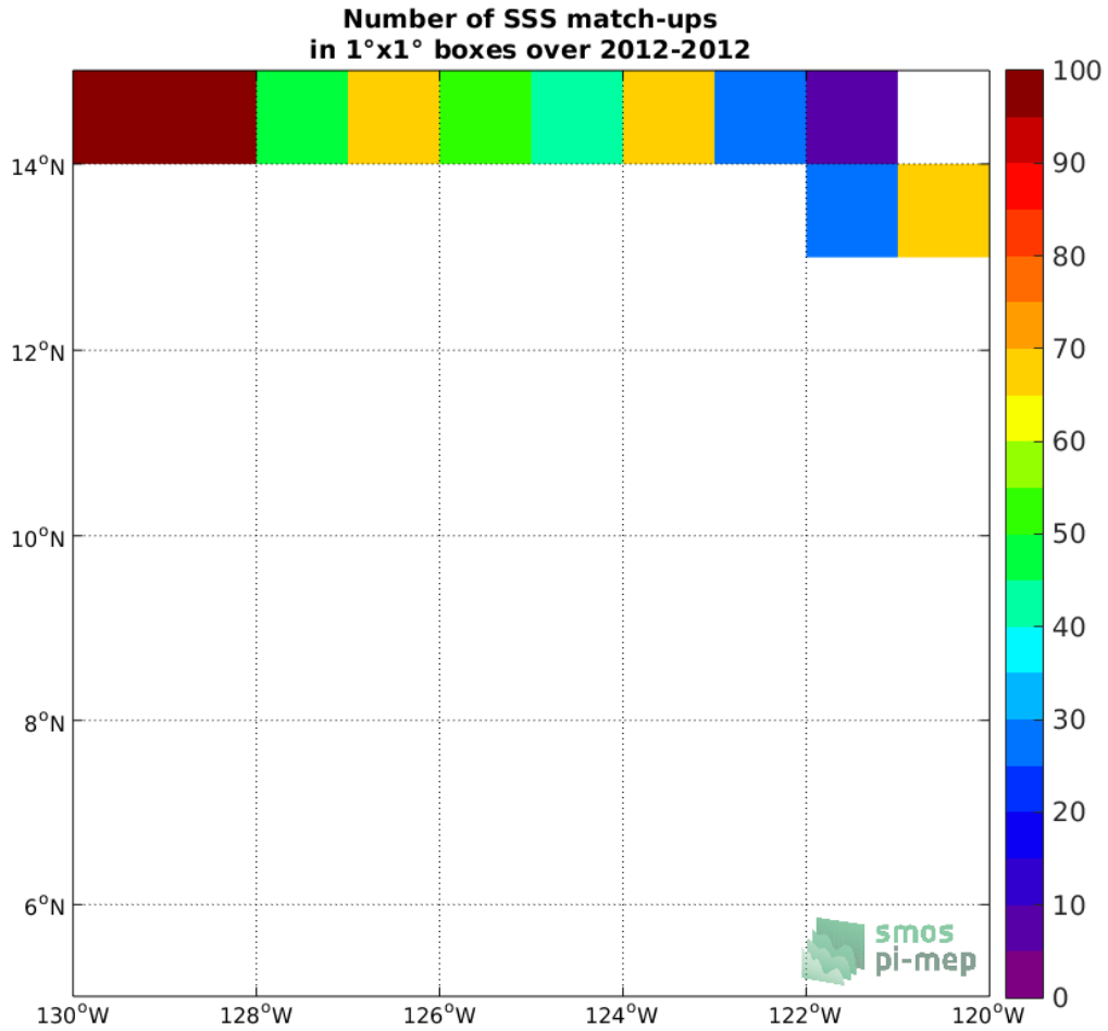
Figure 4: Number of SSS match-ups between TSG (GOSUD-Research-vessel) SSS and the SMOS SSS L3 v2 - Daily - 0.5 Deg (CATDS-CECOS-IFREMER) SSS product for the SPURS 2 Pi-MEP region over 1°x1° boxes and for the full satellite product period.
