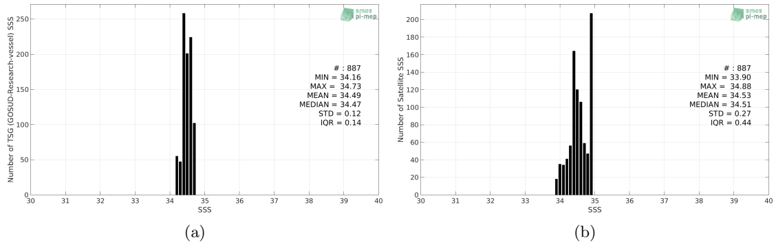
Figure 2: Histograms of SSS from TSG (GOSUD-Research-vessel) (a) and SMOS SSS L3 v2 - Daily - 0.5 Deg (CATDS-CECOS-IFREMER) (b) considering all match-up pairs per bins of 0.1 over the SPURS 2 Pi-MEP region and for the full satellite product period.
