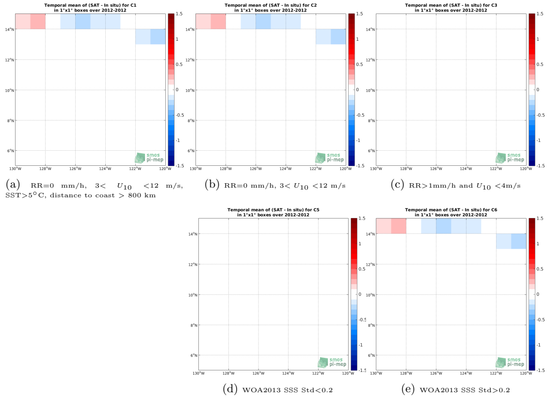
Figure 12: Temporal mean gridded over spatial boxes of size 1^\circ \times 1^\circ of \Delta SSS (SMOS SSS L3 v2 - Daily - 0.5 Deg (CATDS-CECOS-IFREMER) - TSG (GOSUD-Research-vessel)) for 5 different subdatasets corresponding to: RR=0 mm/h, 3 < U_{10} < 12 m/s, SST > 5°C, distance to coast > 800 km (a), RR=0 mm/h, 3 < U_{10} < 12 m/s (b), RR > 1mm/h and U_{10} < 4 m/s (c), WOA2013 SSS Std < 0.2 (d), WOA2013 SSS Std > 0.2 (e).
