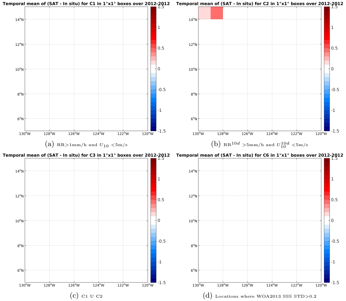
Figure 12: Temporal mean gridded over spatial boxes of size 1°x1° of \Delta SSS (SMOS-L3-CATDS-CECOS-IFREMER-V2-1DAY-0.5DEG - TSG-GOSUD-Research-vessel) for 4 different subdatasets corresponding to:RR>1mm/h and U_{10} < 5m/s (a), RR^{10d} > 5mm/h and U_{10}^{10d} < 5m/s (b), C1 U C2 (c),Locations where WOA2013 SSS STD>0.2 (d).
