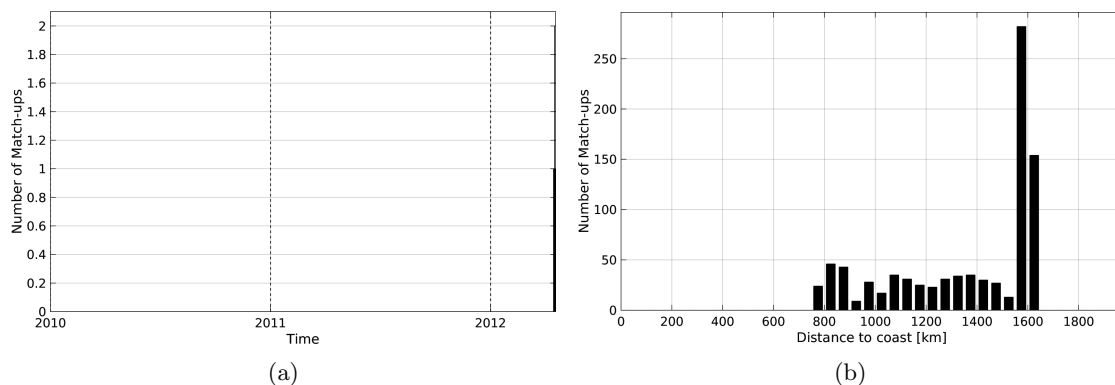
Figure 1: Number of match-ups between TSG-GOSUD-Research-vessel and SMOS-L3-CATDS-CECOS-IFREMER-V2-1DAY-0.5deg SSS as a function of time (a) and as function of the distance to coast (b) over the SPURS 2 Pi-MEP region and for the full satellite product period.
