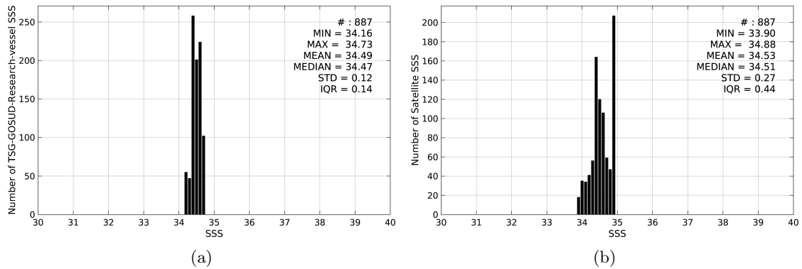
Figure 2: Histograms of SSS from TSG-GOSUD-Research-vessel (a) and SMOS-L3-CATDS-CECOS-IFREMER-V2-1DAY-0.5deg (b) considering all match-up pairs per bins of 0.1 over the SPURS 2 Pi-MEP region and for the full satellite product period.
