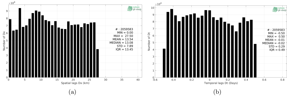
Figure 4: Histograms of the spatial (a) and temporal (b) lags between the location/time of the Salinity Snake measurement and the date of the corresponding SMOS SSS L3 v2 - Daily - 0.5 Deg (CATDS-CECOS-IFREMER) SSS pixel.
