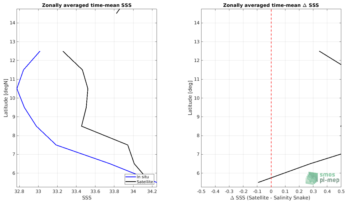
Figure 7: Left panel: Zonal mean SSS from SMOS SSS L3 v2 - Daily - 0.5 Deg (CATDS-CECOS-IFREMER) satellite product (black) and from Salinity Snake (blue). Right panel: Zonal mean of \Delta SSS (Satellite - Salinity Snake) for all the collected Pi-MEP match-up pairs estimated over the full satellite product period.
