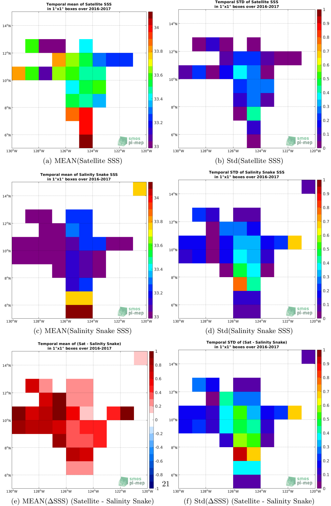
Figure 5: Temporal mean (left) and Std (right) of SSS from SMOS SSS L3 v2 - Daily - 0.5 Deg (CATDS-CECOS-IFREMER) (top), Salinity Snake (middle), and of \Delta SSS (Satellite - Salinity Snake). Only match-up pairs are used to generate these maps.
