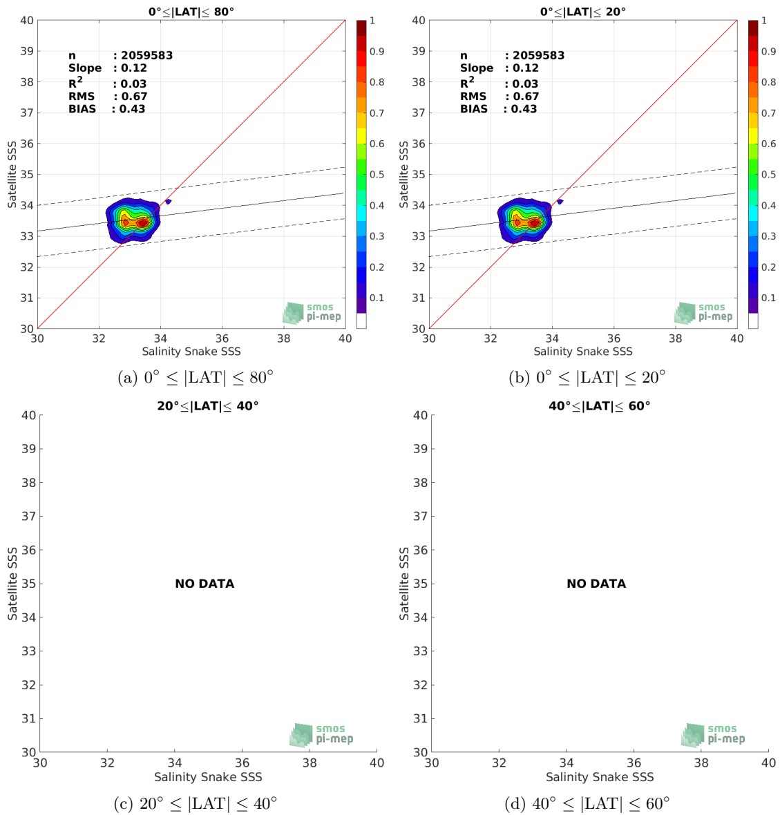
Figure 8: Contour maps of the concentration of SMOS SSS L3 v2 - Daily - 0.5 Deg (CATDS-CECOS-IFREMER) SSS (y-axis) versus Salinity Snake SSS (x-axis) at match-up pairs for different latitude bands. For each plot, the red line shows x=y . The black thin and dashed lines indicate a linear fit through the data cloud and the \pm 95\% confidence levels, respectively. The number match-up pairs n , the slope and R^2 coefficient of the linear fit, the root mean square (RMS) and the mean bias between satellite and in situ data are indicated for each latitude band in each plots.
