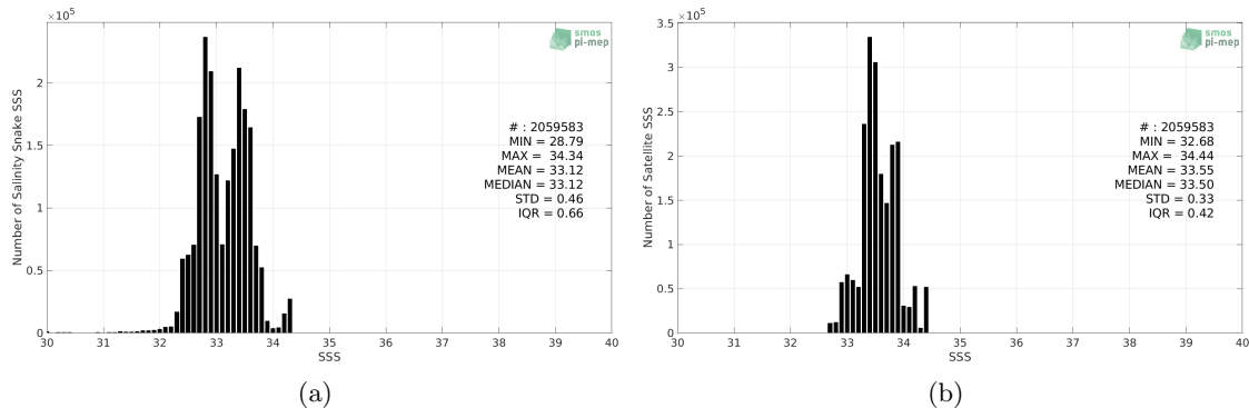
Figure 2: Histograms of SSS from Salinity Snake (a) and SMOS SSS L3 v2 - Daily - 0.5 Deg (CATDS-CECOS-IFREMER) (b) considering all match-up pairs per bins of 0.1 over the SPURS 2 Pi-MEP region and for the full satellite product period.
