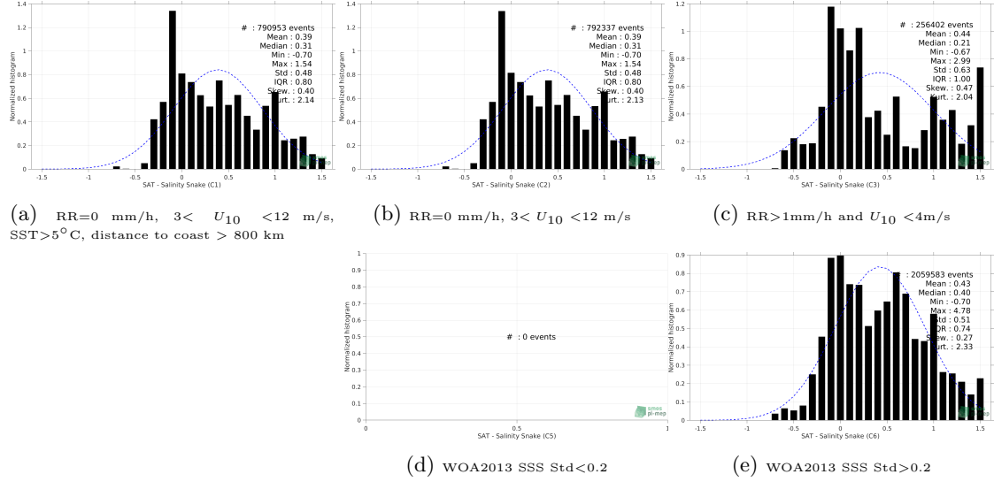
Figure 12: Normalized histogram of \Delta SSS (SMOS SSS L3 v2 - Daily - 0.5 Deg (CATDS-CECOS-IFREMER) - Salinity Snake) for 5 different subdatasets corresponding to: RR=0 mm/h, 3 < U_{10} < 12 m/s, SST > 5°C, distance to coast > 800 km (a), RR=0 mm/h, 3 < U_{10} < 12 m/s (b), RR > 1mm/h and U_{10} < 4 m/s (c), WOA2013 SSS Std < 0.2 (d), WOA2013 SSS Std > 0.2 (e).
