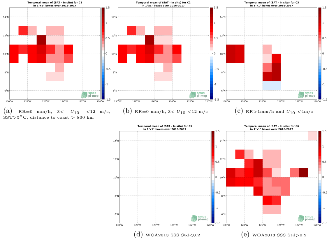
Figure 11: Temporal mean gridded over spatial boxes of size 1^{\circ}\times 1^{\circ} of \Delta\text{SSS} (SMOS SSS L3 v2 - Daily - 0.5 Deg (CATDS-CECOS-IFREMER) - Salinity Snake) for 5 different subdatasets corresponding to:RR=0 mm/h, 3 < U_{10} < 12 m/s, SST >5^{\circ}\text{C} , distance to coast > 800 km (a), RR=0 mm/h, 3 < U_{10} < 12 m/s (b), RR >1 mm/h and U_{10} < 4 m/s (c), WOA2013 SSS Std <0.2 (d), WOA2013 SSS Std >0.2 (e).
