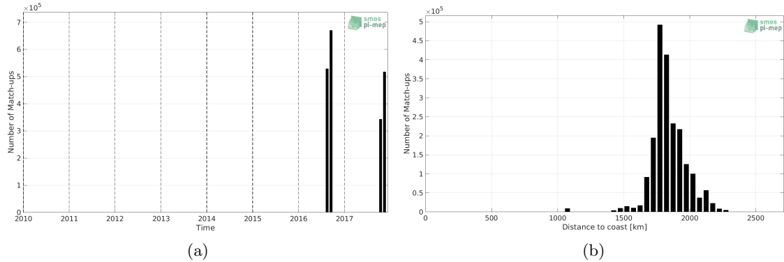
Figure 1: Number of match-ups between Salinity Snake and SMOS SSS L3 v2 - Daily - 0.5 Deg (CATDS-CECOS-IFREMER) SSS as a function of time (a) and as function of the distance to coast (b) over the SPURS 2 Pi-MEP region and for the full satellite product period.
