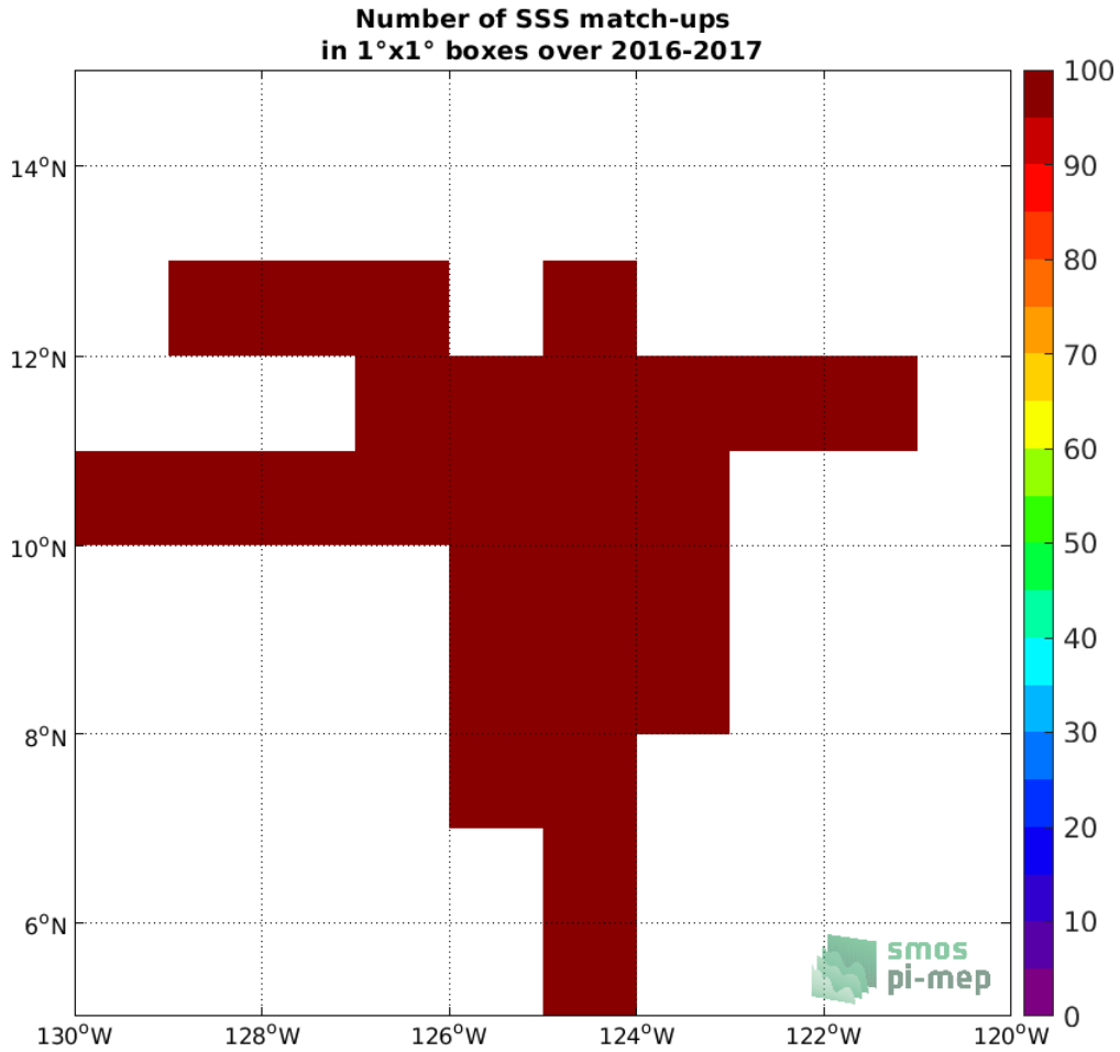
Figure 3: Number of SSS match-ups between Salinity Snake SSS and the SMOS SSS L3 v2 - Daily - 0.5 Deg (CATDS-CECOS-IFREMER) SSS product for the SPURS 2 Pi-MEP region over 1°x1° boxes and for the full satellite product period.
