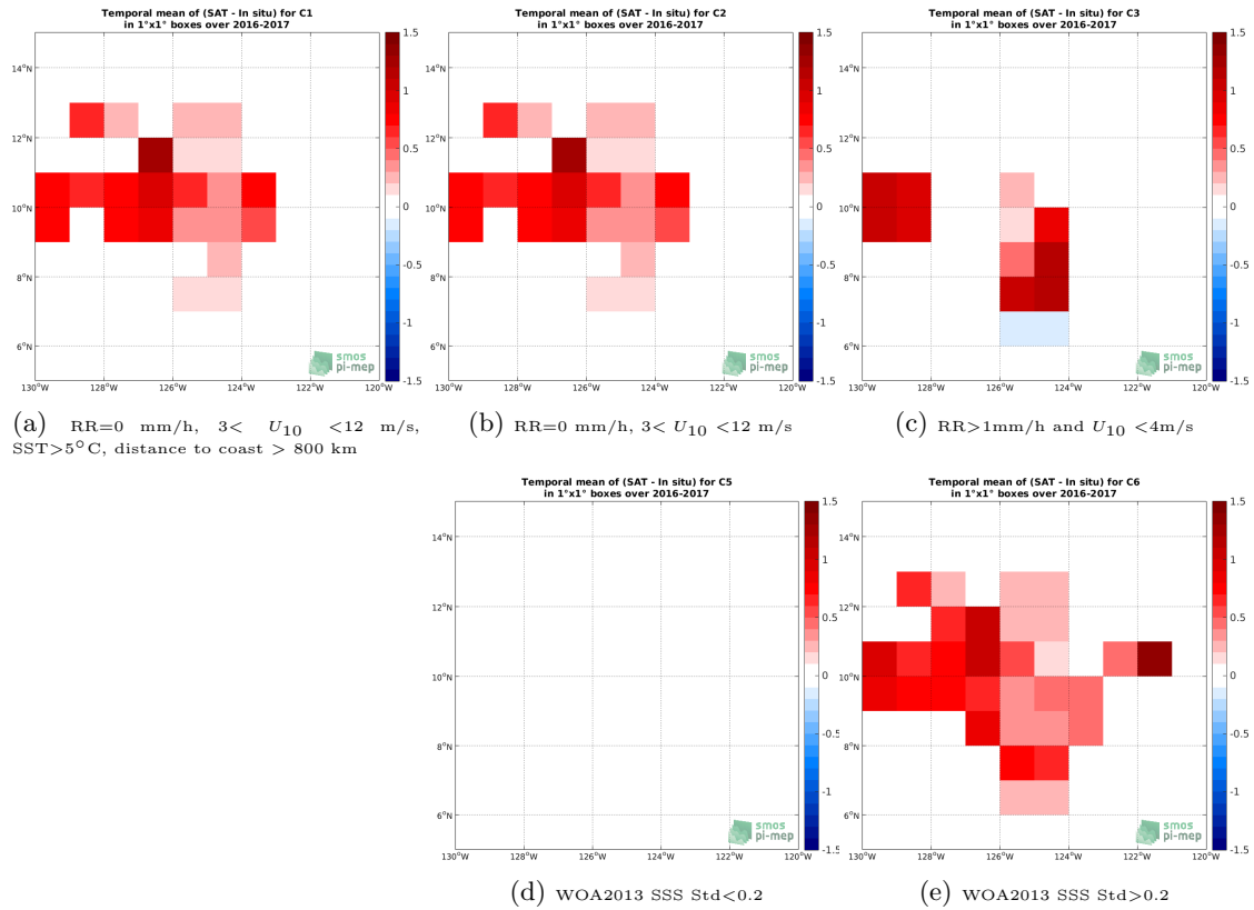
Figure 12: Temporal mean gridded over spatial boxes of size 1^{\circ}\times 1^{\circ} of \Delta\text{SSS} (SMOS SSS L3 v2 - Daily - 0.5 Deg (CATDS-CECOS-IFREMER) - Salinity Snake) for 5 different subdatasets corresponding to:RR=0 mm/h, 3 < U_{10} < 12 m/s, SST >5^{\circ}\text{C} , distance to coast > 800 km (a), RR=0 mm/h, 3 < U_{10} < 12 m/s (b), RR >1 mm/h and U_{10} < 4 m/s (c), WOA2013 SSS Std <0.2 (d), WOA2013 SSS Std >0.2 (e).
