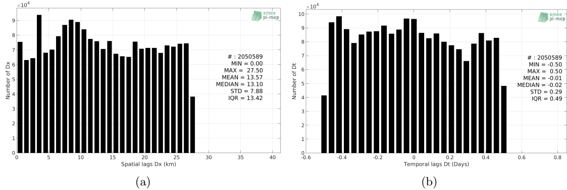
Figure 5: Histograms of the spatial (a) and temporal (b) lags between the time of the Salinity Snake measurements and the date of the corresponding SMOS SSS L3 v2 - Daily - 0.5 Deg (CATDS-CECOS-IFREMER) SSS product.
