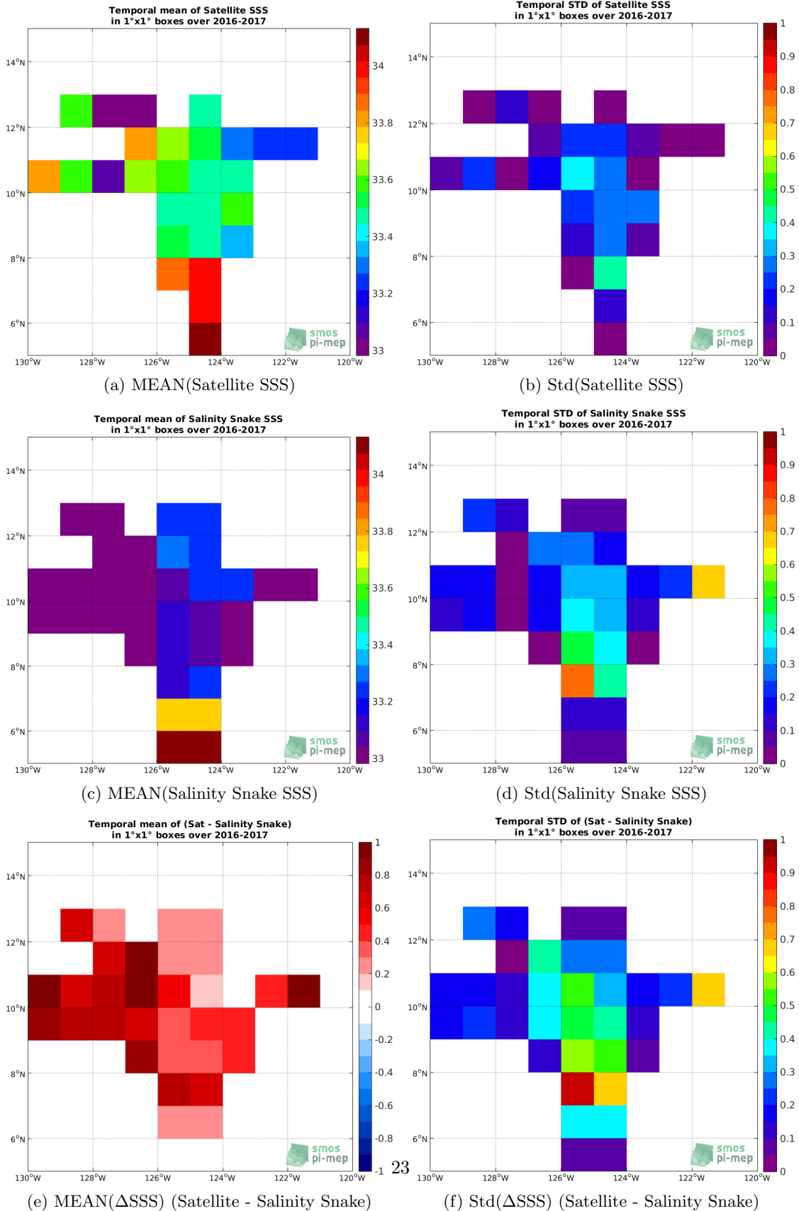
Figure 6: Temporal mean (left) and Std (right) of SSS from SMOS SSS L3 v2 - Daily - 0.5 Deg (CATDS-CECOS-IFREMER) (top), Salinity Snake (middle), and of \Delta SSS (Satellite - Salinity Snake). Only match-up pairs are used to generate these maps.
