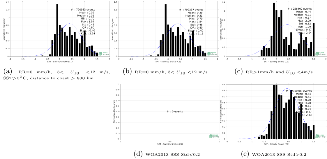
Figure 13: Normalized histogram of \Delta SSS (SMOS SSS L3 v2 - Daily - 0.5 Deg (CATDS-CECOS-IFREMER) - Salinity Snake) for 5 different subdatasets corresponding to: RR=0 mm/h, 3 < U_{10} < 12 m/s, SST>5°C, distance to coast > 800 km (a), RR=0 mm/h, 3 < U_{10} < 12 m/s (b), RR>1mm/h and U_{10} < 4 m/s (c), WOA2013 SSS Std<0.2 (d), WOA2013 SSS Std>0.2 (e).
