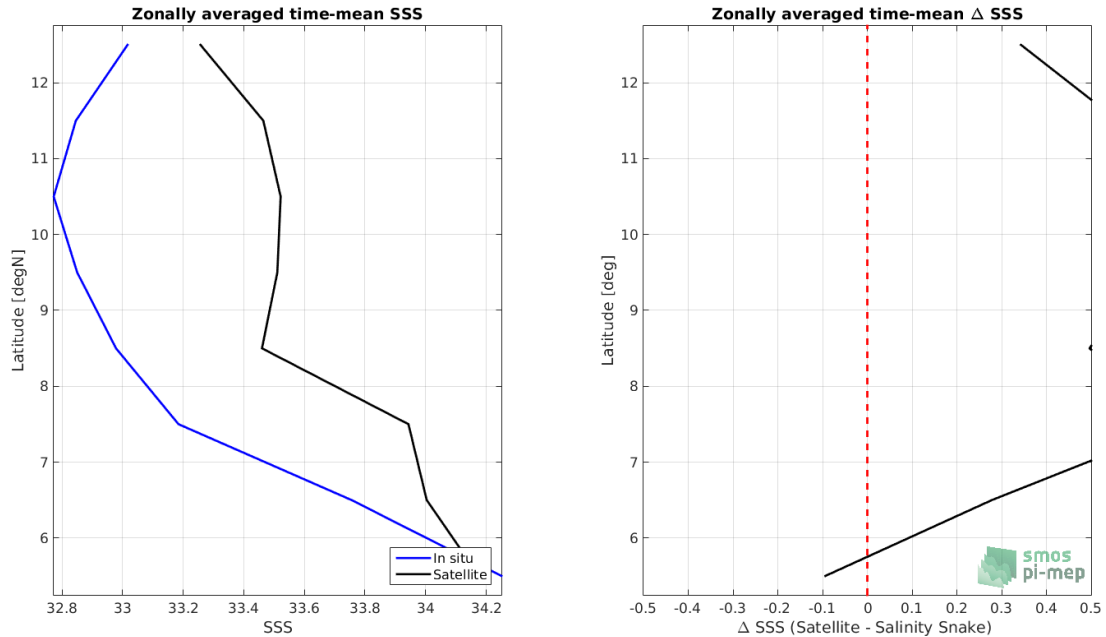
Figure 8: Left panel: Zonal mean SSS from SMOS SSS L3 v2 - Daily - 0.5 Deg (CATDS-CECOS-IFREMER) satellite product (black) and from Salinity Snake (blue). Right panel: Zonal mean of \Delta SSS (Satellite - Salinity Snake) for all the collected Pi-MEP match-up pairs estimated over the full satellite product period.
