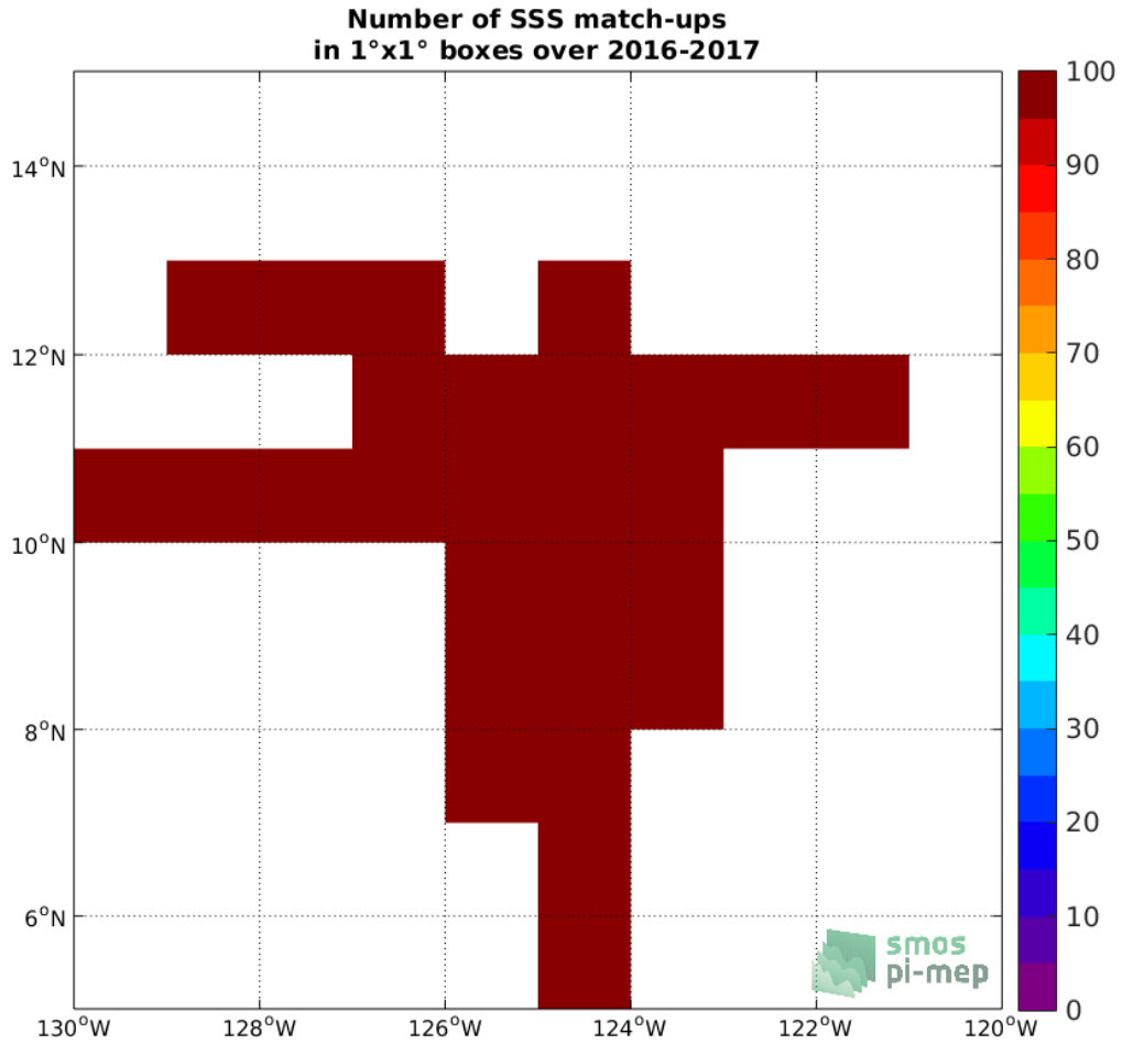
Figure 4: Number of SSS match-ups between Salinity Snake SSS and the SMOS SSS L3 v2 - Daily - 0.5 Deg (CATDS-CECOS-IFREMER) SSS product for the SPURS 2 Pi-MEP region over 1°x1° boxes and for the full satellite product period.
