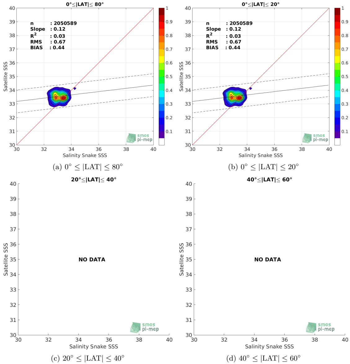
Figure 9: Contour maps of the concentration of SMOS SSS L3 v2 - Daily - 0.5 Deg (CATDS-CECOS-IFREMER) SSS (y-axis) versus Salinity Snake SSS (x-axis) at match-up pairs for different latitude bands. For each plot, the red line shows x=y . The black thin and dashed lines indicate a linear fit through the data cloud and the \pm 95\% confidence levels, respectively. The number match-up pairs n , the slope and R^2 coefficient of the linear fit, the root mean square (RMS) and the mean bias between satellite and in situ data are indicated for each latitude band in each plots.
