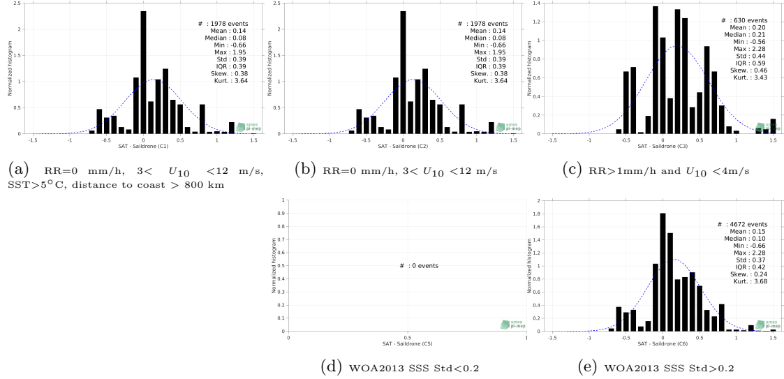
Figure 12: Normalized histogram of \Delta SSS (SMOS SSS L3 v2 - Daily - 0.5 Deg (CATDS-CECOS-IFREMER) - Saildrone) for 5 different subdatasets corresponding to: RR=0 mm/h, 3 < U_{10} < 12 m/s, SST > 5°C, distance to coast > 800 km (a), RR=0 mm/h, 3 < U_{10} < 12 m/s (b), RR > 1mm/h and U_{10} < 4 m/s (c), WOA2013 SSS Std < 0.2 (d), WOA2013 SSS Std > 0.2 (e).
