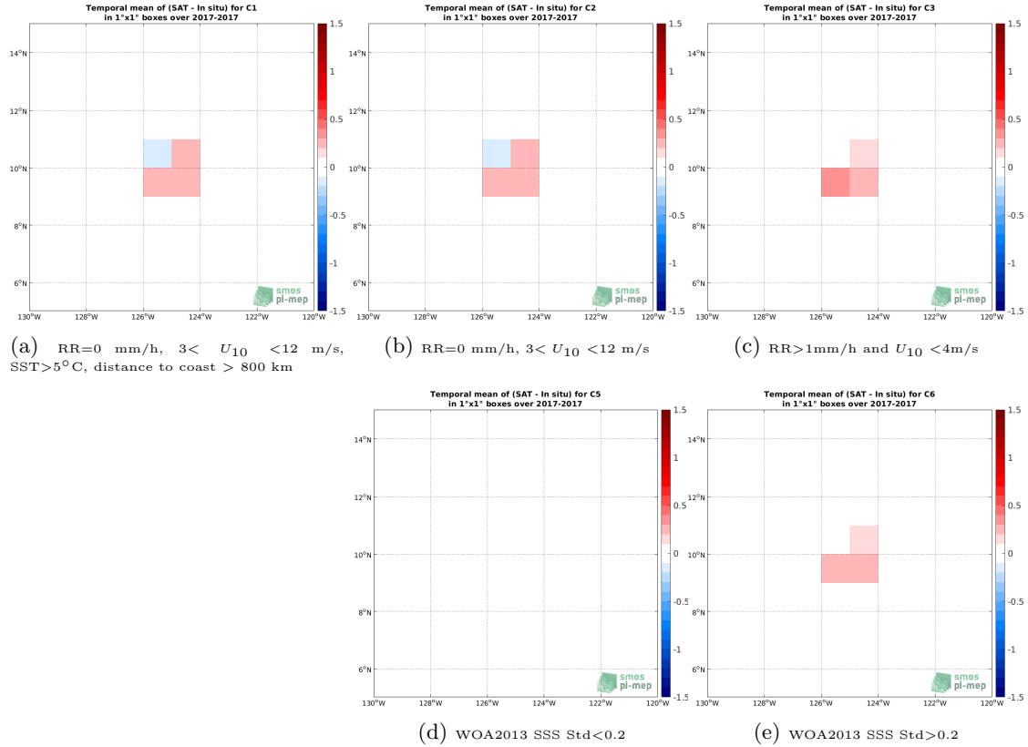
Figure 11: Temporal mean gridded over spatial boxes of size 1^{\circ}\times 1^{\circ} of \Delta\text{SSS} (SMOS SSS L3 v2 - Daily - 0.5 Deg (CATDS-CECOS-IFREMER) - Saildrone) for 5 different subdatasets corresponding to:RR=0 mm/h, 3 < U_{10} < 12 m/s, SST >5^{\circ}\text{C} , distance to coast > 800 km (a), RR=0 mm/h, 3 < U_{10} < 12 m/s (b), RR >1 mm/h and U_{10} < 4 m/s (c), WOA2013 SSS Std <0.2 (d), WOA2013 SSS Std >0.2 (e).
