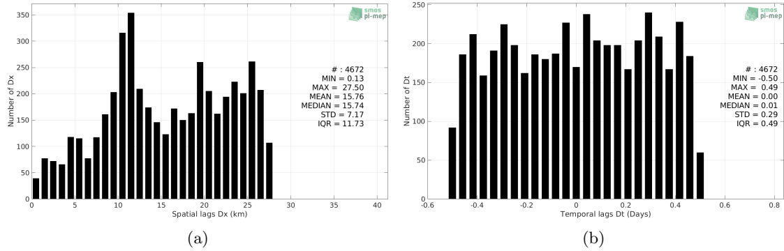
Figure 4: Histograms of the spatial (a) and temporal (b) lags between the location/time of the Saildrone measurement and the date of the corresponding SMOS SSS L3 v2 - Daily - 0.5 Deg (CATDS-CECOS-IFREMER) SSS pixel.
