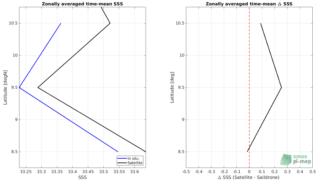
Figure 7: Left panel: Zonal mean SSS from SMOS SSS L3 v2 - Daily - 0.5 Deg (CATDS-CECOS-IFREMER) satellite product (black) and from Sairdrone (blue). Right panel: Zonal mean of \Delta SSS (Satellite - Sairdrone) for all the collected Pi-MEP match-up pairs estimated over the full satellite product period.
