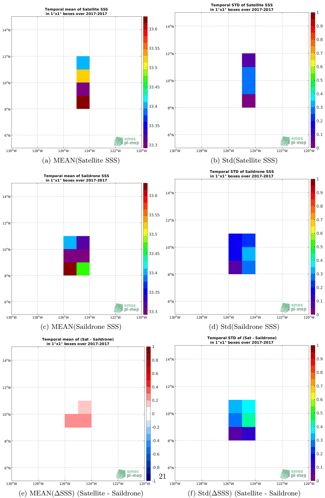
Figure 5: Temporal mean (left) and Std (right) of SSS from SMOS SSS L3 v2 - Daily - 0.5 Deg (CATDS-CECOS-IFREMER) (top), Saildrone (middle), and of \Delta SSS (Satellite - Saildrone). Only match-up pairs are used to generate these maps.
