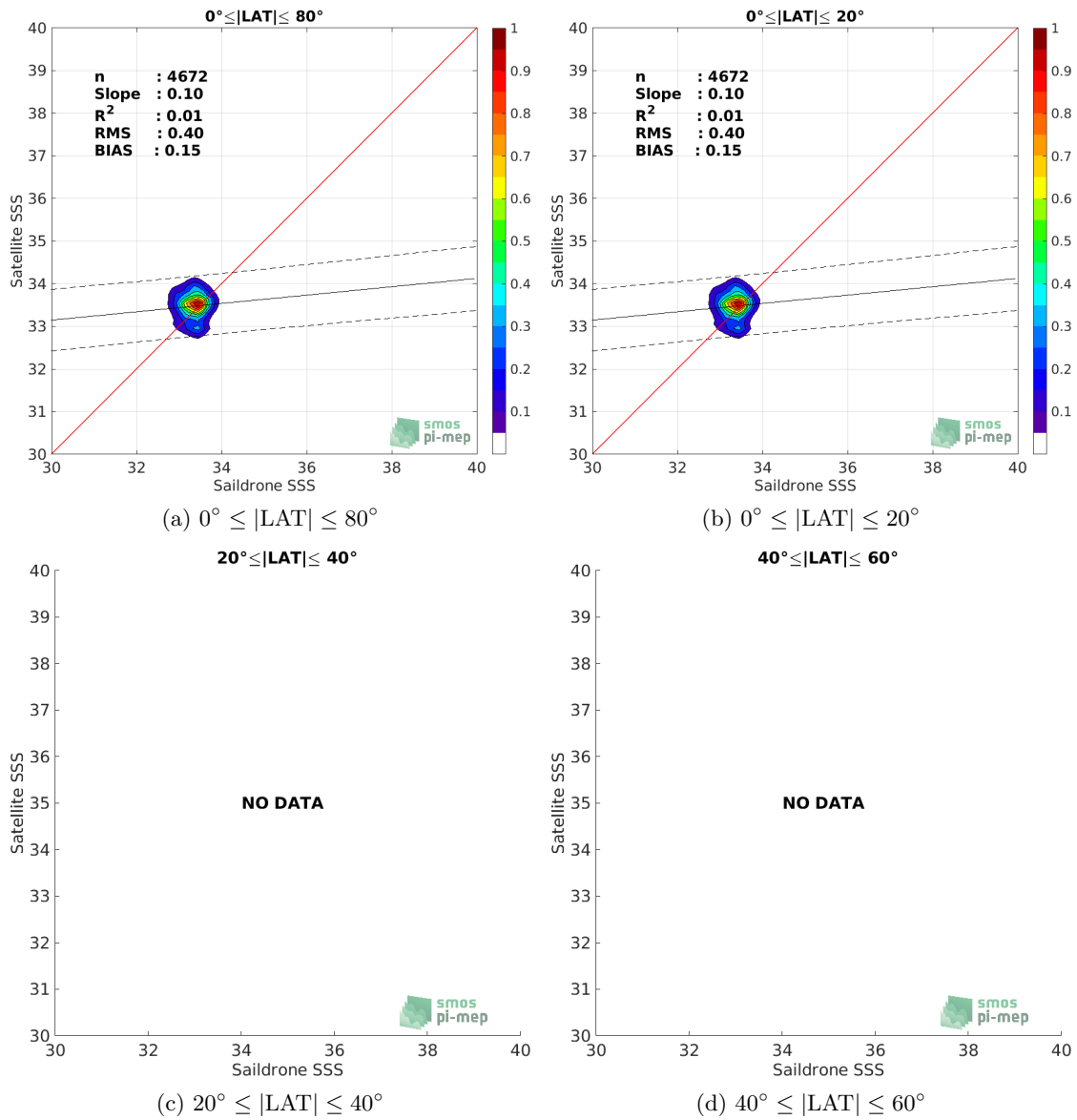
Figure 8: Contour maps of the concentration of SMOS SSS L3 v2 - Daily - 0.5 Deg (CATDS-CECOS-IFREMER) SSS (y-axis) versus Saildrone SSS (x-axis) at match-up pairs for different latitude bands. For each plot, the red line shows x=y . The black thin and dashed lines indicate a linear fit through the data cloud and the \pm 95\% confidence levels, respectively. The number match-up pairs n , the slope and R^2 coefficient of the linear fit, the root mean square (RMS) and the mean bias between satellite and in situ data are indicated for each latitude band in each plots.
