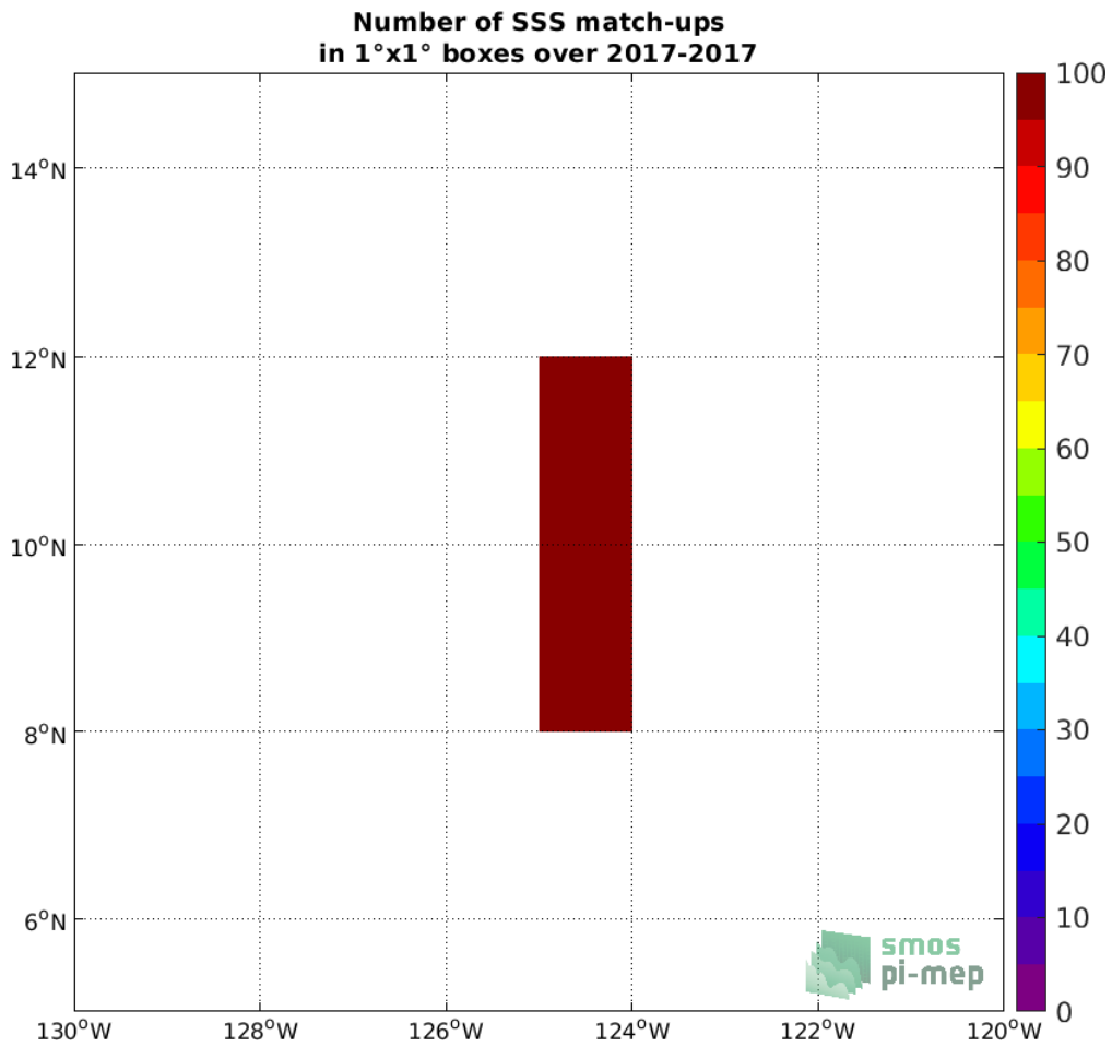
Figure 3: Number of SSS match-ups between Saildrone SSS and the SMOS SSS L3 v2 - Daily - 0.5 Deg (CATDS-CECOS-IFREMER) SSS product for the SPURS 2 Pi-MEP region over 1°x1° boxes and for the full satellite product period.
