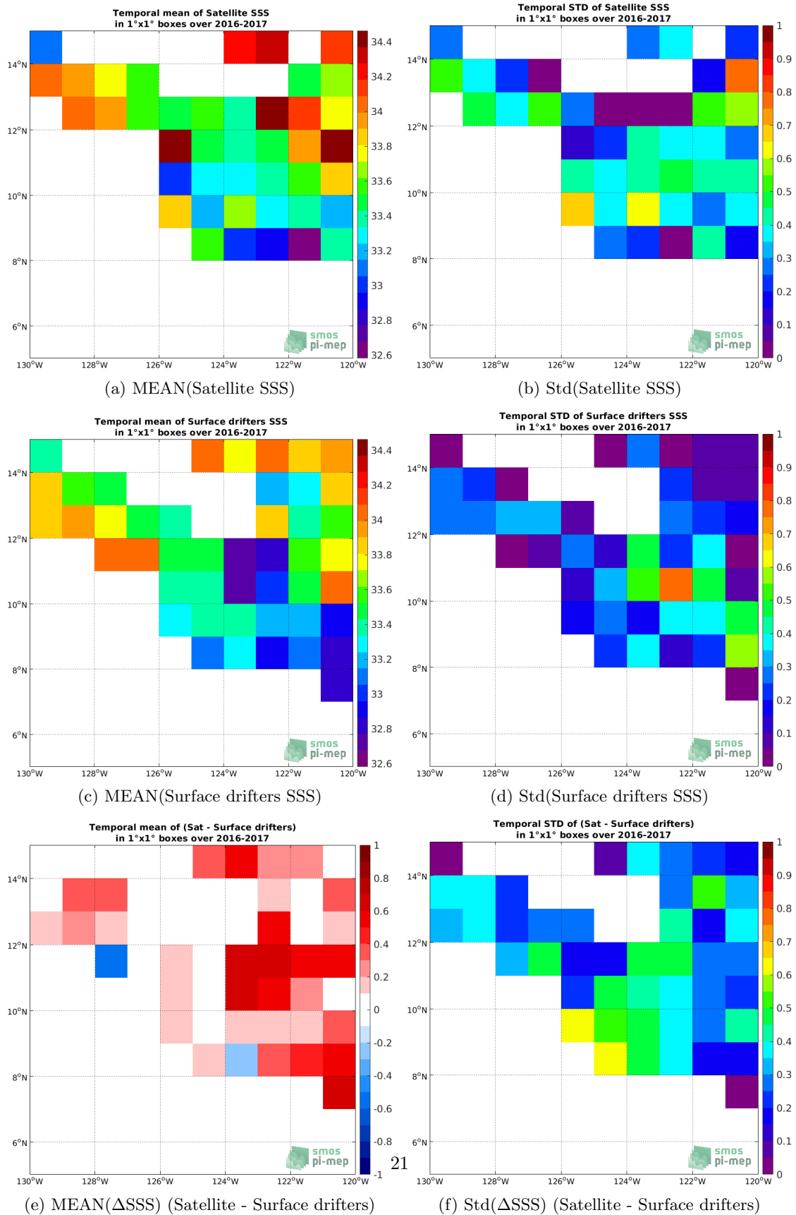
Figure 5: Temporal mean (left) and Std (right) of SSS from SMOS SSS L3 v2 - Daily - 0.5 Deg (CATDS-CECOS-IFREMER) (top), Surface drifters (middle), and of \Delta SSS (Satellite - Surface drifters). Only match-up pairs are used to generate these maps.
