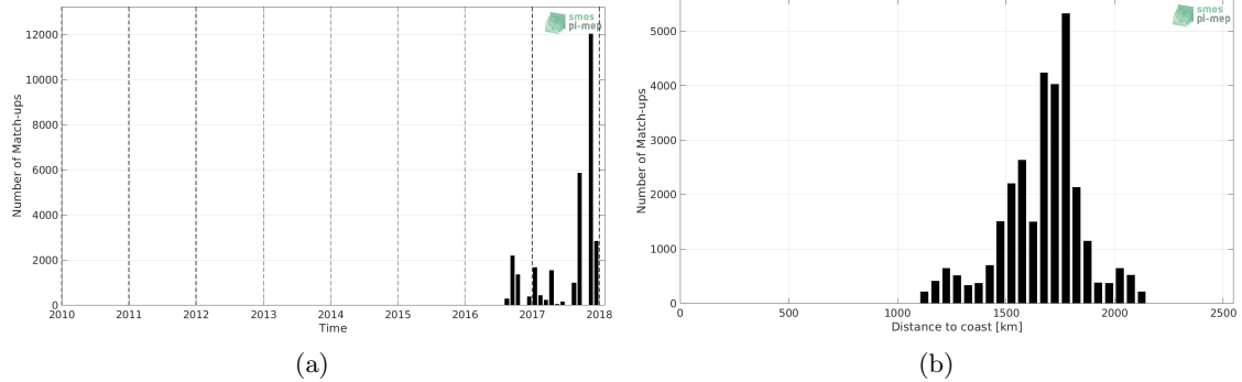
Figure 1: Number of match-ups between Surface drifters and SMOS SSS L3 v2 - Daily - 0.5 Deg (CATDS-CECOS-IFREMER) SSS as a function of time (a) and as function of the distance to coast (b) over the SPURS 2 Pi-MEP region and for the full satellite product period.
