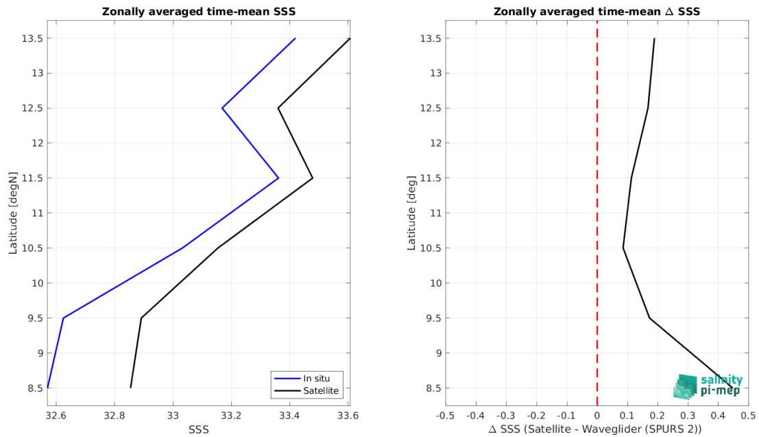
Figure 9: Left panel: Zonal mean SSS from SMOS SSS L3 v335 - Monthly - 25 km (CATDS-CPDC) satellite product (black) and from Waveglider (SPURS 2) (blue). Right panel: Zonal mean of \Delta SSS (Satellite - Waveglider (SPURS 2)) for all the collected Pi-MEP match-up pairs estimated over the full satellite product period.
