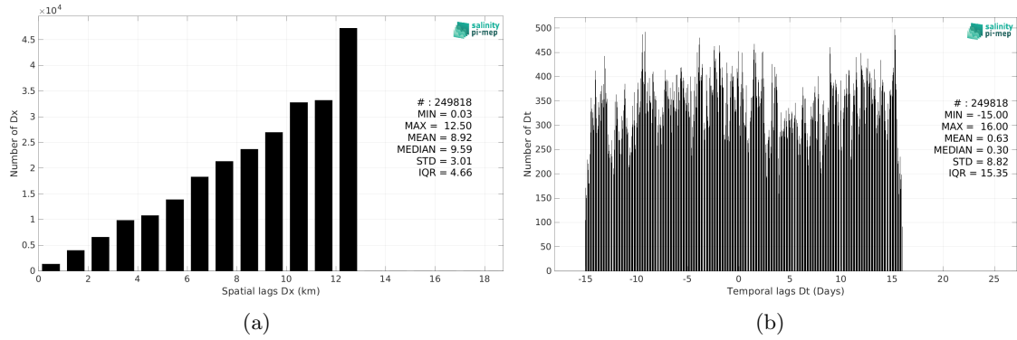
Figure 6: Histograms of the spatial (a) and temporal (b) lags between the location/time of the Waveglider (SPURS 2) measurement and the date of the corresponding SMOS SSS L3 v335 - Monthly - 25 km (CATDS-CPDC) SSS pixel.
