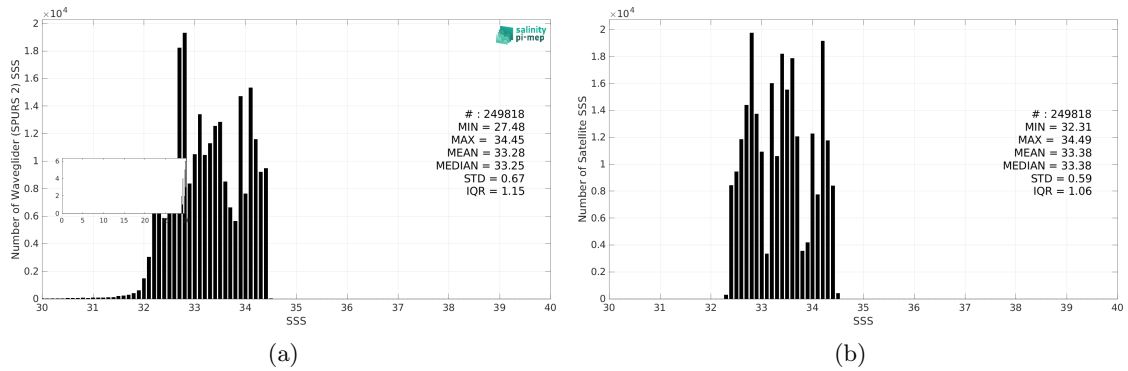
Figure 3: Histograms of SSS from Waveglider (SPURS 2) (a) and SMOS SSS L3 v335 - Monthly - 25 km (CATDS-CPDC) (b) considering all match-up pairs per bins of 0.1 over the SPURS 2 Pi-MEP region and for the full satellite product period.
