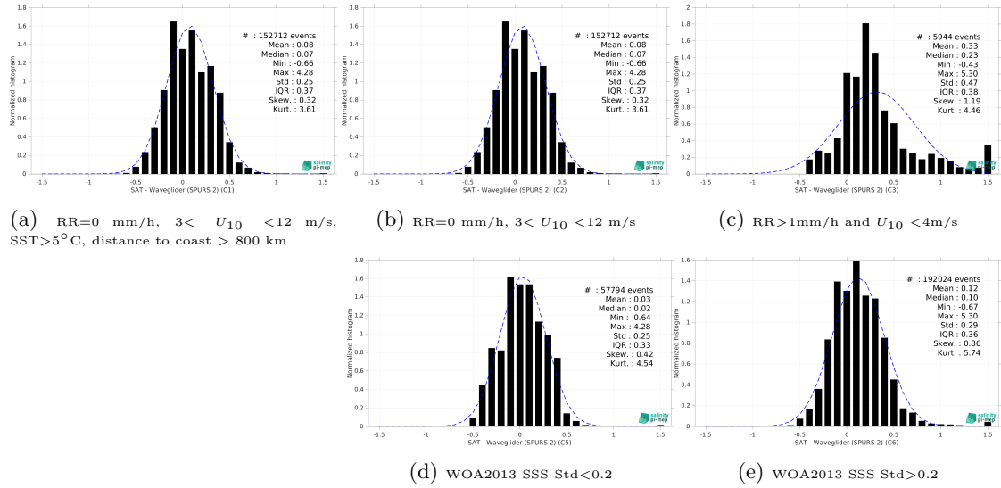
Figure 15: Normalized histogram of \Delta SSS (SMOS SSS L3 v335 - Monthly - 25 km (CATDS-CPDC) - Waveglider (SPURS 2) for 5 different subdatasets corresponding to: RR=0 mm/h, 3 < U_{10} < 12 m/s, SST > 5°C, distance to coast > 800 km (a), RR=0 mm/h, 3 < U_{10} < 12 m/s (b), RR > 1mm/h and U_{10} < 4 m/s (c), WOA2013 SSS Std < 0.2 (d), WOA2013 SSS Std > 0.2 (e).
