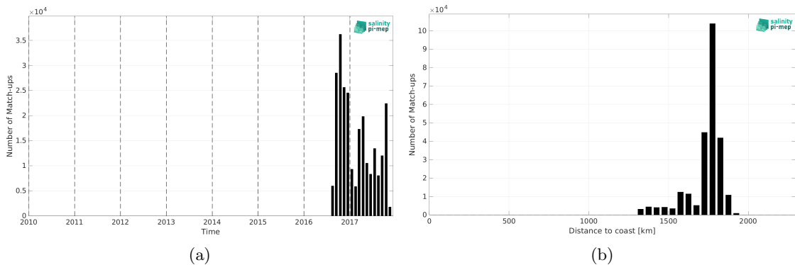
Figure 2: Number of match-ups between Waveglider (SPURS 2) and SMOS SSS L3 v335 - Monthly - 25 km (CATDS-CPDC) SSS as a function of time (a) and as function of the distance to coast (b) over the SPURS 2 Pi-MEP region and for the full satellite product period.
