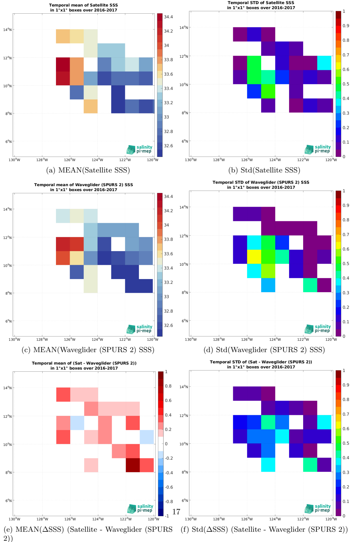
Figure 7: Temporal mean (left) and Std (right) of SSS from SMOS SSS L3 v335 - Monthly - 25 km (CATDS-CPDC) (top), Waveglider (SPURS 2) (middle), and of \Delta SSS (Satellite - Waveglider (SPURS 2)). Only match-up pairs are used to generate these maps.
