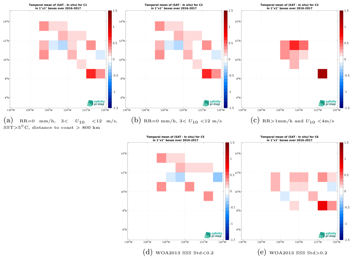
Figure 14: Temporal mean gridded over spatial boxes of size 1^\circ \times 1^\circ of \Delta\text{SSS} (SMOS SSS L3 v335 - Monthly - 25 km (CATDS-CPDC) - Waveglider (SPURS 2)) for 5 different subdatasets corresponding to:RR=0 mm/h, 3 < U_{10} < 12 m/s, SST>5°C, distance to coast > 800 km (a), RR=0 mm/h, 3 < U_{10} < 12 m/s (b), RR>1mm/h and U_{10} < 4 m/s (c), WOA2013 SSS Std<0.2 (d), WOA2013 SSS Std>0.2 (e).
