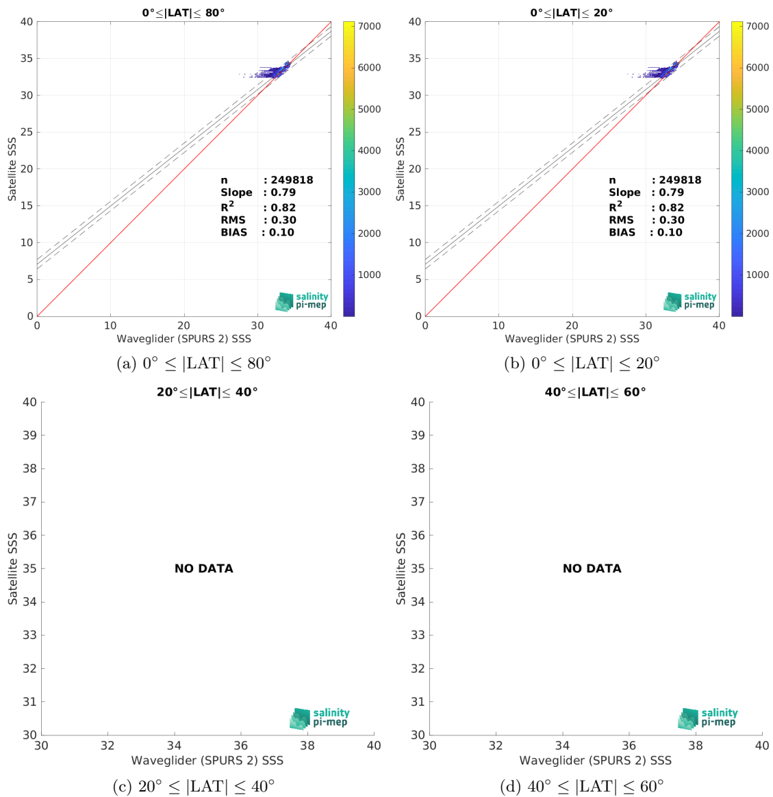
Figure 10: Contour maps of the concentration of SMOS SSS L3 v335 - Monthly - 25 km (CATDS-CPDC) SSS (y-axis) versus Waveglider (SPURS 2) SSS (x-axis) at match-up pairs for different latitude bands. For each plot, the red line shows x=y . The black thin and dashed lines indicate a linear fit through the data cloud and the \pm 95\% confidence levels, respectively. The number match-up pairs n , the slope and R^2 coefficient of the linear fit, the root mean square (RMS) and the mean bias between satellite and in situ data are indicated for each latitude band in each plots.
