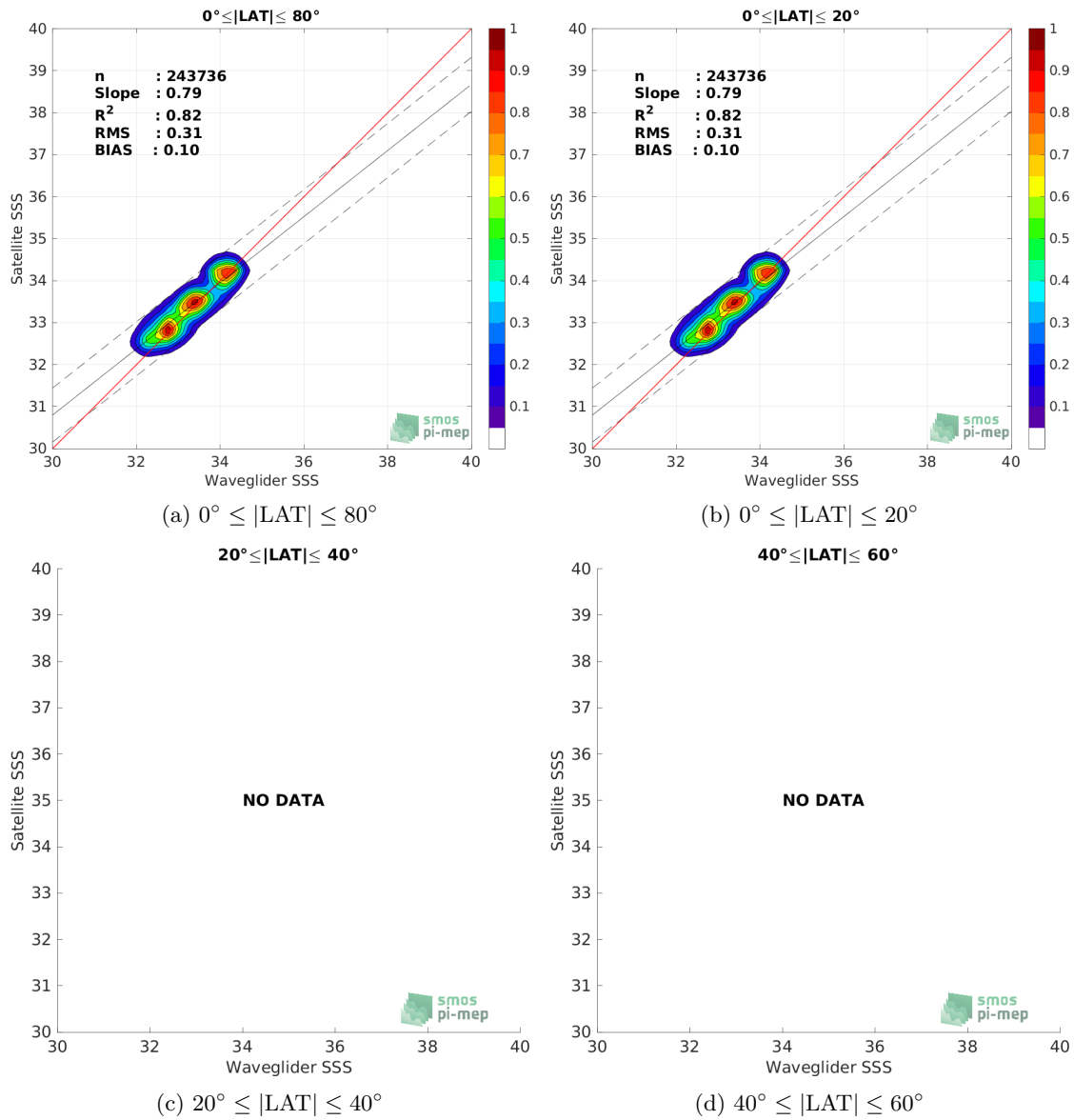
Figure 9: Contour maps of the concentration of SMOS SSS L3 v335 - Monthly - 25 km (CATDS-CPDC) SSS (y-axis) versus Waveglider SSS (x-axis) at match-up pairs for different latitude bands. For each plot, the red line shows x=y . The black thin and dashed lines indicate a linear fit through the data cloud and the \pm 95\% confidence levels, respectively. The number match-up pairs n , the slope and R^2 coefficient of the linear fit, the root mean square (RMS) and the mean bias between satellite and in situ data are indicated for each latitude band in each plots.
