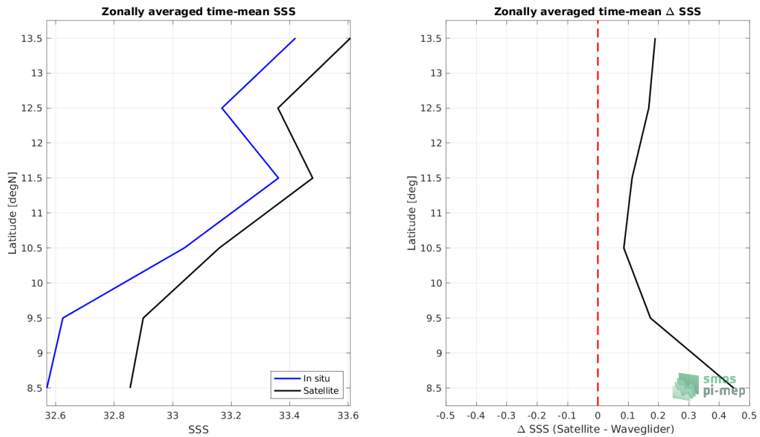
Figure 8: Left panel: Zonal mean SSS from SMOS SSS L3 v335 - Monthly - 25 km (CATDS-CPDC) satellite product (black) and from Waveglider (blue). Right panel: Zonal mean of \Delta SSS (Satellite - Waveglider) for all the collected Pi-MEP match-up pairs estimated over the full satellite product period.
