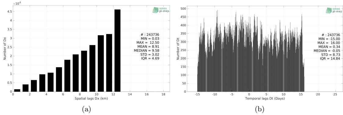
Figure 5: Histograms of the spatial (a) and temporal (b) lags between the location/time of the Waveglider measurement and the date of the corresponding SMOS SSS L3 v335 - Monthly - 25 km (CATDS-CPDC) SSS pixel.
