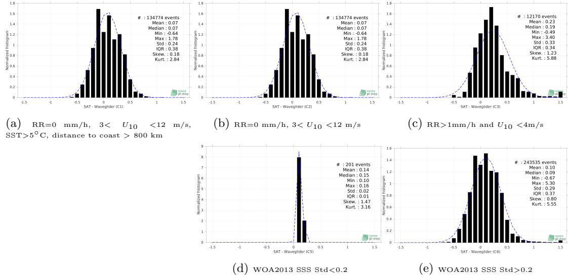
Figure 13: Normalized histogram of \Delta SSS (SMOS SSS L3 v335 - Monthly - 25 km (CATDS-CPDC) - Waveglider) for 5 different subdatasets corresponding to: RR=0 mm/h, 3 < U_{10} < 12 m/s, SST>5°C, distance to coast > 800 km (a), RR=0 mm/h, 3 < U_{10} < 12 m/s (b), RR>1mm/h and U_{10} < 4 m/s (c), WOA2013 SSS Std<0.2 (d), WOA2013 SSS Std>0.2 (e).
