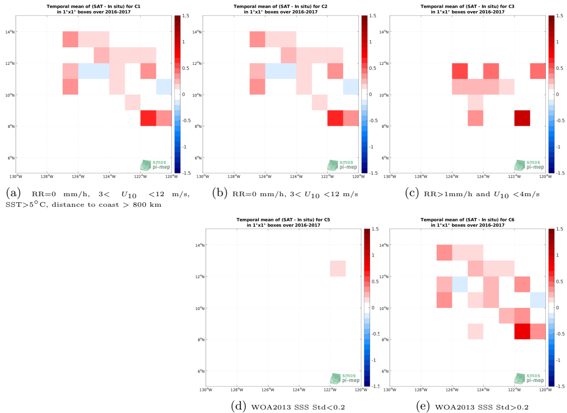
Figure 12: Temporal mean gridded over spatial boxes of size 1^\circ \times 1^\circ of \Delta SSS (SMOS SSS L3 v335 - Monthly - 25 km (CATDS-CPDC) - Waveglider) for 5 different subdatasets corresponding to:RR=0 mm/h, 3 < U_{10} < 12 m/s, SST >5^\circ\text{C} , distance to coast > 800 km (a), RR=0 mm/h, 3 < U_{10} < 12 m/s (b), RR >1 mm/h and U_{10} < 4 m/s (c), WOA2013 SSS Std <0.2 (d), WOA2013 SSS Std >0.2 (e).
