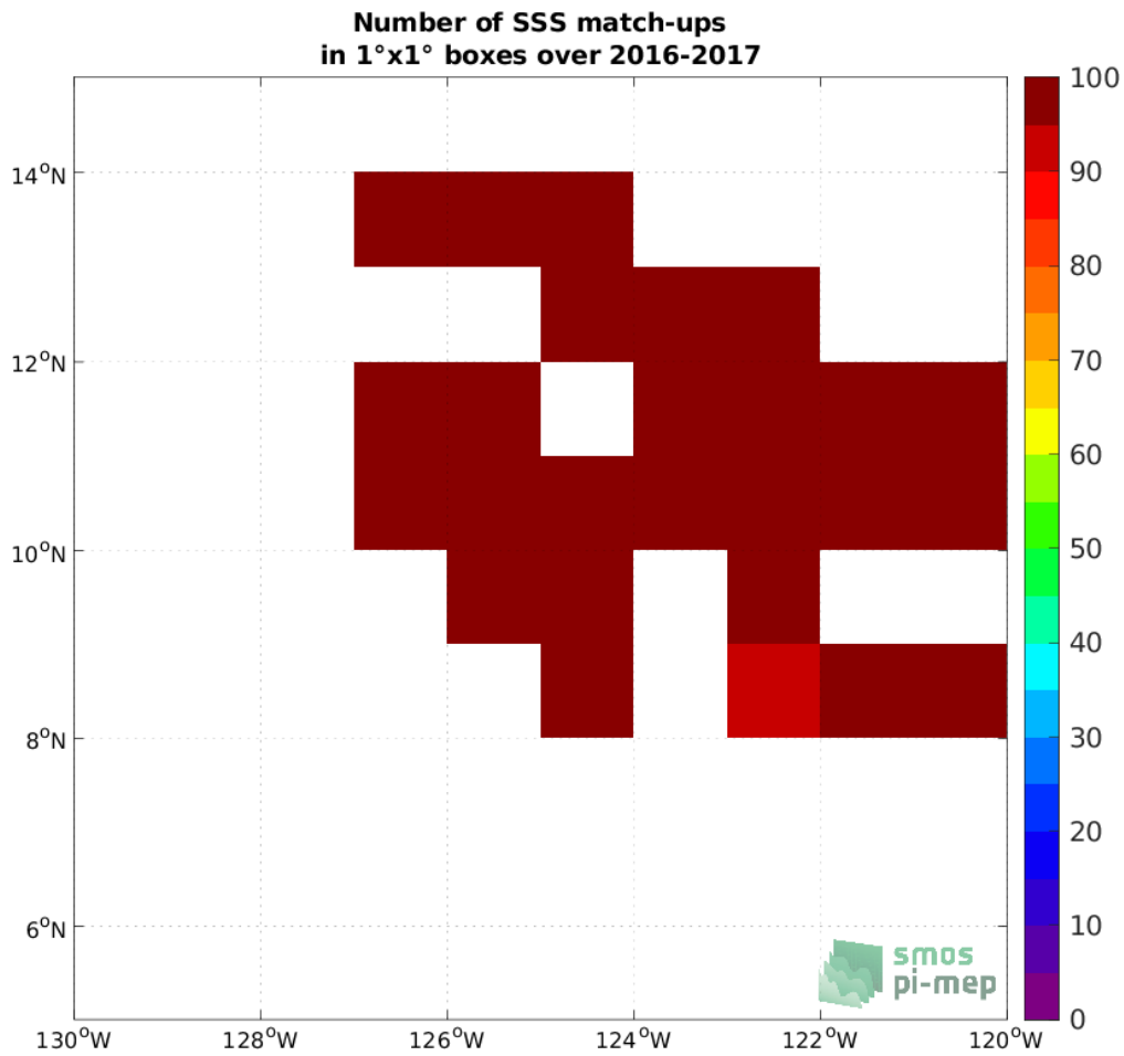
Figure 4: Number of SSS match-ups between Waveglider SSS and the SMOS SSS L3 v335 - Monthly - 25 km (CATDS-CPDC) SSS product for the SPURS 2 Pi-MEP region over 1°x1° boxes and for the full satellite product period.
