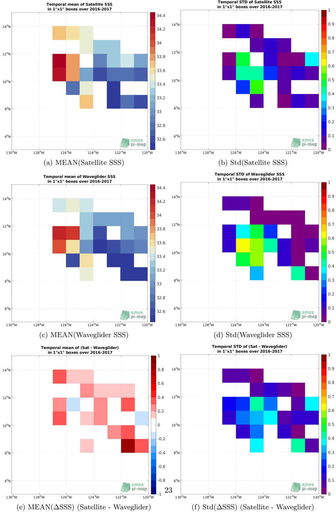
Figure 6: Temporal mean (left) and Std (right) of SSS from SMOS SSS L3 v335 - Monthly - 25 km (CATDS-CPDC) (top), Waveglider (middle), and of \Delta SSS (Satellite - Waveglider). Only match-up pairs are used to generate these maps.
