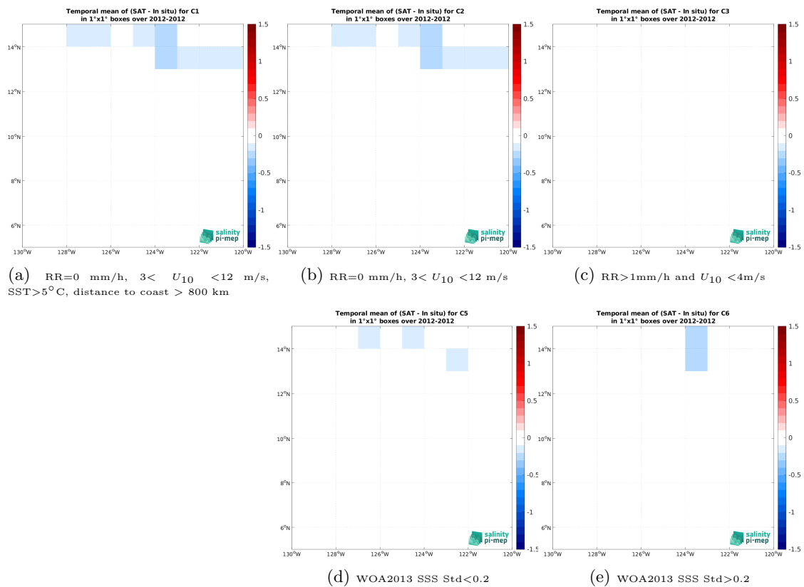
Figure 14: Temporal mean gridded over spatial boxes of size 1^\circ \times 1^\circ of \Delta\text{SSS} (SMOS SSS L3 v335 - Monthly - 25 km (CATDS-CPDC) - TSG (GOSUD-Research-vessel)) for 5 different subdatasets corresponding to: RR=0 mm/h, 3 < U_{10} < 12 m/s, SST > 5°C, distance to coast > 800 km (a), RR=0 mm/h, 3 < U_{10} < 12 m/s (b), RR > 1mm/h and U_{10} < 4 m/s (c), WOA2013 SSS Std < 0.2 (d), WOA2013 SSS Std > 0.2 (e).
