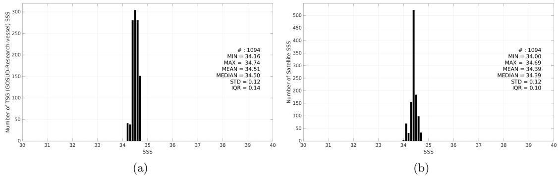
Figure 3: Histograms of SSS from TSG (GOSUD-Research-vessel) (a) and SMOS SSS L3 v335 - Monthly - 25 km (CATDS-CPDC) (b) considering all match-up pairs per bins of 0.1 over the SPURS 2 Pi-MEP region and for the full satellite product period.
