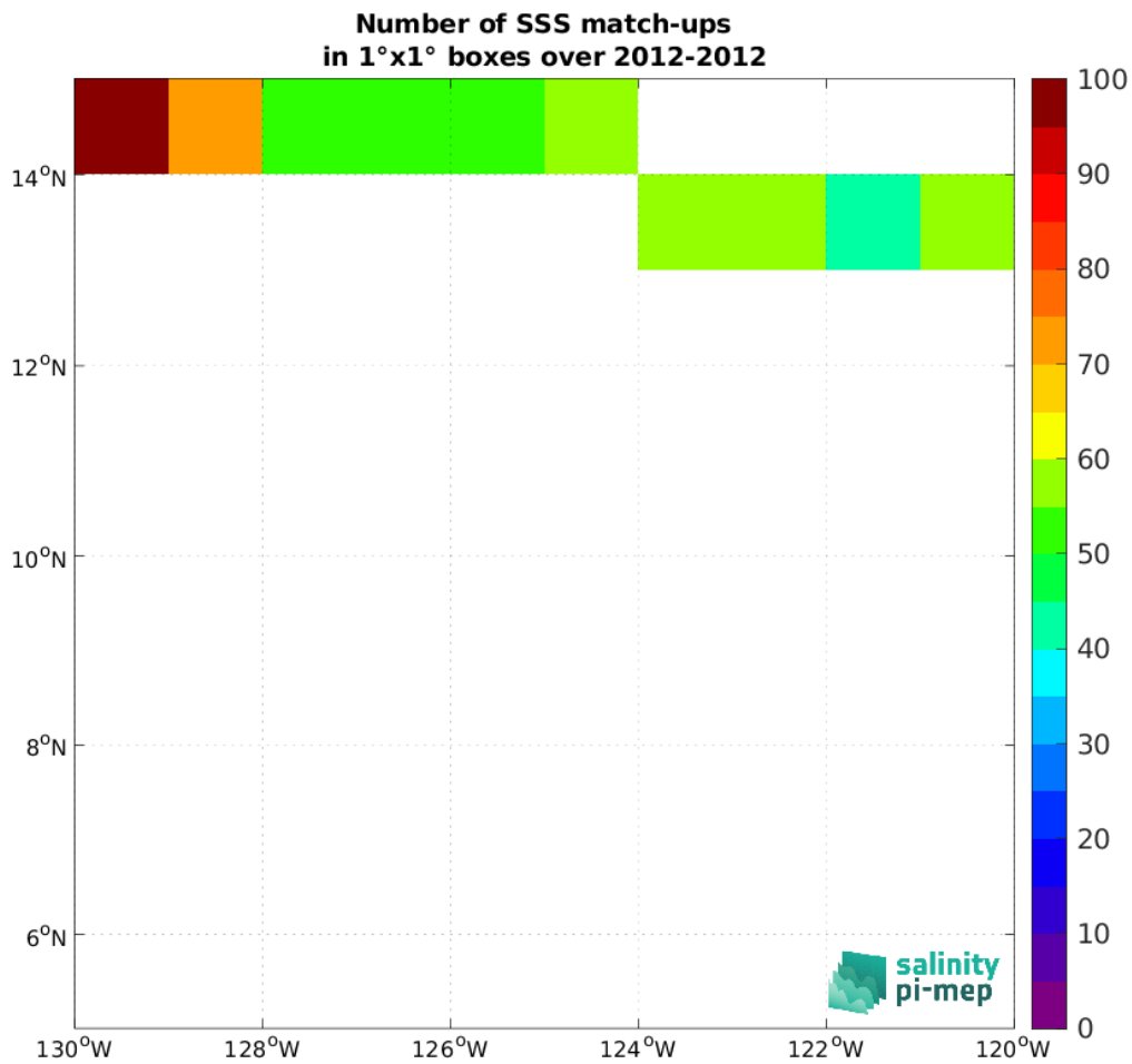
Figure 4: Number of SSS match-ups between TSG (GOSUD-Research-vessel) SSS and the SMOS SSS L3 v335 - Monthly - 25 km (CATDS-CPDC) SSS product for the SPURS 2 Pi-MEP region over 1^\circ \times 1^\circ boxes and for the full satellite product period.
