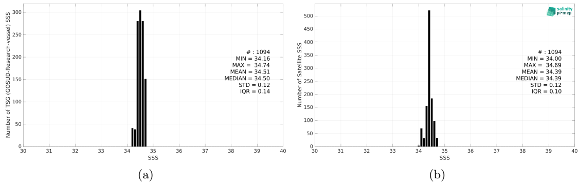
Figure 2: Histograms of SSS from TSG (GOSUD-Research-vessel) (a) and SMOS SSS L3 v335 - Monthly - 25 km (CATDS-CPDC) (b) considering all match-up pairs per bins of 0.1 over the SPURS 2 Pi-MEP region and for the full satellite product period.
